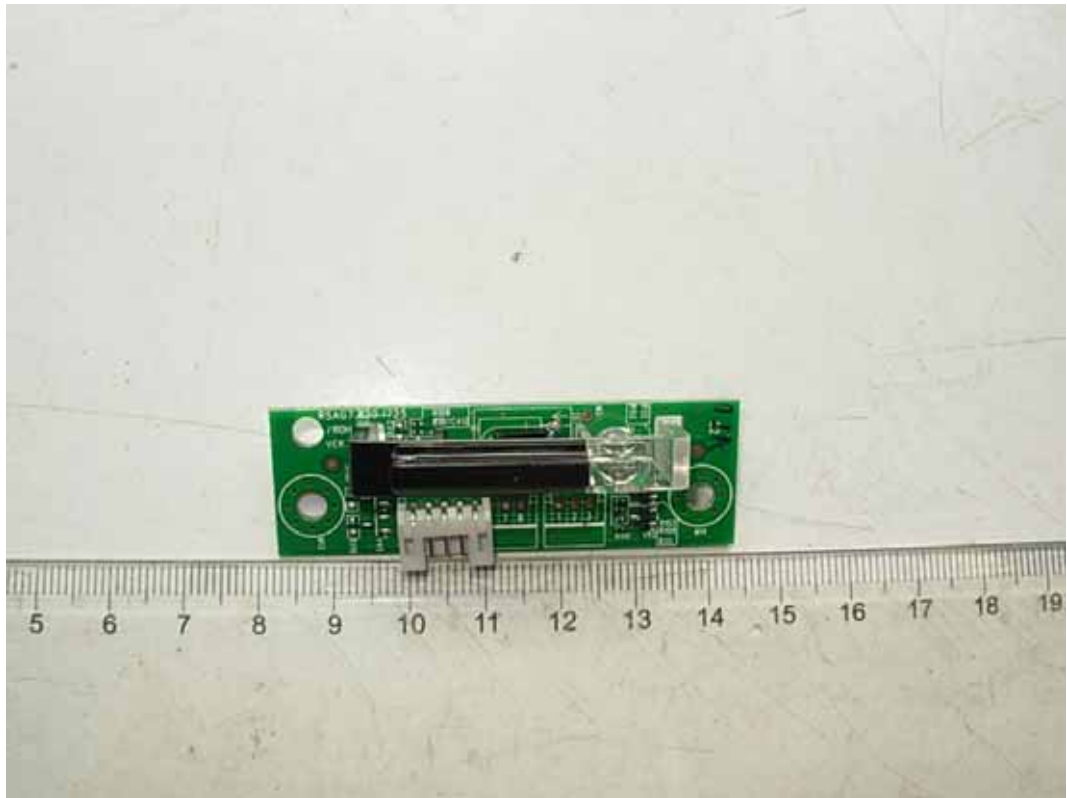
FIGURE 9 LCD TV (M/N: LTDN46V86US) IR BOARD (COMPONENT SIDE)
