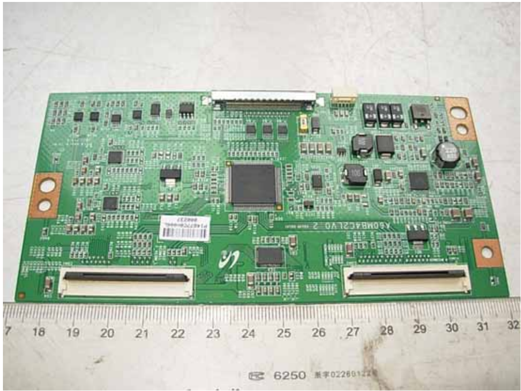
FIGURE 13 LCD TV (M/N: LTDN46V86US) DISPLAY BOARD (COMPONENT SIDE)
