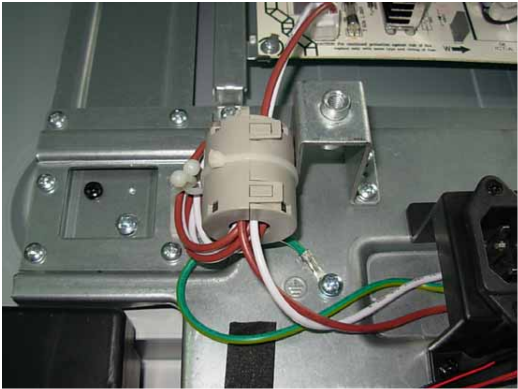
FIGURE 17 LCD TV (M/N: LTDN46V86US) DEBUG 1
