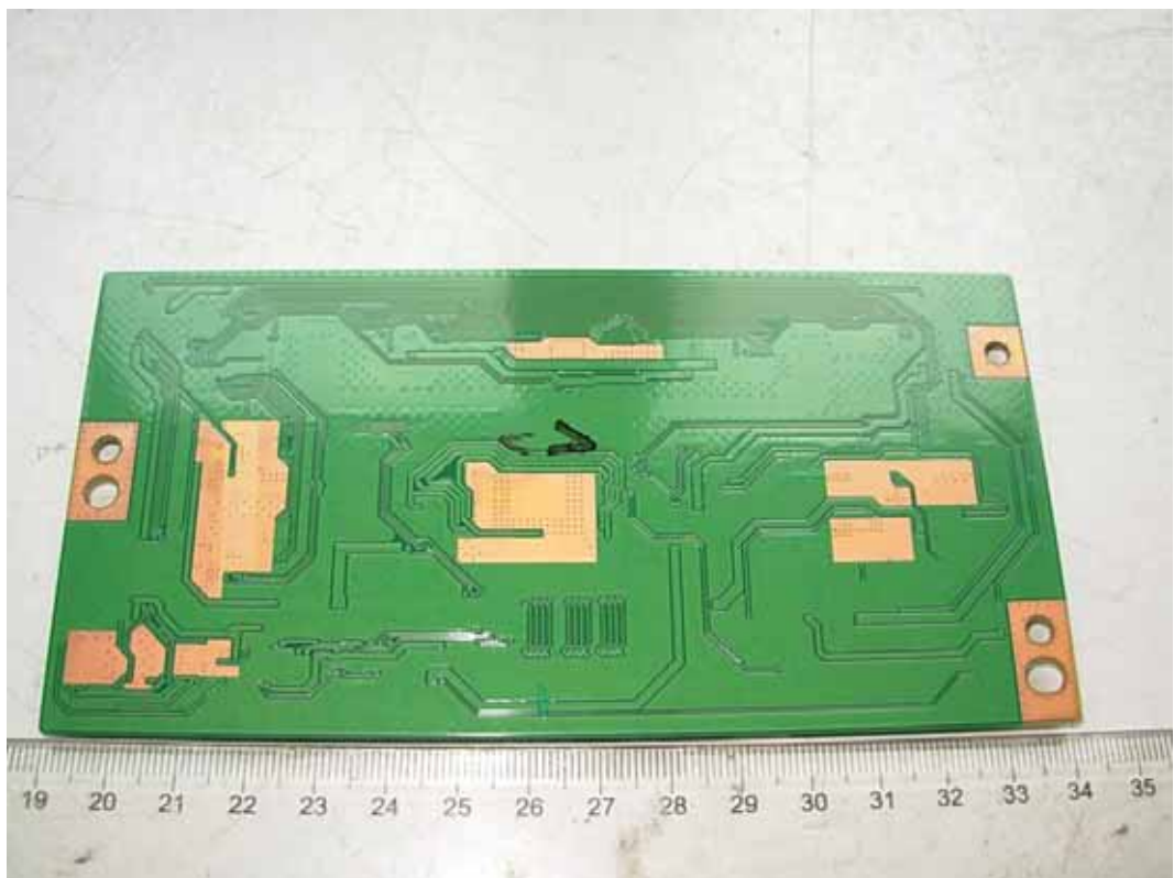
FIGURE 14 LCD TV (M/N: LTDN46V86US) DISPLAY BOARD (SOLDERED SIDE)
