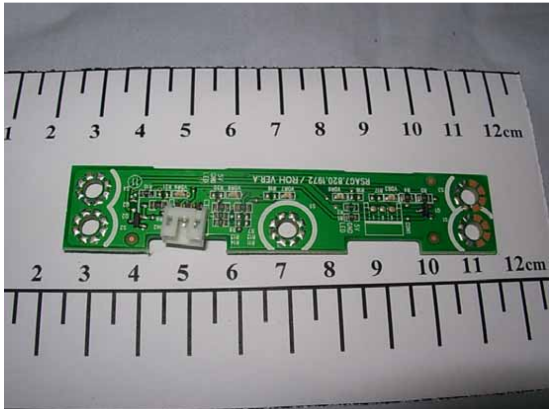
FIGURE 14 LCD TV (M/N: LTDN47T18GUS) LED BOARD (COMPONENT SIDE)
