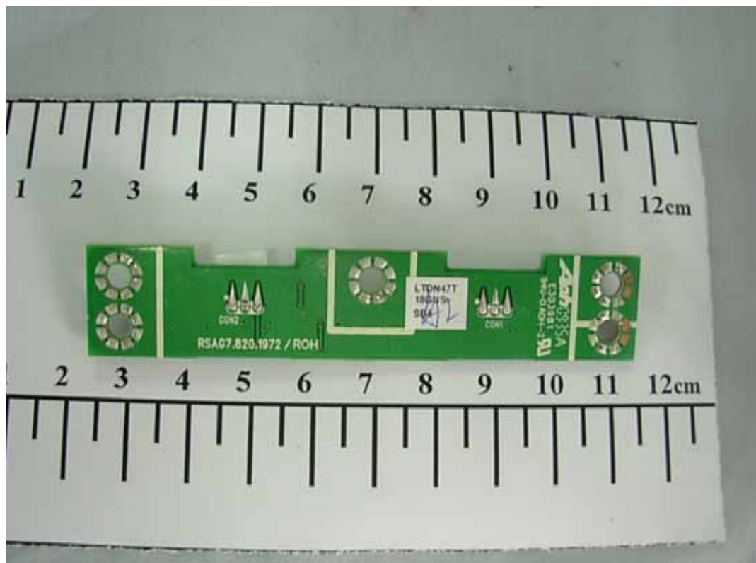
FIGURE 15 LCD TV (M/N: LTDN47T18GUS) LED BOARD (SOLDERED SIDE)
