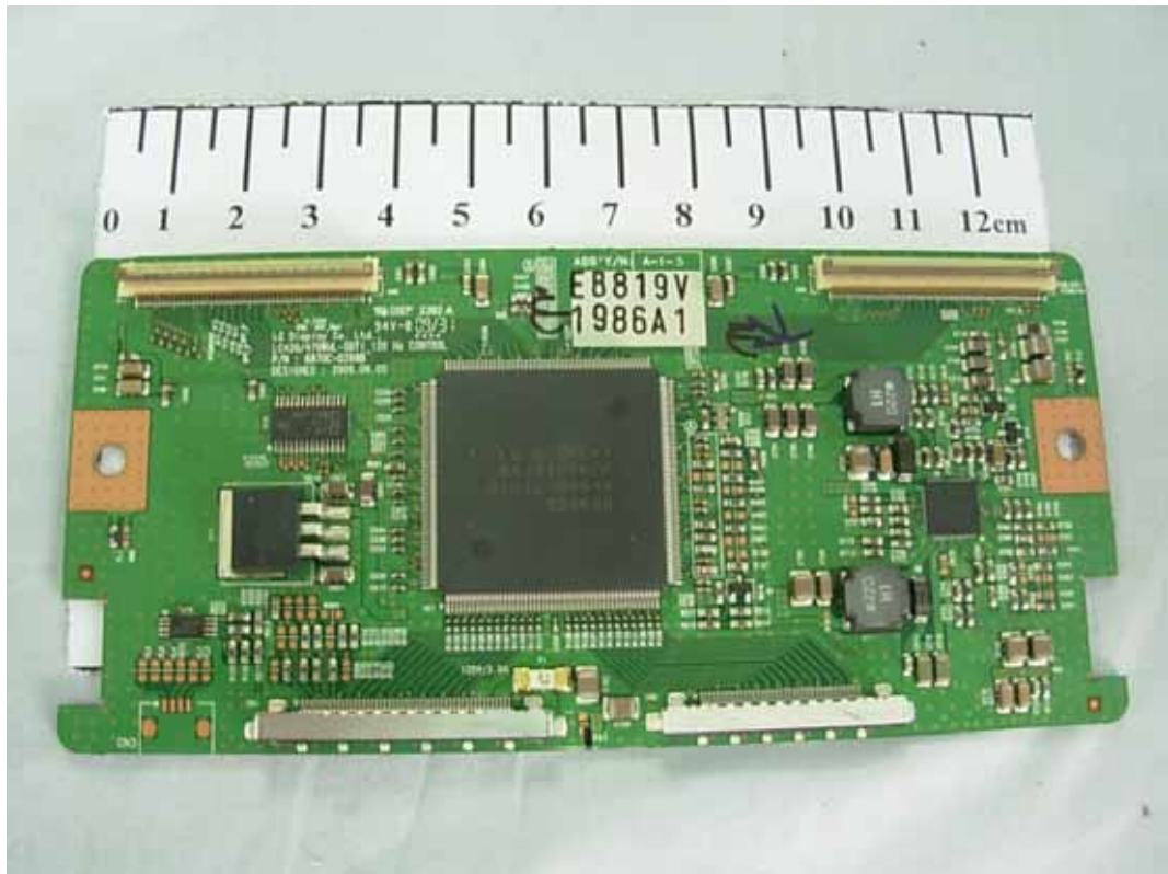
FIGURE 16 LCD TV (M/N: LTDN47T18GUS) DISPLAY BOARD (COMPONENT SIDE)
