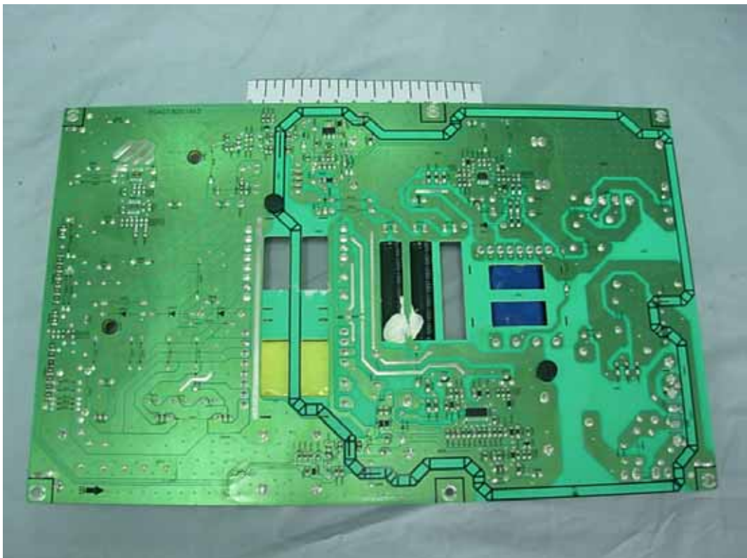
FIGURE 8 LCD TV (M/N: LTDN47T18GUS) POWER BOARD (SOLDERED SIDE)
