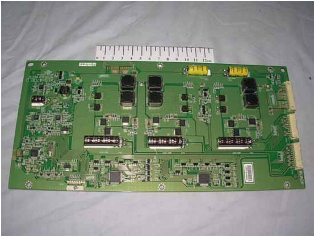
FIGURE 9 LCD TV (M/N: LTDN47T18GUS) INVERTER BOARD (COMPONENT SIDE)
