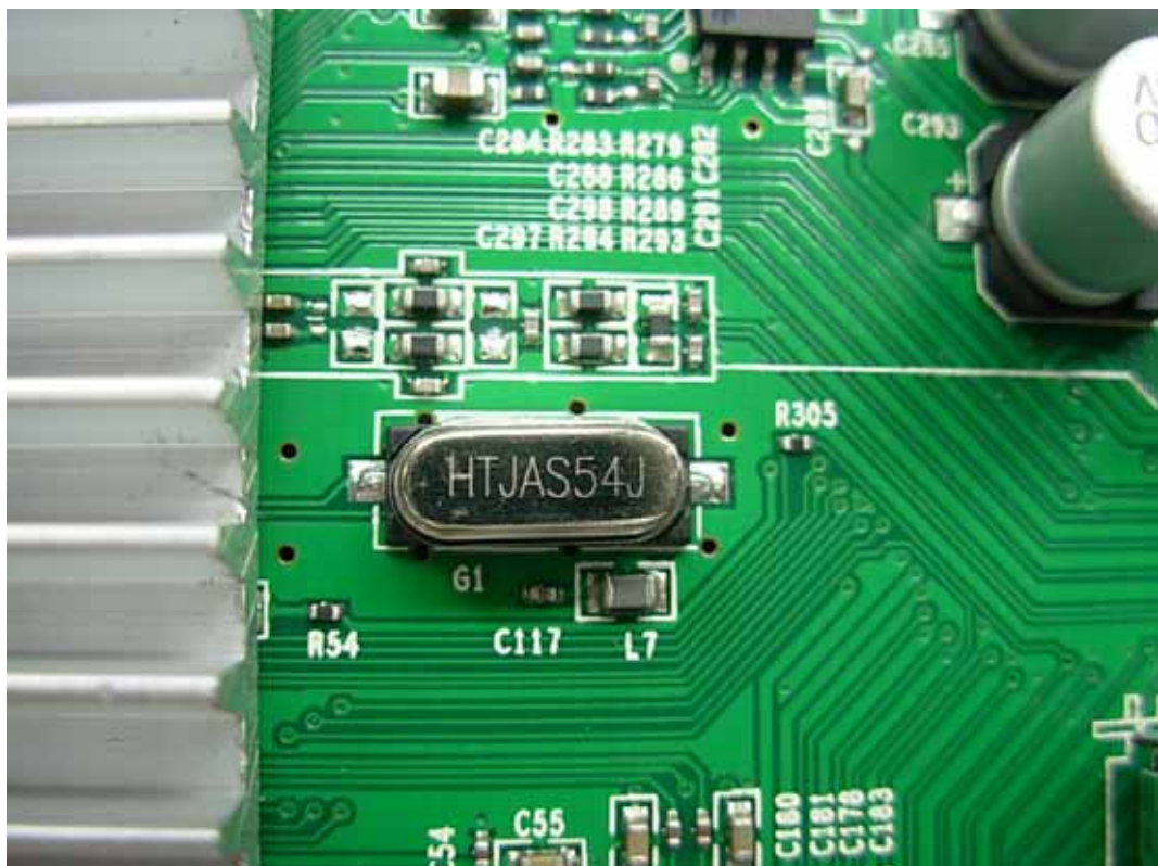
FIGURE 5 LCD TV (M/N: LTDN47T18GUS) CRYSTAL 1 ON MAIN BOARD
