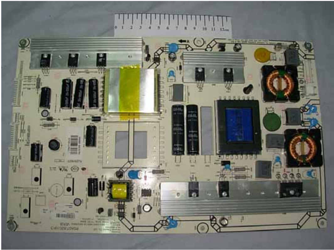
FIGURE 7 LCD TV (M/N: LTDN47T18GUS) POWER BOARD (COMPONENT SIDE)
