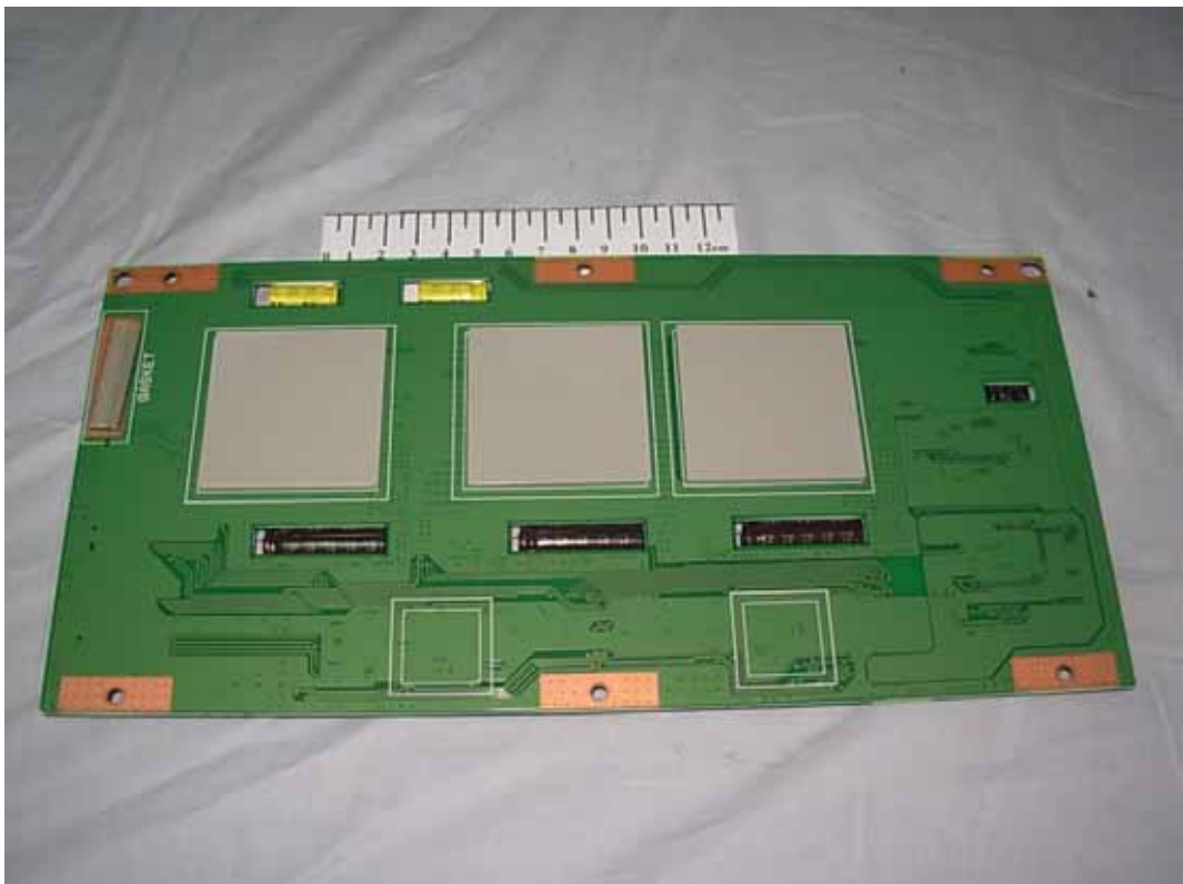
FIGURE 10 LCD TV (M/N: LTDN47T18GUS) INVERTER BOARD (SOLDERED SIDE)
