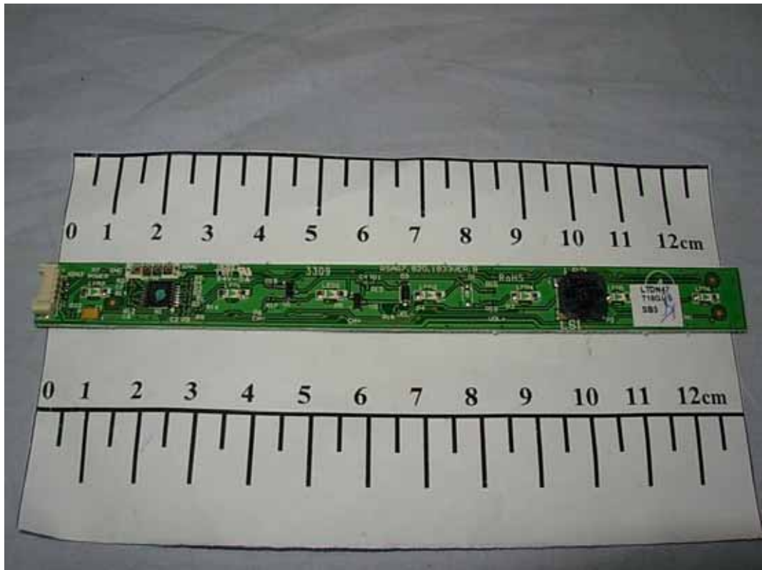
FIGURE 12 LCD TV (M/N: LTDN47T18GUS) BUTTON BOARD (COMPONENT SIDE)
