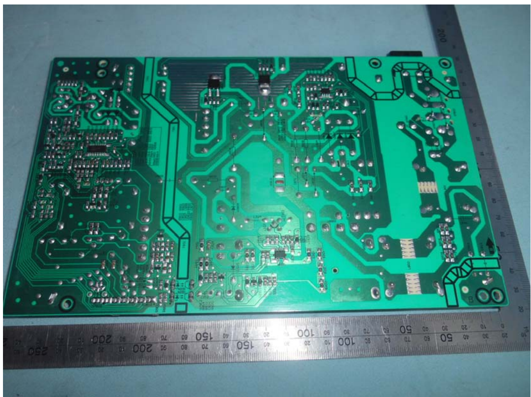
FIGURE 4 LED LCD TV (M/N: LC-43P7000U) POWER BOARD (SOLDERED SIDE)
