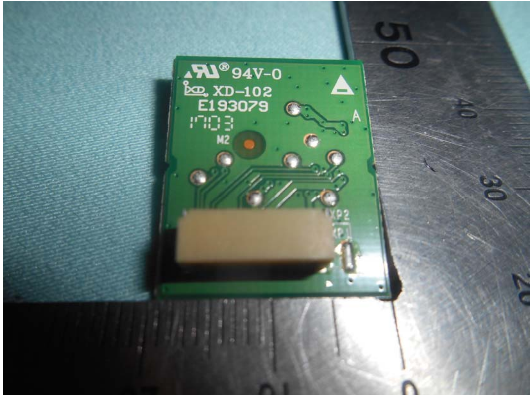
FIGURE 5 LED LCD TV (M/N: LC-43P7000U) IR BOARD (COMPONENT SIDE)
