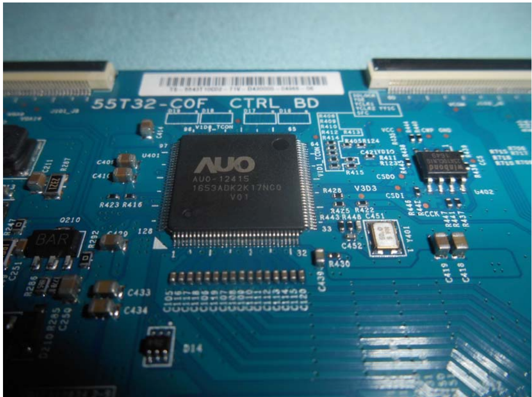
FIGURE 19 LED LCD TV (M/N: LC-43P7000U) CHIP AND CRYSTAL ON PANEL BOARD
