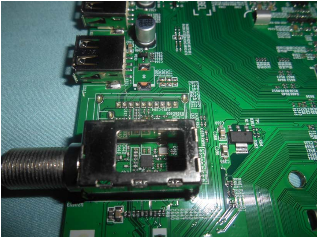
FIGURE 10 LED LCD TV (M/N: LC-43P7000U) TUNER
