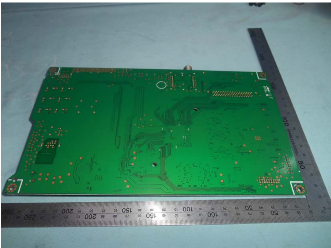
FIGURE 8 LED LCD TV (M/N: LC-43P7000U) MAIN BOARD (SOLDERED SIDE)
