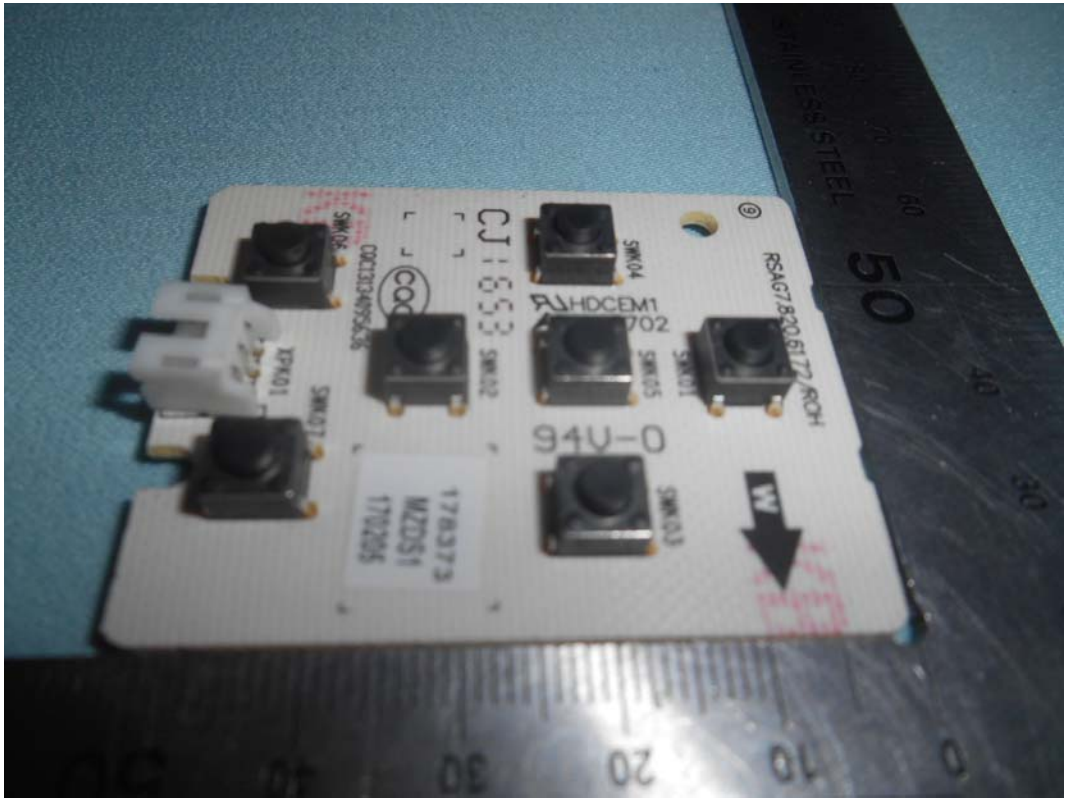
FIGURE 11 LED LCD TV (M/N: LC-43P7000U) KEY BOARD (COMPONENT SIDE)
