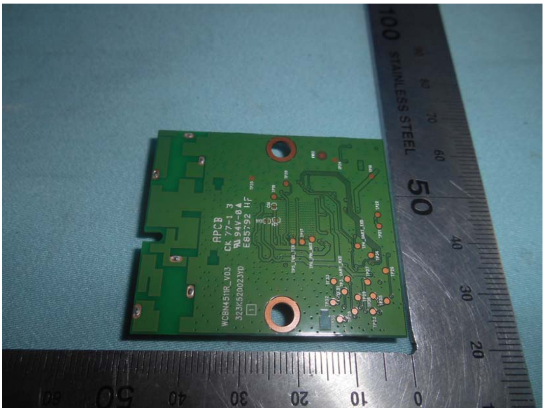
FIGURE 14 LED LCD TV (M/N: LC-43P7000U) RF BOARD (SOLDERED SIDE)
