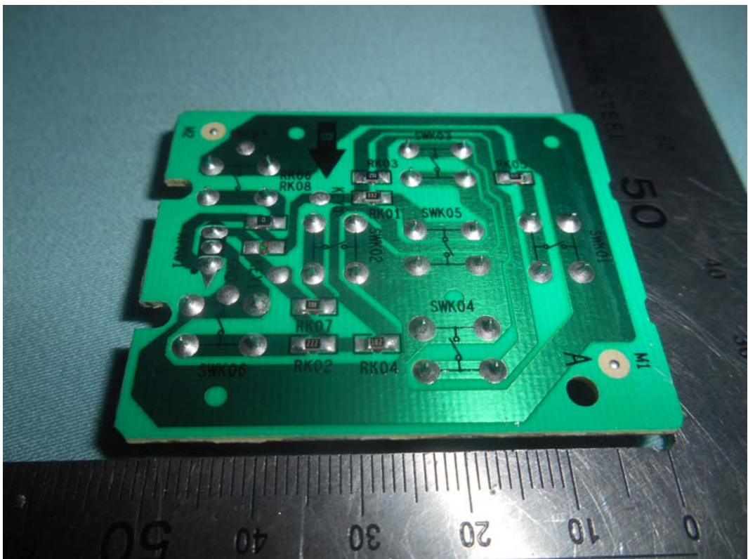
FIGURE 12 LED LCD TV (M/N: LC-43P7000U) KEY BOARD (SOLDERED SIDE)
