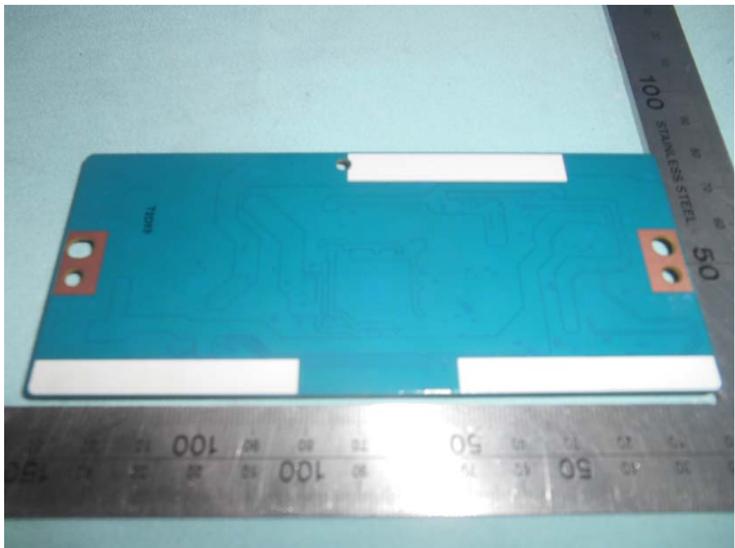
FIGURE 18 LED LCD TV (M/N: LC-43P7000U) PANEL BOARD (SOLDERED SIDE)
