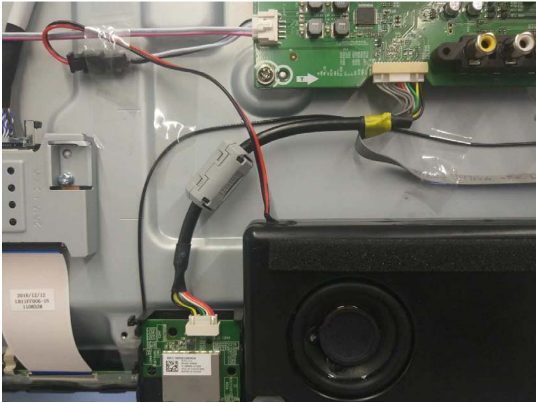
FIGURE 19 LED LCD TV (M/N: 43H4D) DEBUG
