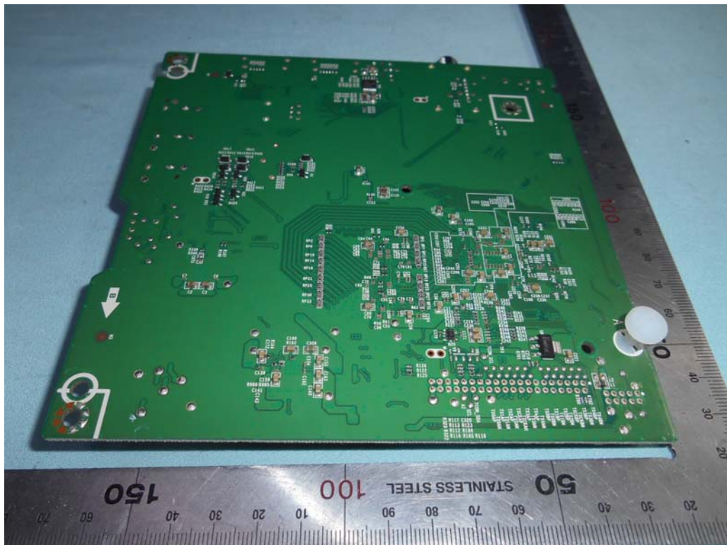
FIGURE 4 LED LCD TV (M/N: 43H4D) MAIN BOARD (SOLDERED SIDE)
