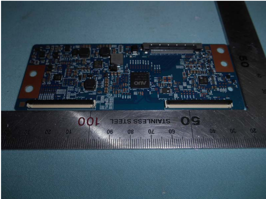
FIGURE 12 LED LCD TV (M/N: 43H4D) LCD PANEL BOARD (COMPONENT SIDE)
