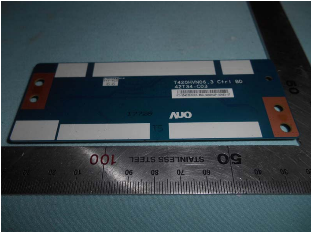
FIGURE 13 LED LCD TV (M/N: 43H4D) LCD PANEL BOARD (SOLDERED SIDE)
