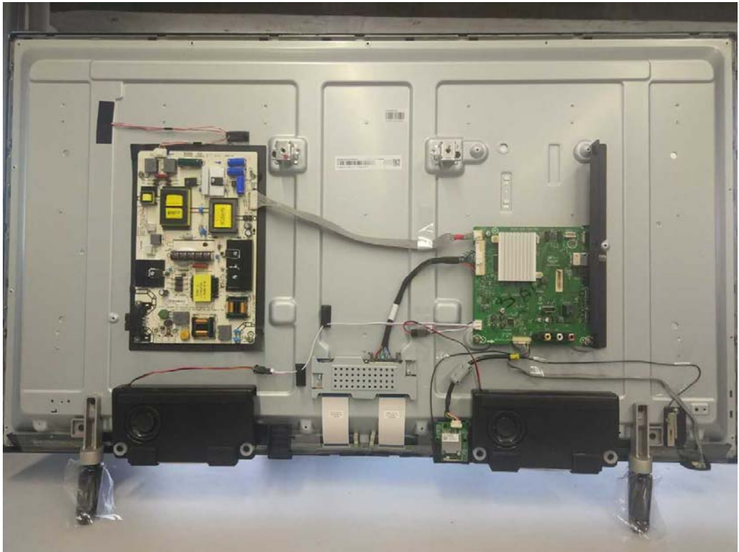
FIGURE 1 LED LCD TV (M/N: 43H4D) COVER REMOVED
