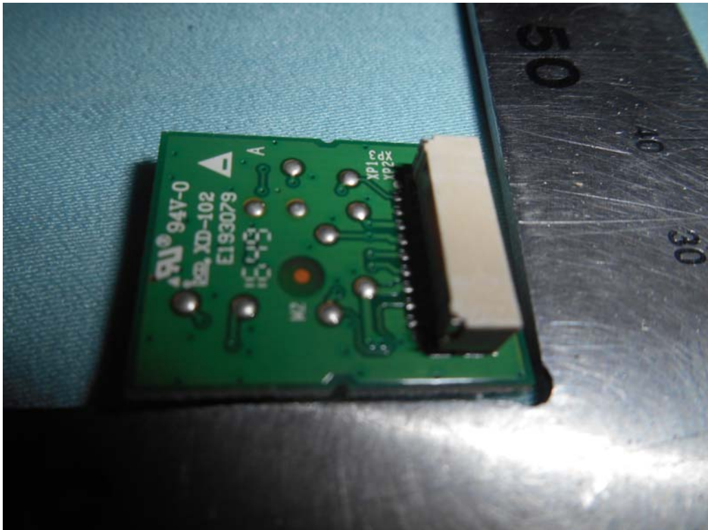
FIGURE 18 LED LCD TV (M/N: 43H4D) IR BOARD (SOLDERED SIDE)
