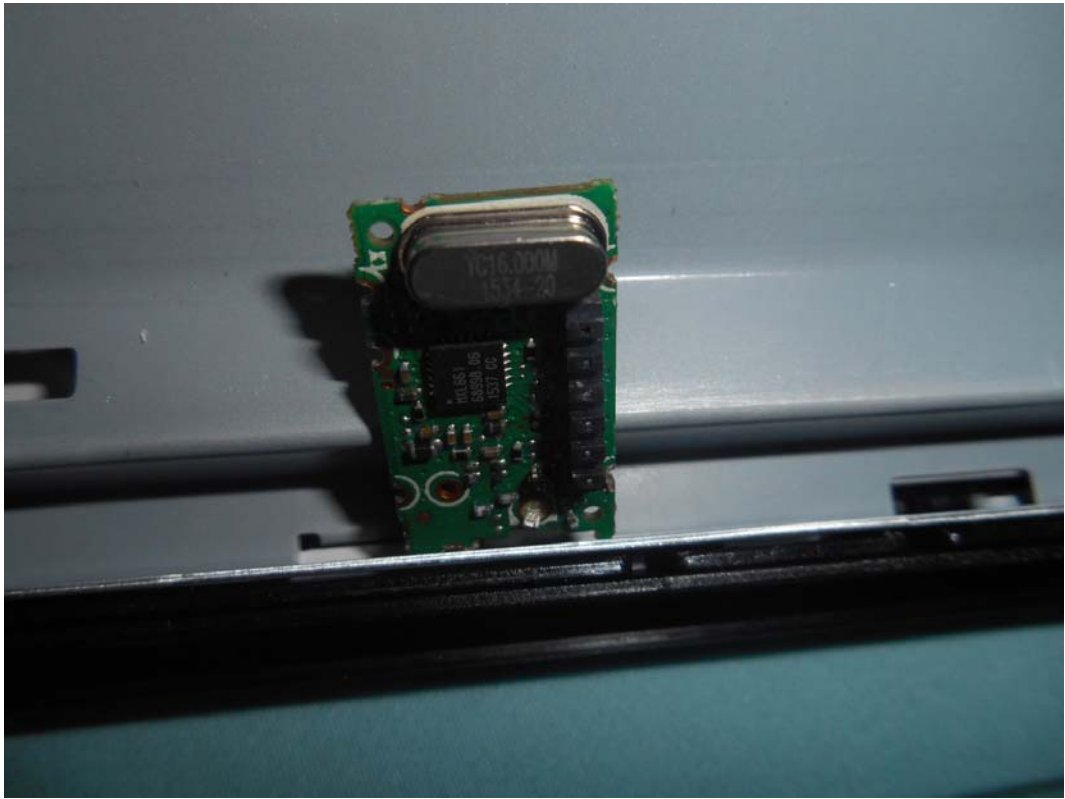
FIGURE 9 LED LCD TV (M/N: LC-43N6100U) TUNER CRYSTAL ON MAIN BOARD
