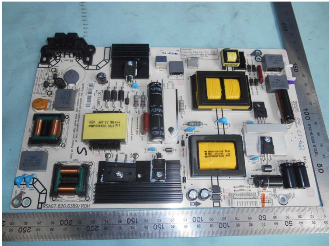
FIGURE 17 LED LCD TV (M/N: LC-43N6100U) POWER BOARD (COMPONENT SIDE)
