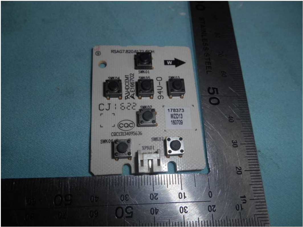
FIGURE 19 LED LCD TV (M/N: LC-43N6100U) KEY BOARD (COMPONENT SIDE)
