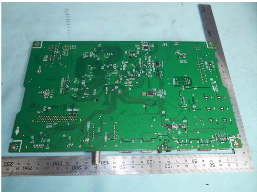
FIGURE 4 LED LCD TV (M/N: LC-43N6100U) MAIN BOARD (SOLDERED SIDE)
