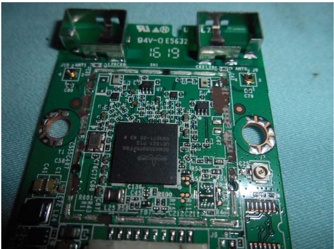
FIGURE 16 LED LCD TV (M/N: LC-43N6100U) RF BOARD COVER REMOVED
