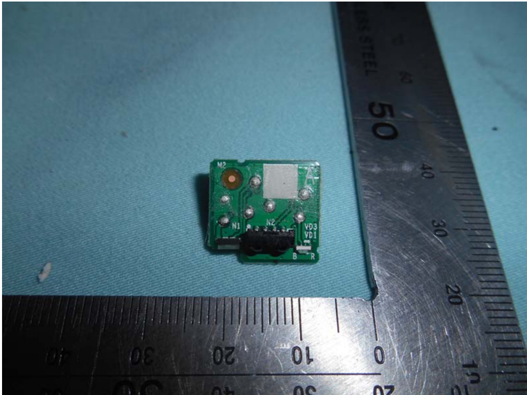
FIGURE 17 LED LCD TV (M/N: 43H7C) IR BOARD (COMPONENT SIDE)
