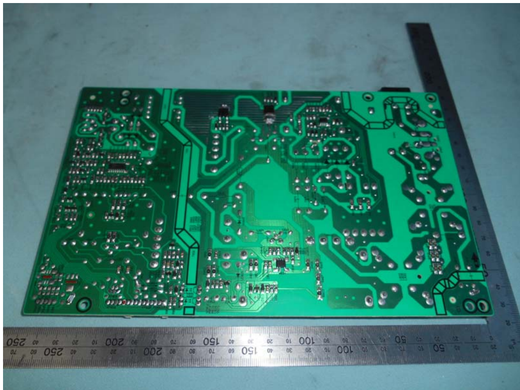
FIGURE 4 LED LCD TV (M/N: 43H7C) POWER BOARD (SOLDERED SIDE)
