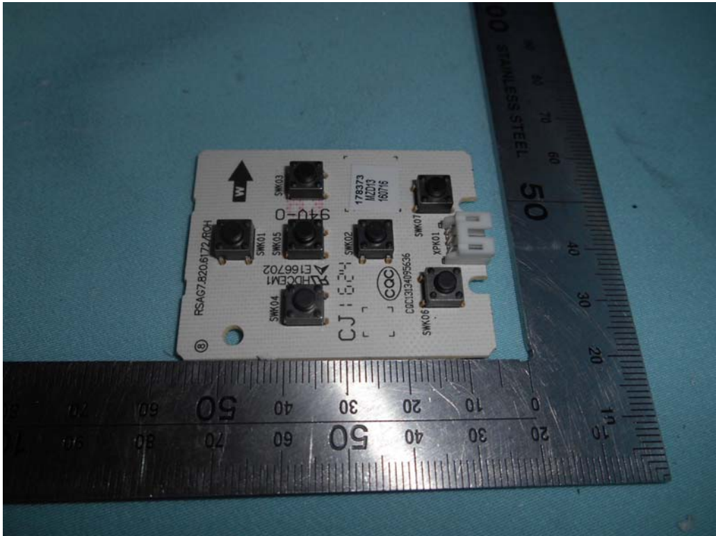
FIGURE 15 LED LCD TV (M/N: 43H7C) KEY BOARD (COMPONENT SIDE)
