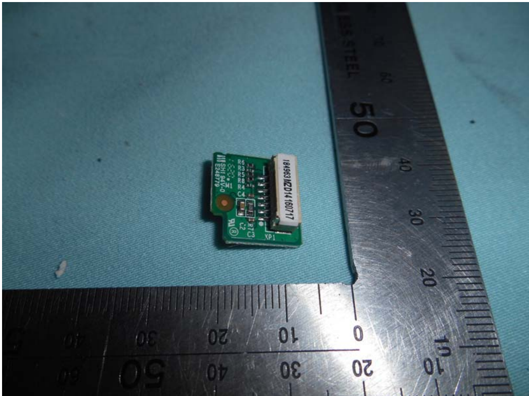
FIGURE 18 LED LCD TV (M/N: 43H7C) IR BOARD (SOLDERED SIDE)
