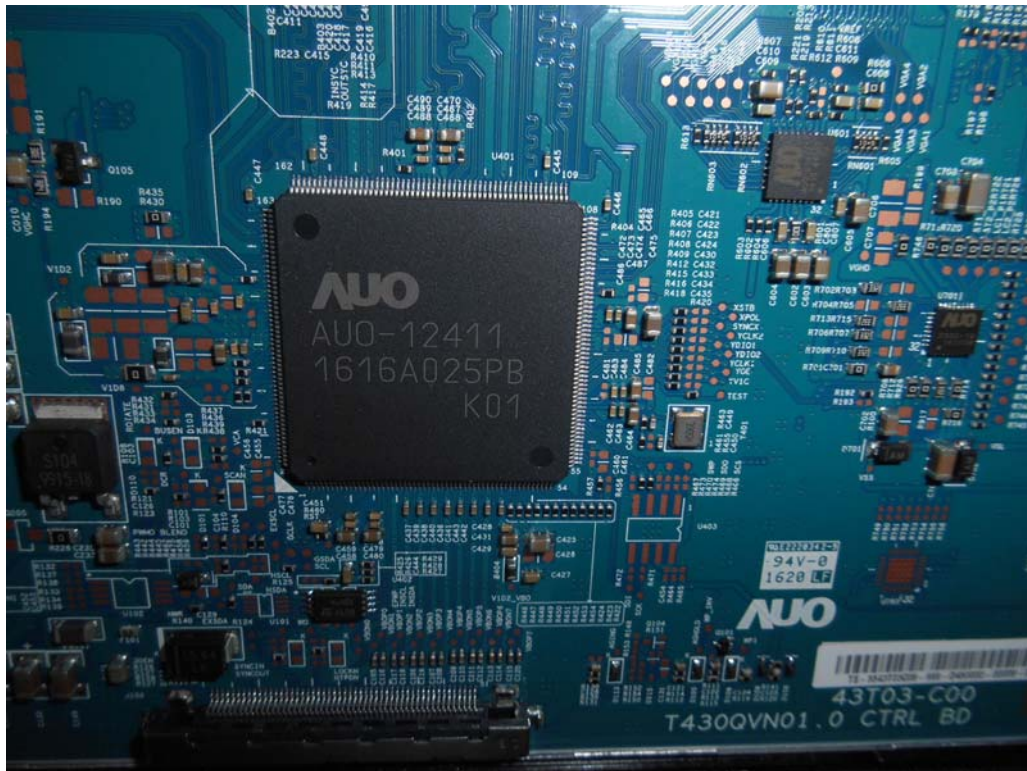
FIGURE 14 LED LCD TV (M/N: 43H7C) CHIP AND CRYSTAL ON PANEL BOARD
