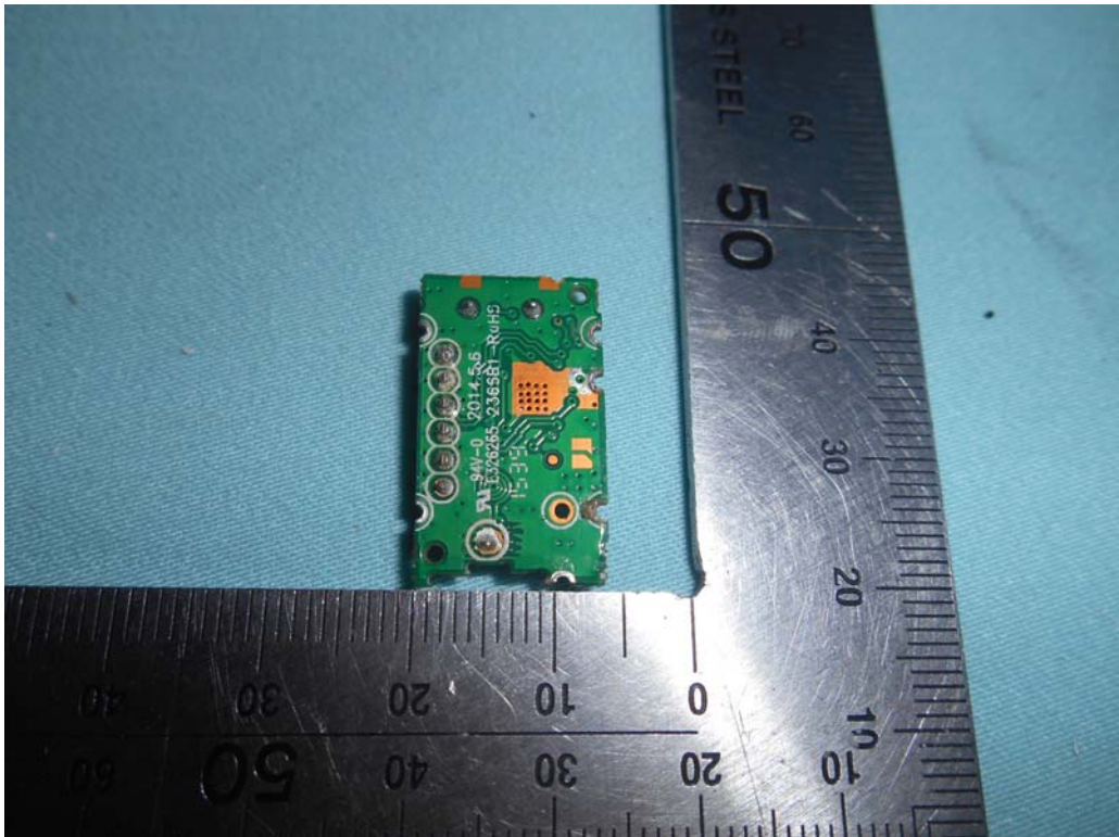
FIGURE 10 LED LCD TV (M/N: 43H7C) MAIN BOARD (SOLDERED SIDE)
