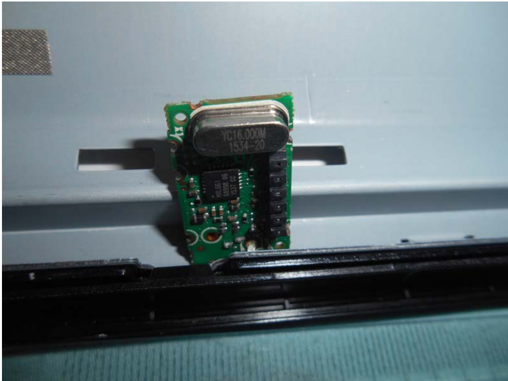
FIGURE 11 LED LCD TV (M/N: 43H7C) CRYSTAL ON TUNER BOARD
