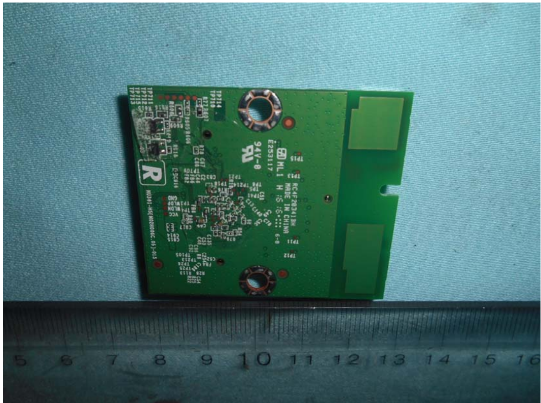
FIGURE 14 LED LCD TV (M/N: LC-43N7000U) RF BOARD (SOLDERED SIDE)
