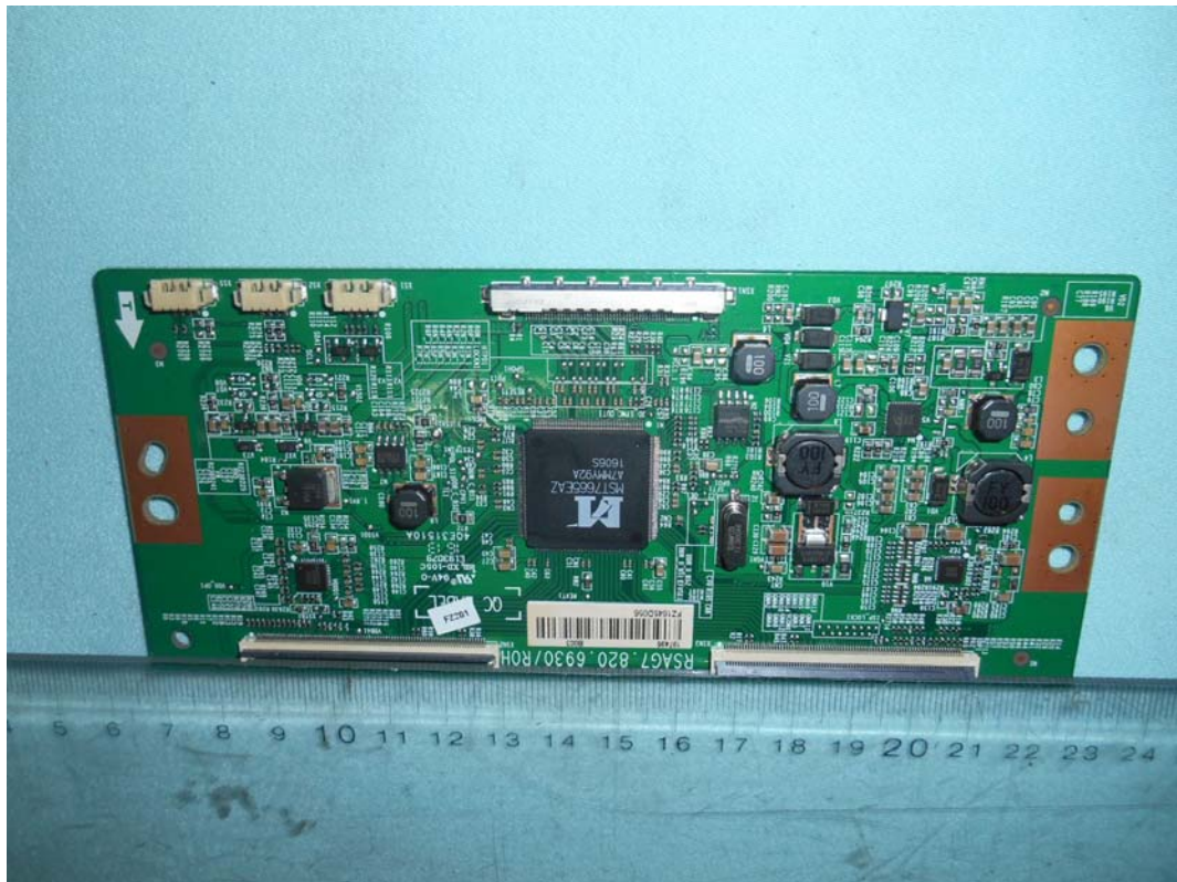
FIGURE 10 LED LCD TV (M/N: LC-43N7000U) PANEL BOARD (COMPONENT SIDE)
