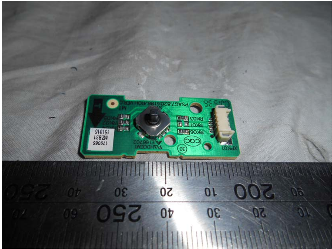
FIGURE 19 LED LCD TV (M/N: LC-43N7000U) KEY BOARD (COMPONENT SIDE)
