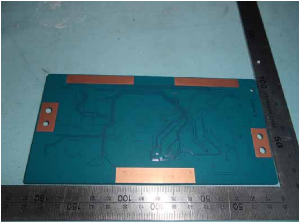
FIGURE 12 LED LCD TV (M/N: RLED4350-UHD-B-SM) PANEL BOARD (SOLDERED SIDE)
