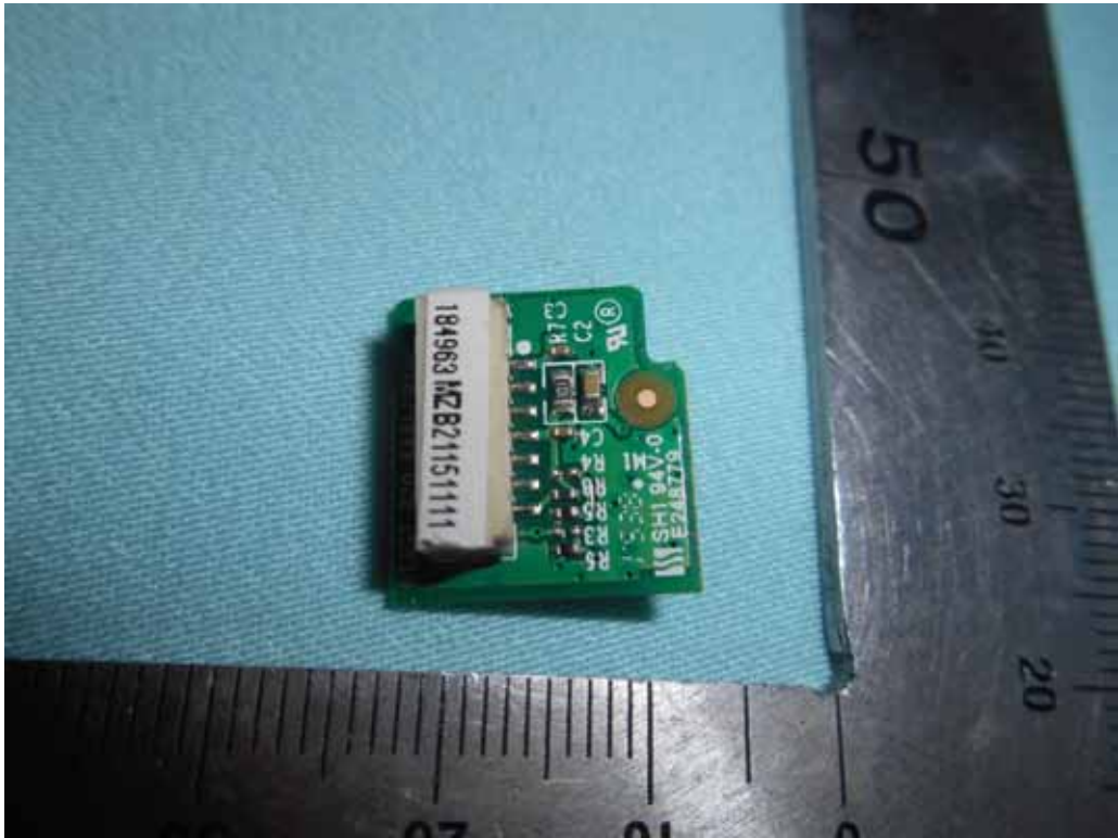
FIGURE 21 LED LCD TV (M/N: RLED4350-UHD-B-SM) IR BOARD (SOLDERED SIDE)
