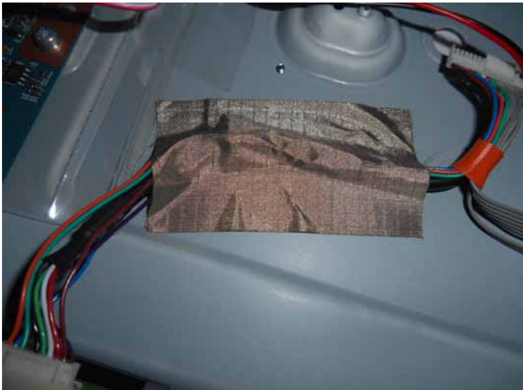
FIGURE 22 LED LCD TV (M/N: RLED4350-UHD-B-SM) DEBUG #1
