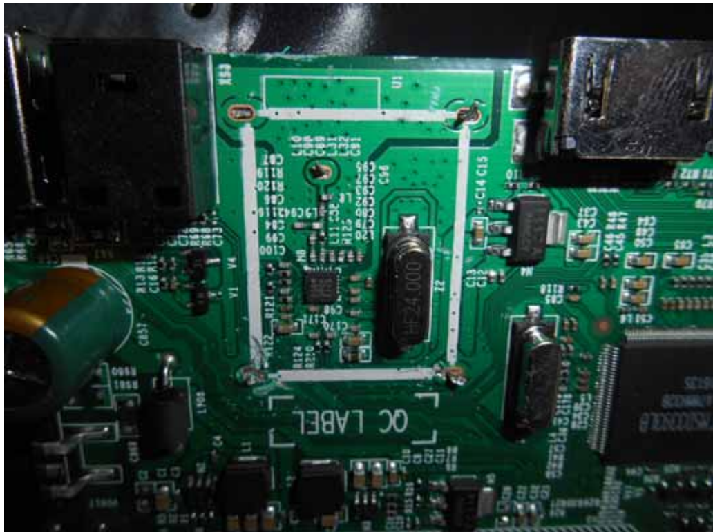
FIGURE 5 LED LCD TV (M/N: LC-40N3000U) TUNER & CRYSTAL ON MAIN BOARD
