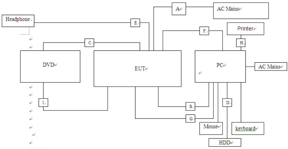
System Diagram of Connections between EUT and Simulators
