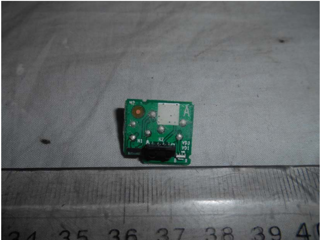
FIGURE 21 LED LCD TV (M/N: LC-43N6100U) IR BOARD (COMPONENT SIDE)
