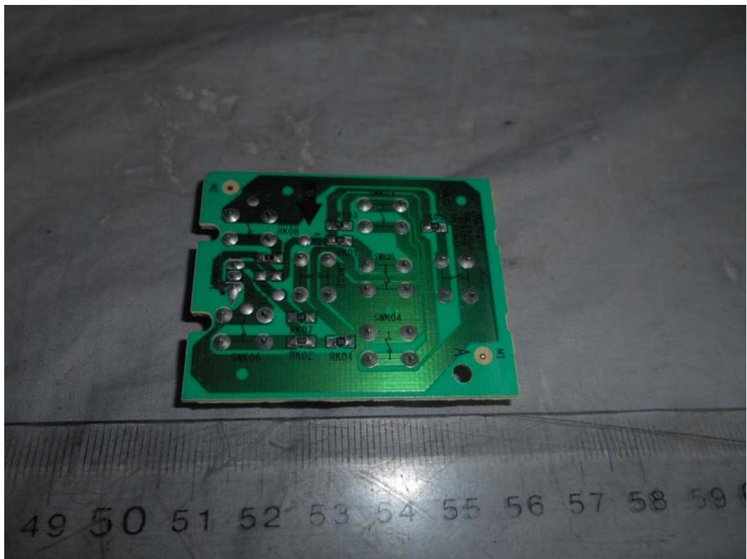
FIGURE 20 LED LCD TV (M/N: LC-43N6100U) KEY BOARD (SOLDERED SIDE)
