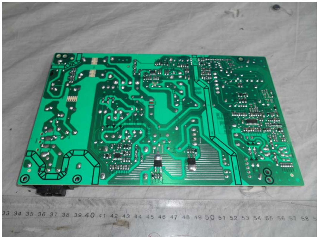
FIGURE 18 LED LCD TV (M/N: LC-43N6100U) POWER BOARD (SOLDERED SIDE)
