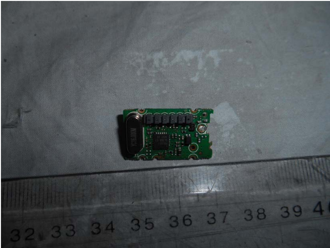
FIGURE 7 LED LCD TV (M/N: LC-40N5000U) TUNER BOARD (COMPONENT SIDE)
