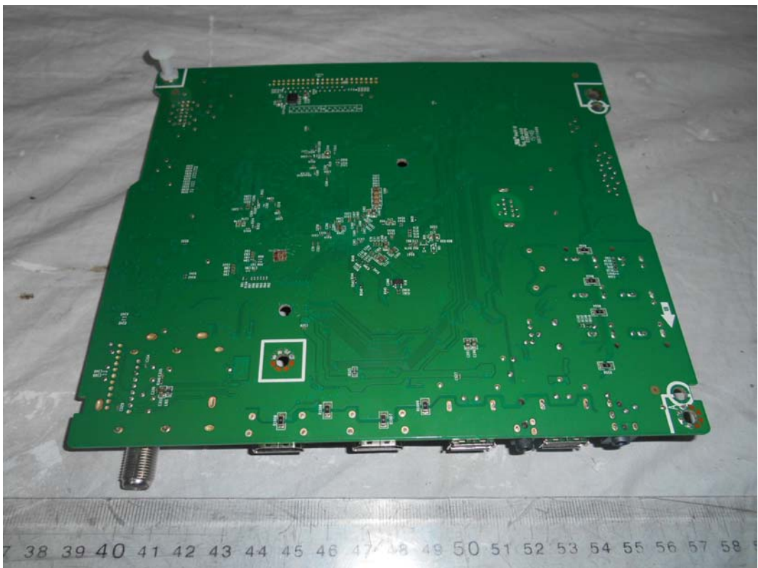
FIGURE 4 LED LCD TV (M/N: LC-40N5000U) MAIN BOARD (SOLDERED SIDE)
