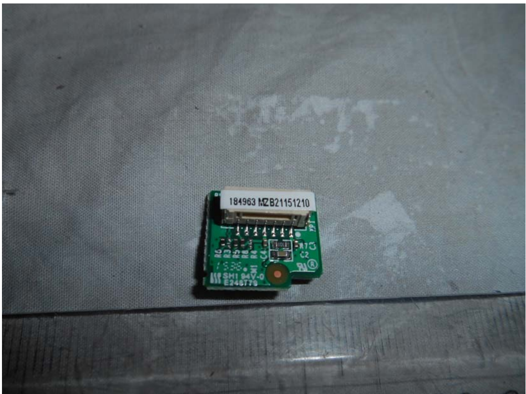
FIGURE 19 LED LCD TV (M/N: LC-40N5000U) IR BOARD (SOLDERED SIDE)
