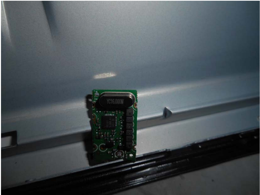
FIGURE 9 LED LCD TV (M/N: LC-40N5000U) TUNER CRYSTAL ON MAIN BOARD
