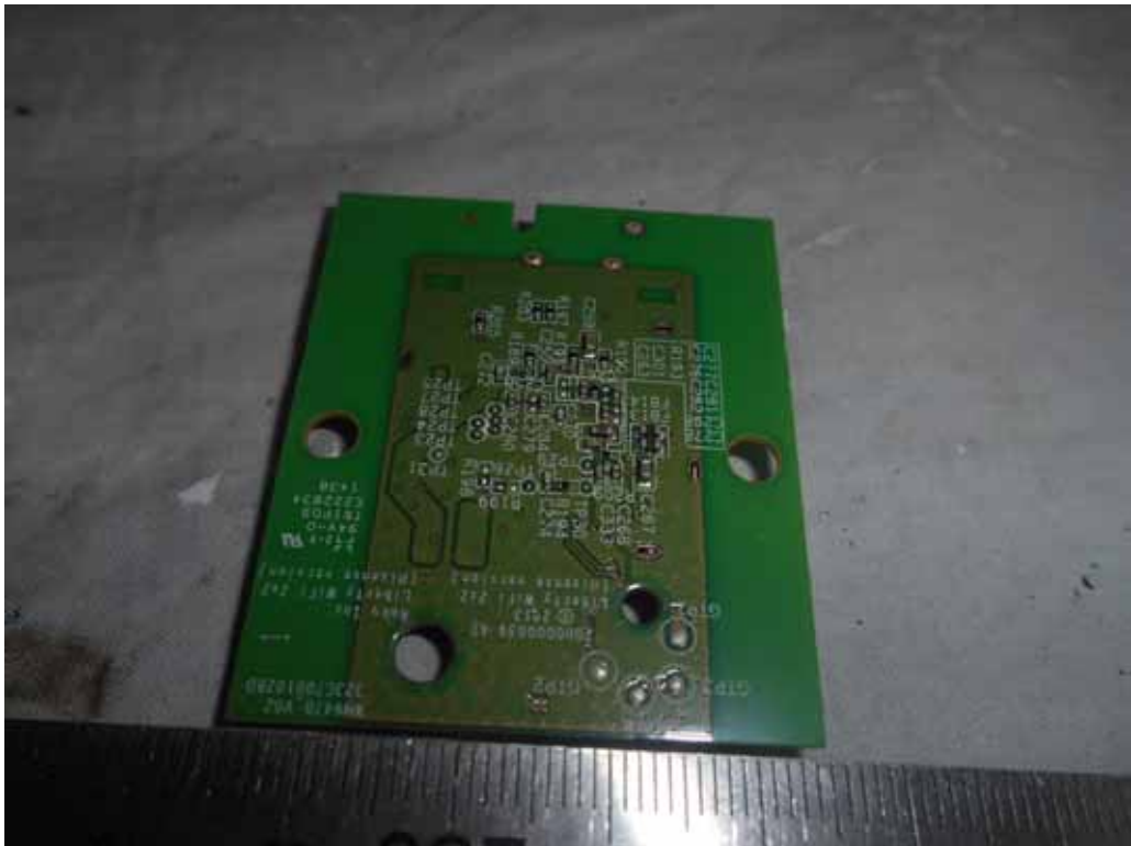
FIGURE 16 LED LCD TV (M/N: LC-43N4000U) RF BOARD (SOLDERED SIDE)
