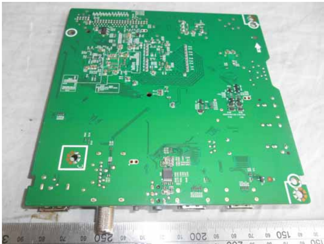
FIGURE 6 LED LCD TV (M/N: LC-43N4000U) MAIN BOARD (SOLDERED SIDE)
