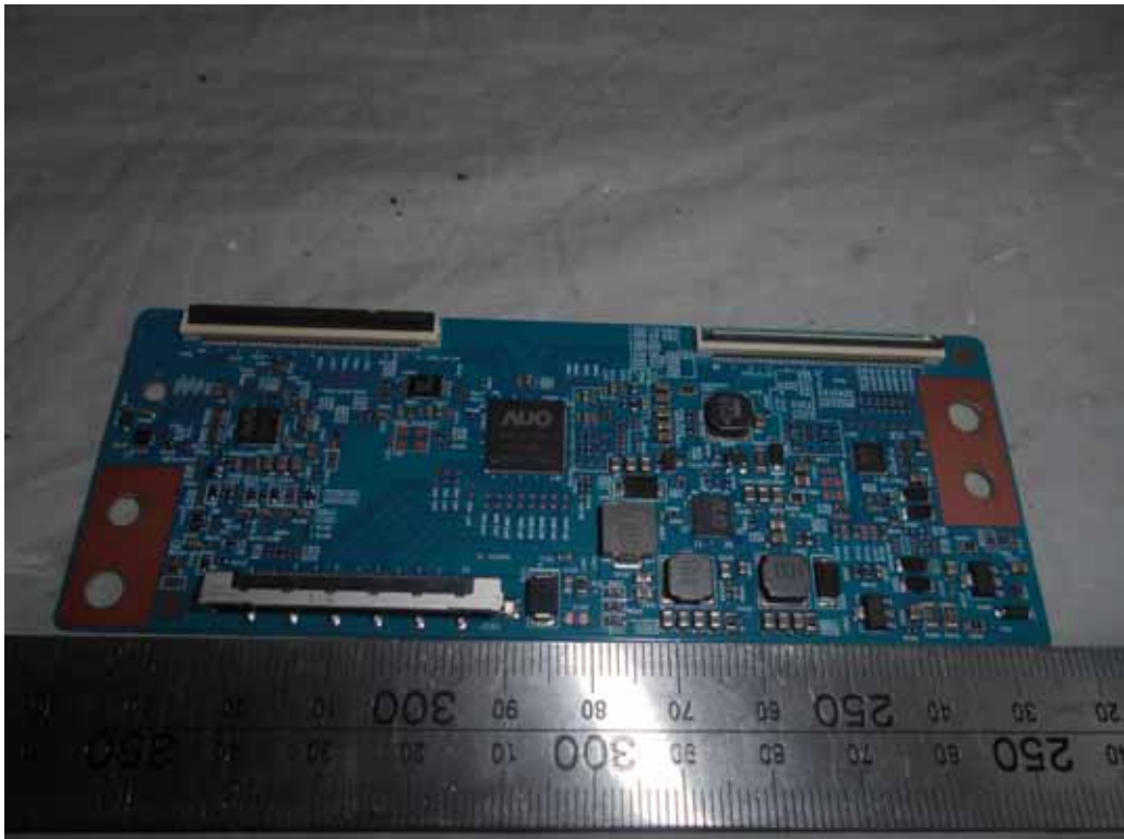
FIGURE 12 LED LCD TV (M/N: LC-43N4000U) PANEL BOARD (COMPONENT SIDE)
