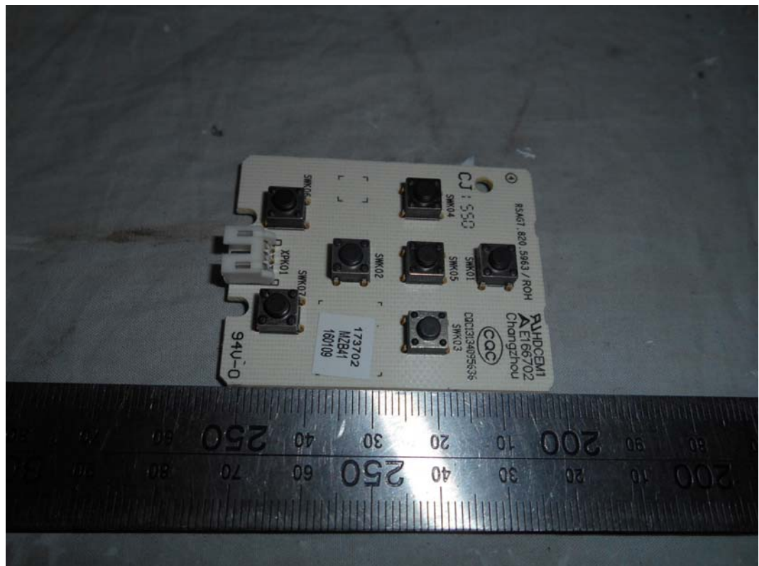
FIGURE 12 LED LCD TV (M/N: 40H5B) KEY BOARD (COMPONENT SIDE)
