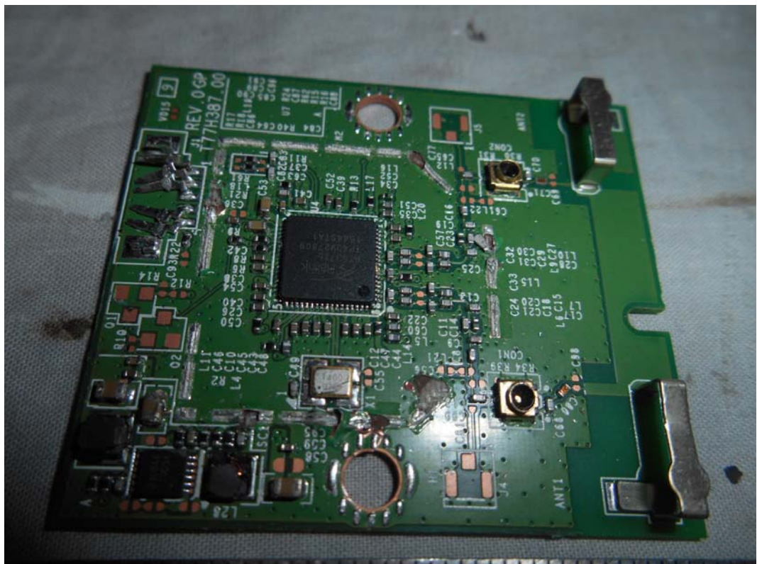
FIGURE 11 LED LCD TV (M/N: 40H5B) RF BOARD COVER REMOVED
