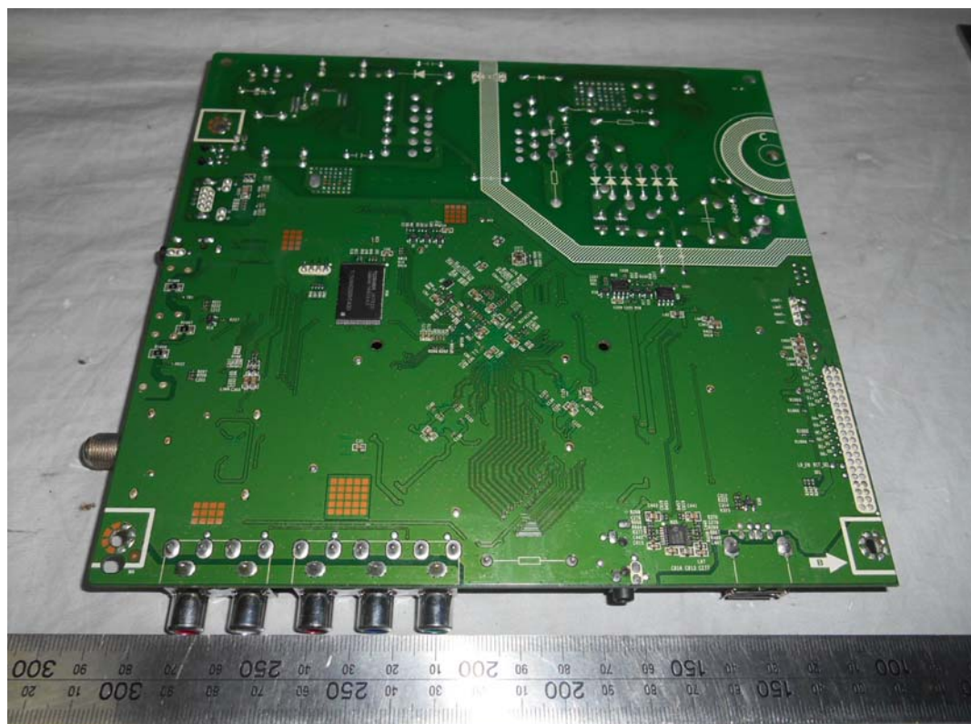
FIGURE 4 LED LCD TV (M/N: 40H5B) MAIN BOARD (SOLDERED SIDE)
