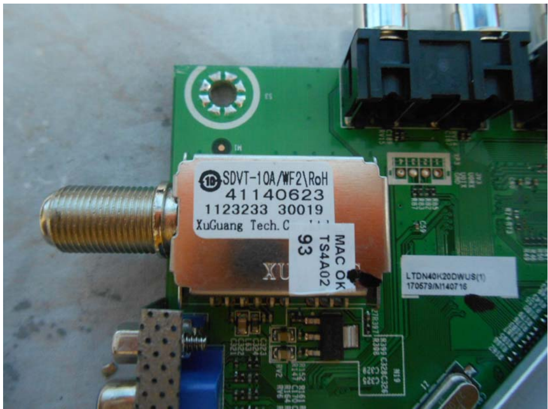
FIGURE 8 LED LCD TV (M/N: 40K20DW) TUNER ON MAIN BOARD
