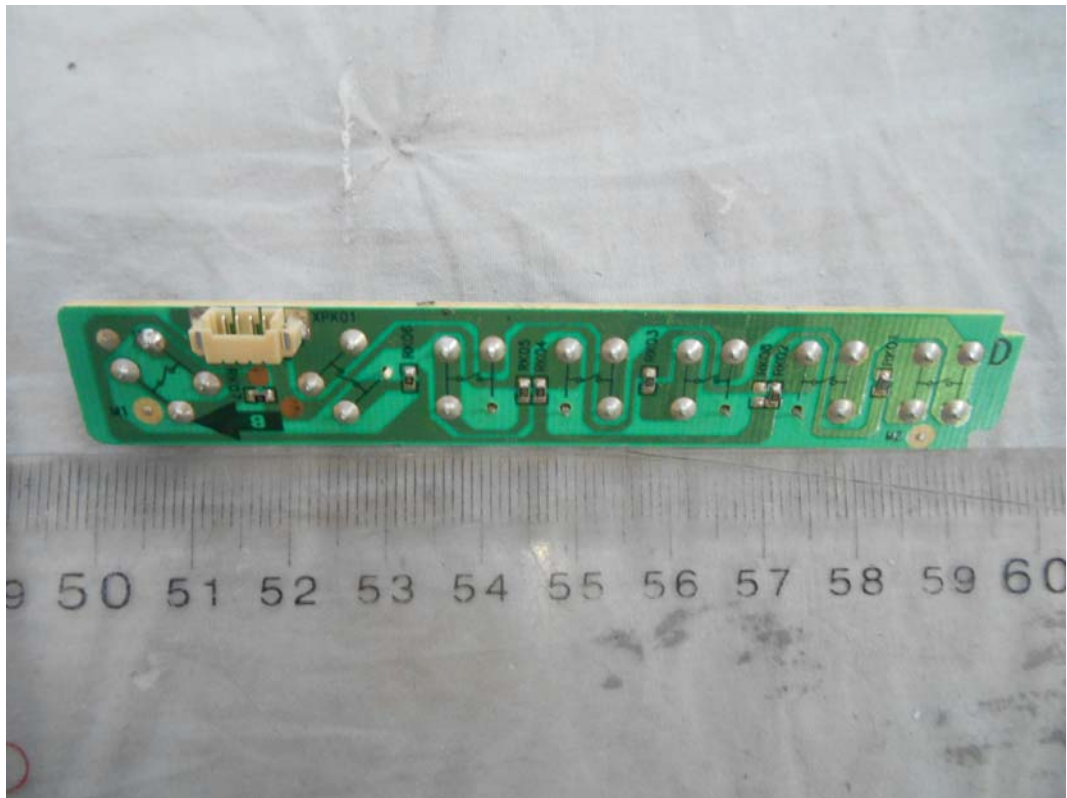
FIGURE 13 LED LCD TV (M/N: 40K20DW) KEY BOARD (SOLDERED SIDE)
