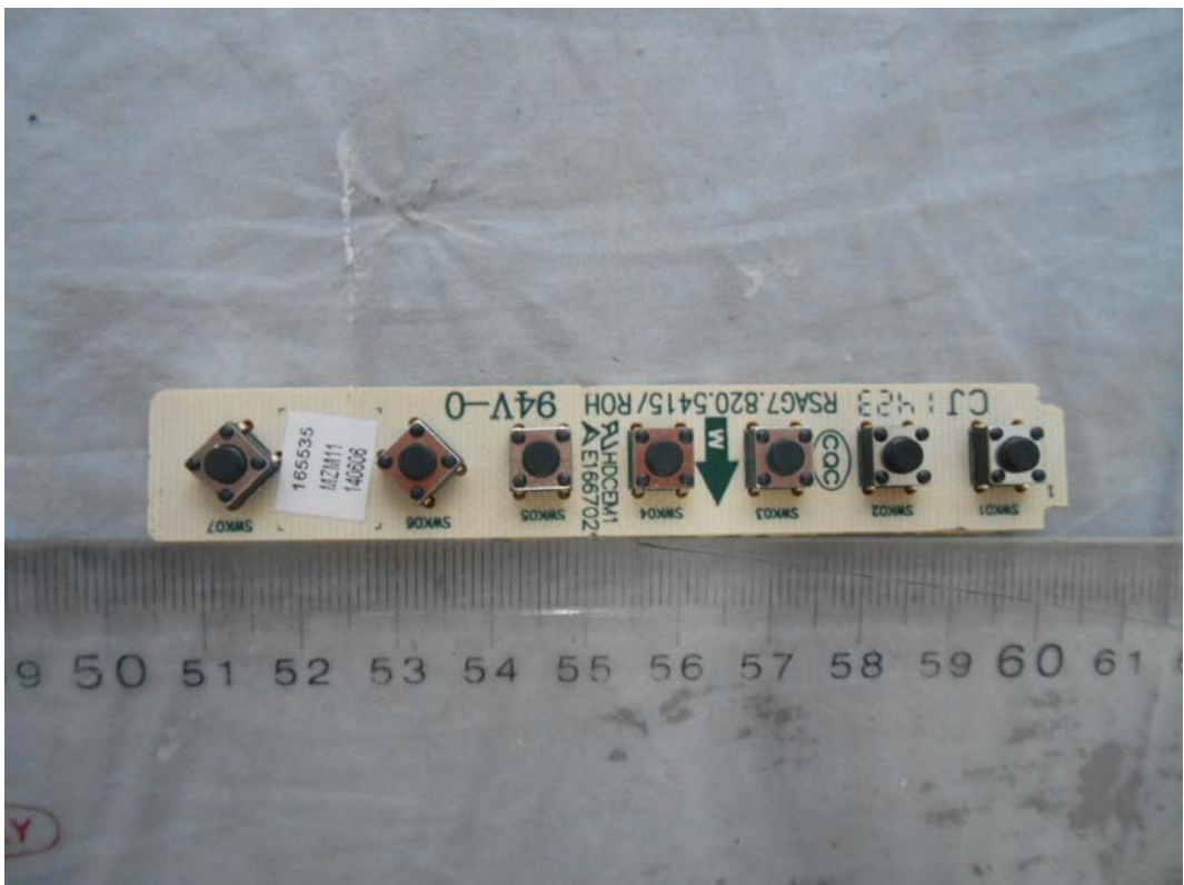
FIGURE 12 LED LCD TV (M/N: 40K20DW) KEY BOARD (COMPONENT SIDE)
