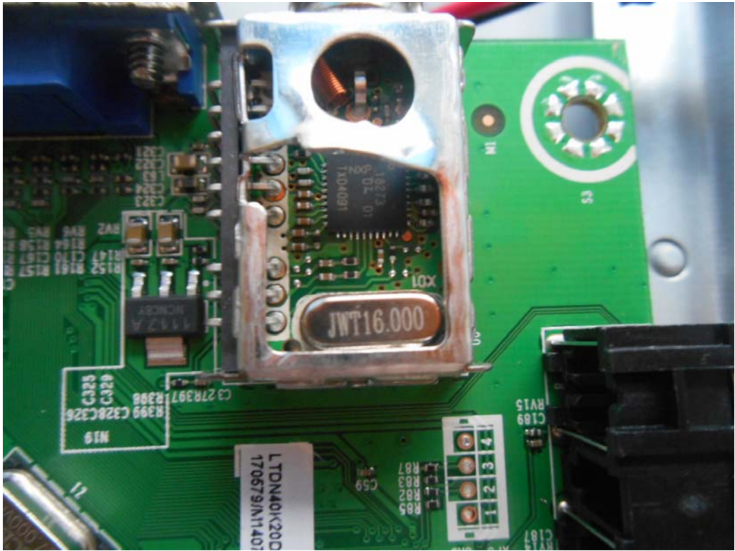
FIGURE 9 LED LCD TV (M/N: 40K20DW) TUNER COVER REMOVED
