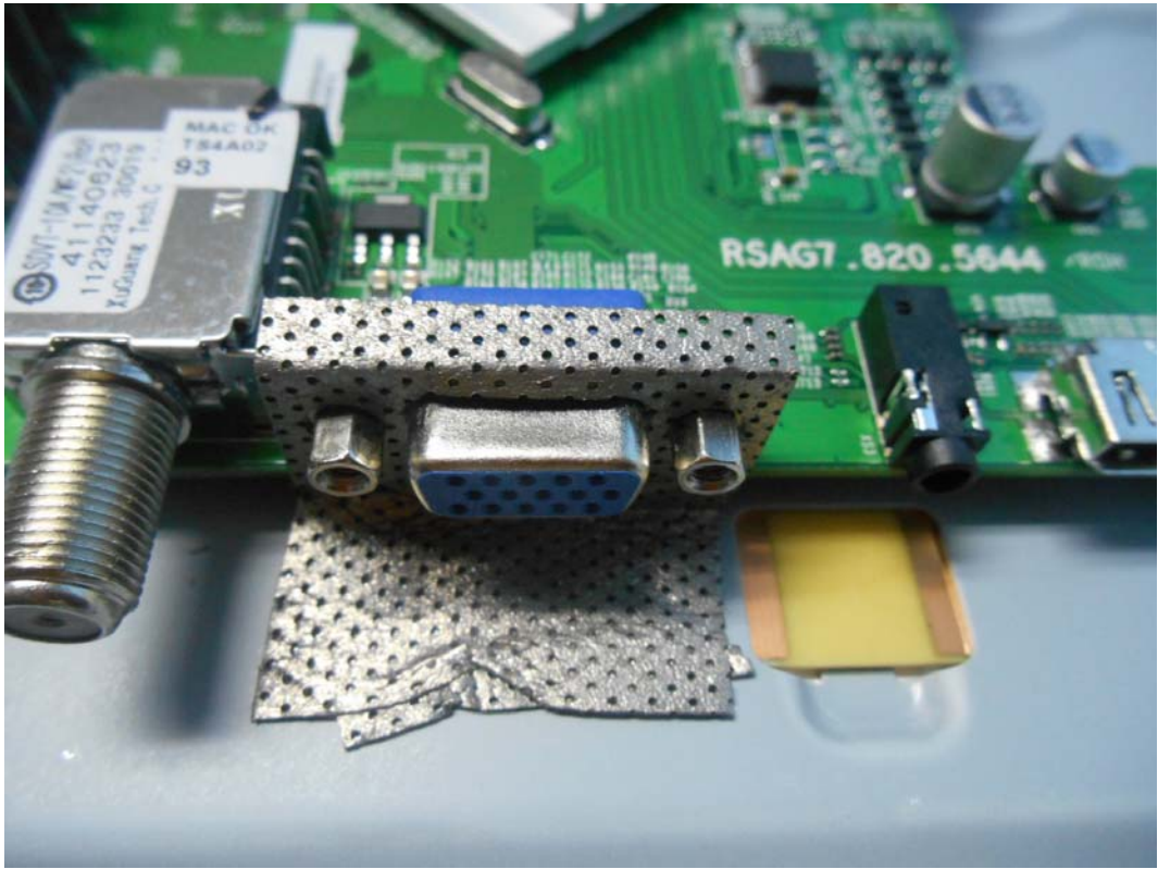
FIGURE 21 LED LCD TV (M/N: 40K20DW) DEBUG #1
