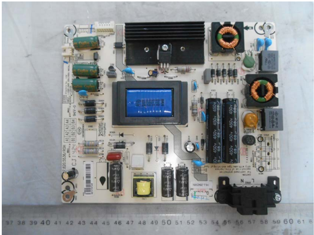
FIGURE 3 LED LCD TV (M/N: 40K20DW) POWER BOARD (COMPONENT SIDE)
