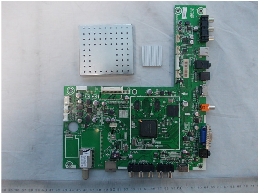
FIGURE 4 LED LCD TV (M/N: 39A300MH) MAIN BOARD (COMPONENT SIDE)
