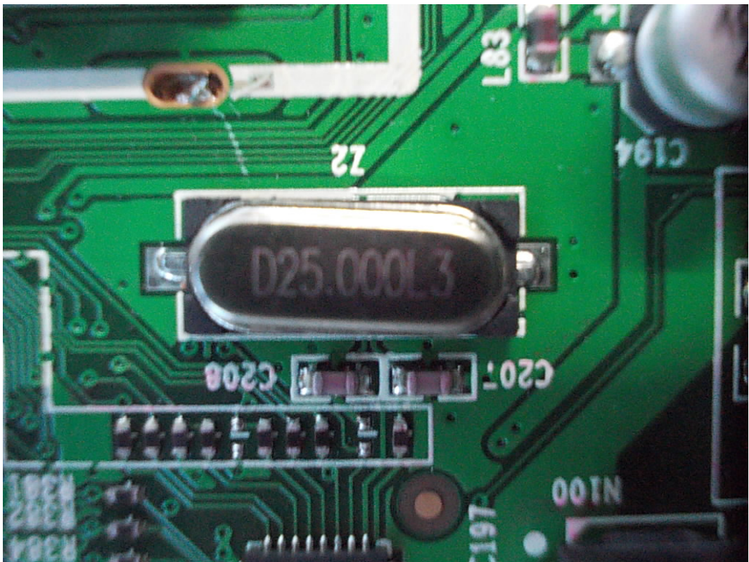
FIGURE 7 LED LCD TV (M/N: 39A300MH) CRYSTAL #1 ON MAIN BOARD
