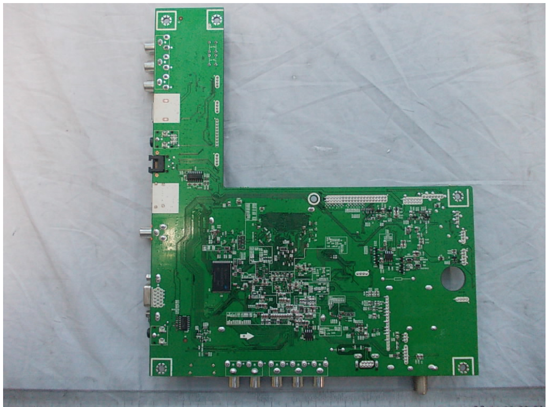
FIGURE 5 LED LCD TV (M/N: 39A300MH) MAIN BOARD (SOLDERED SIDE)
