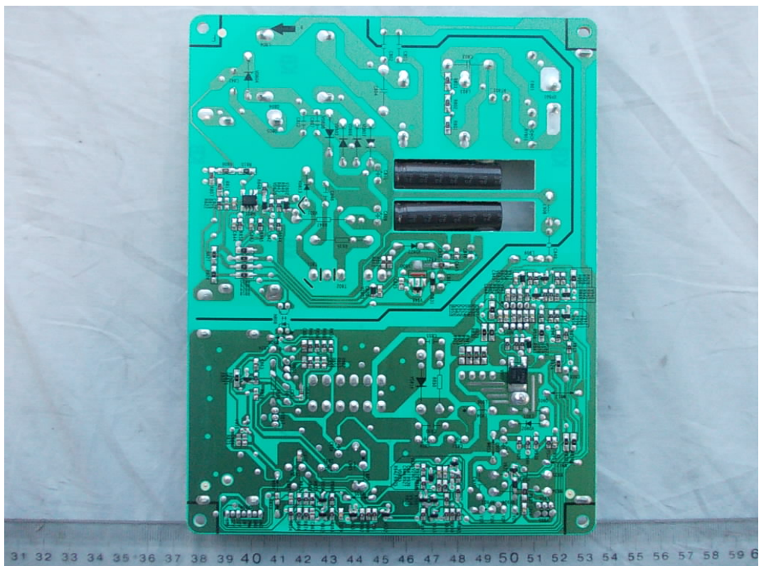
FIGURE 3 LED LCD TV (M/N: 39A300MH) POWER BOARD (SOLDERED SIDE)
