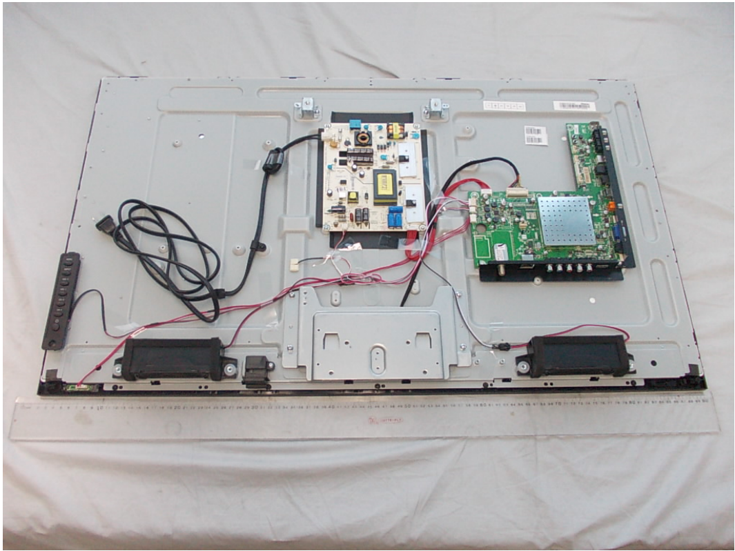
FIGURE 1 LED LCD TV (M/N: 39A300MH) COVER REMOVED
