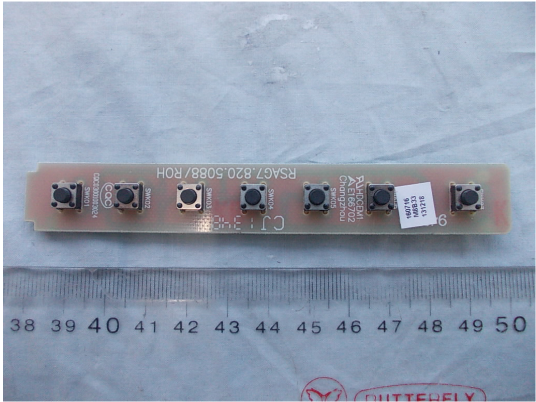
FIGURE 10 LED LCD TV (M/N: 39A300MH) KEY BOARD (COMPONENT SIDE)
