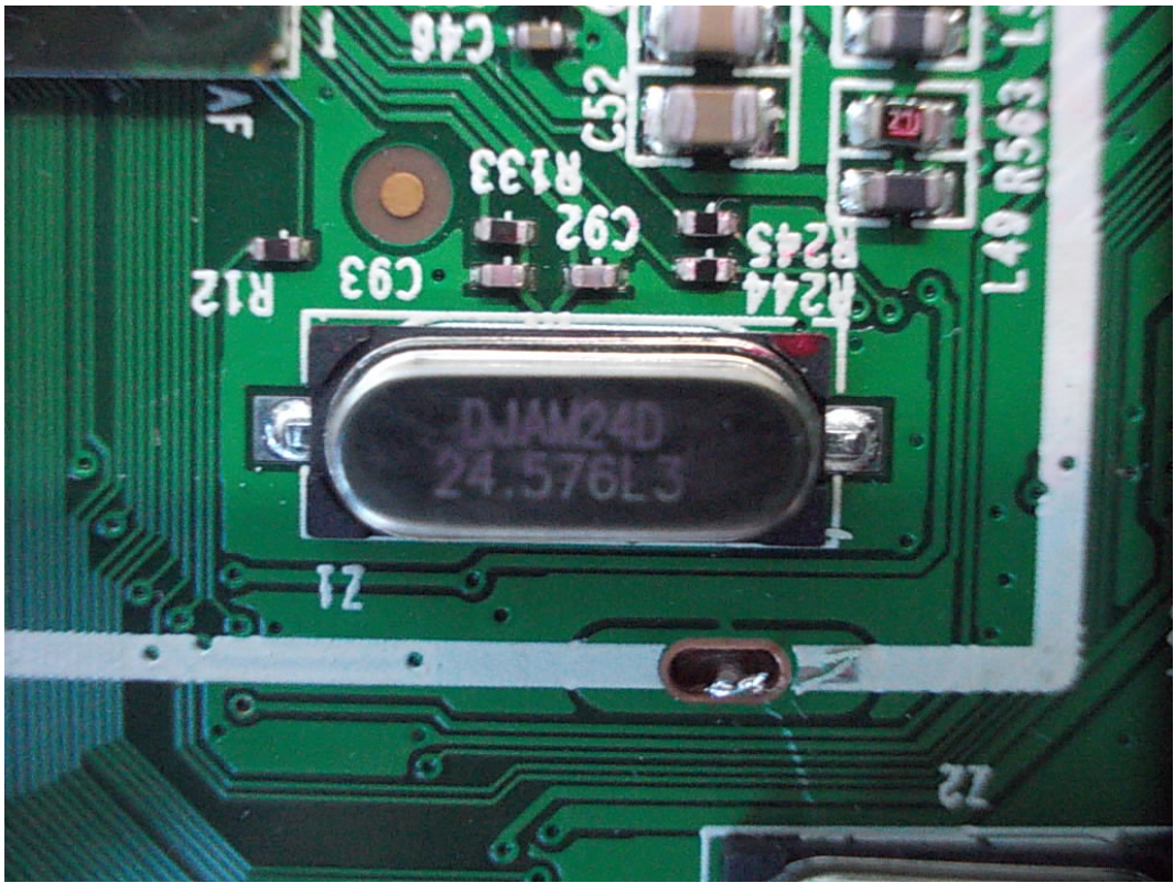
FIGURE 8 LED LCD TV (M/N: 39A300MH) CRYSTAL #2 ON MAIN BOARD
