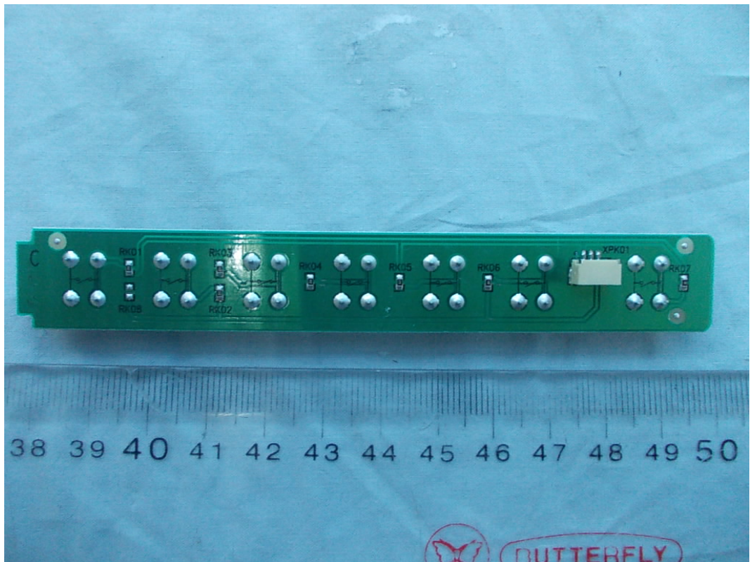
FIGURE 11 LED LCD TV (M/N: 39A300MH) KEY BOARD (SOLDERED SIDE)
