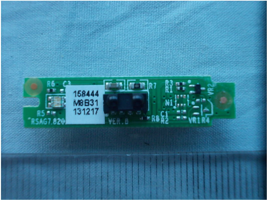
FIGURE 12 LED LCD TV (M/N: 39A300MH) IR BOARD (COMPONENT SIDE)
