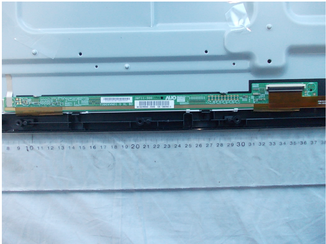
FIGURE 14 LED LCD TV (M/N: 39A300MH) LCD PANEL CONTROL BOARD (FRONT SIDE)
