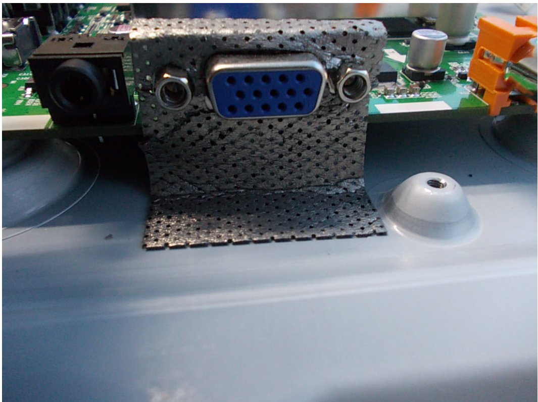
FIGURE 17 LED LCD TV (M/N: 39A300MH) DEBUG #2
