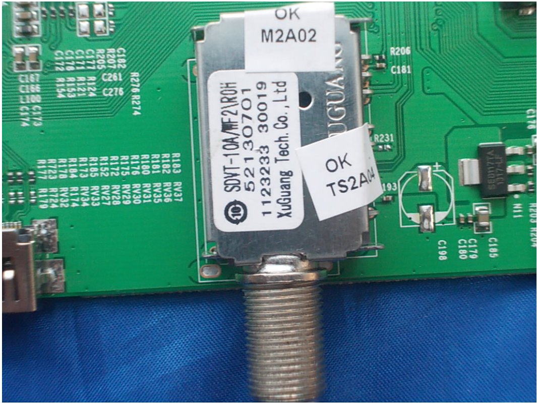
FIGURE 7 LED LCD TV (M/N: LTDN42A300US) TUNER ON MAIN BOARD
