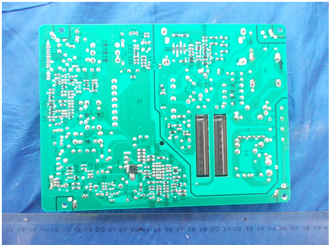
FIGURE 4 LED LCD TV (M/N: LTDN42A300US) POWER BOARD (SOLDERED SIDE)
