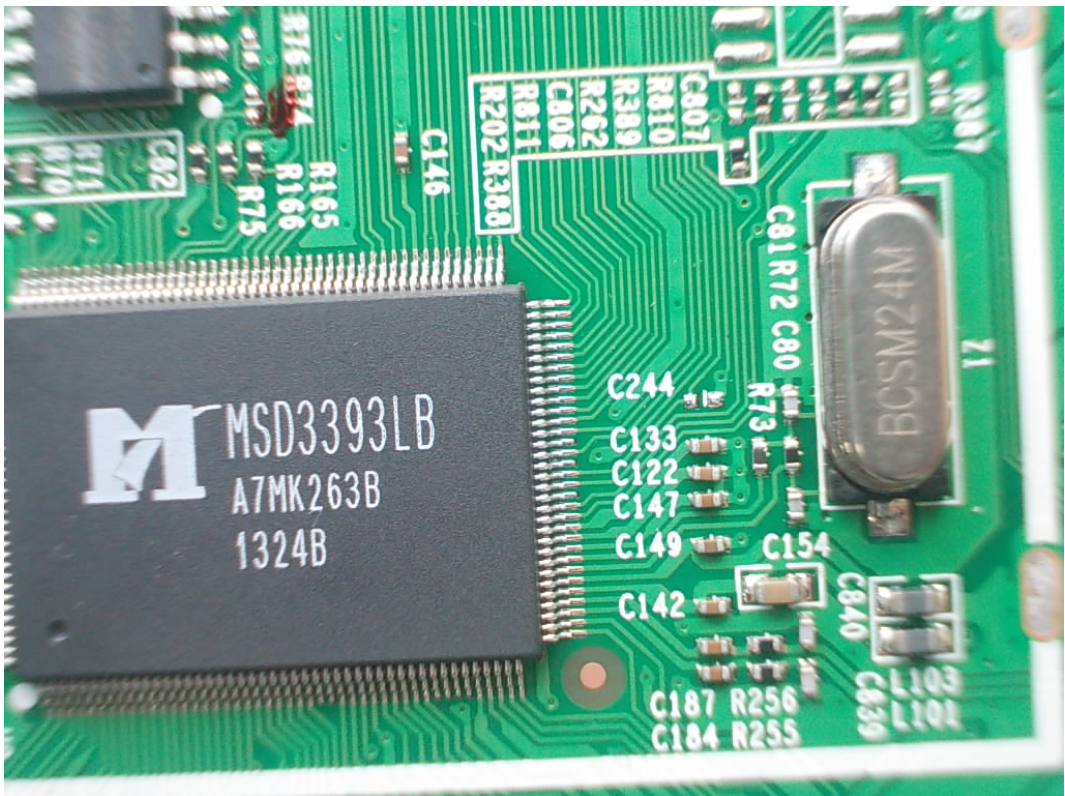
FIGURE 8 LED LCD TV (M/N: LTDN42A300US) CHIP & CRYSTAL ON MAIN BOARD
