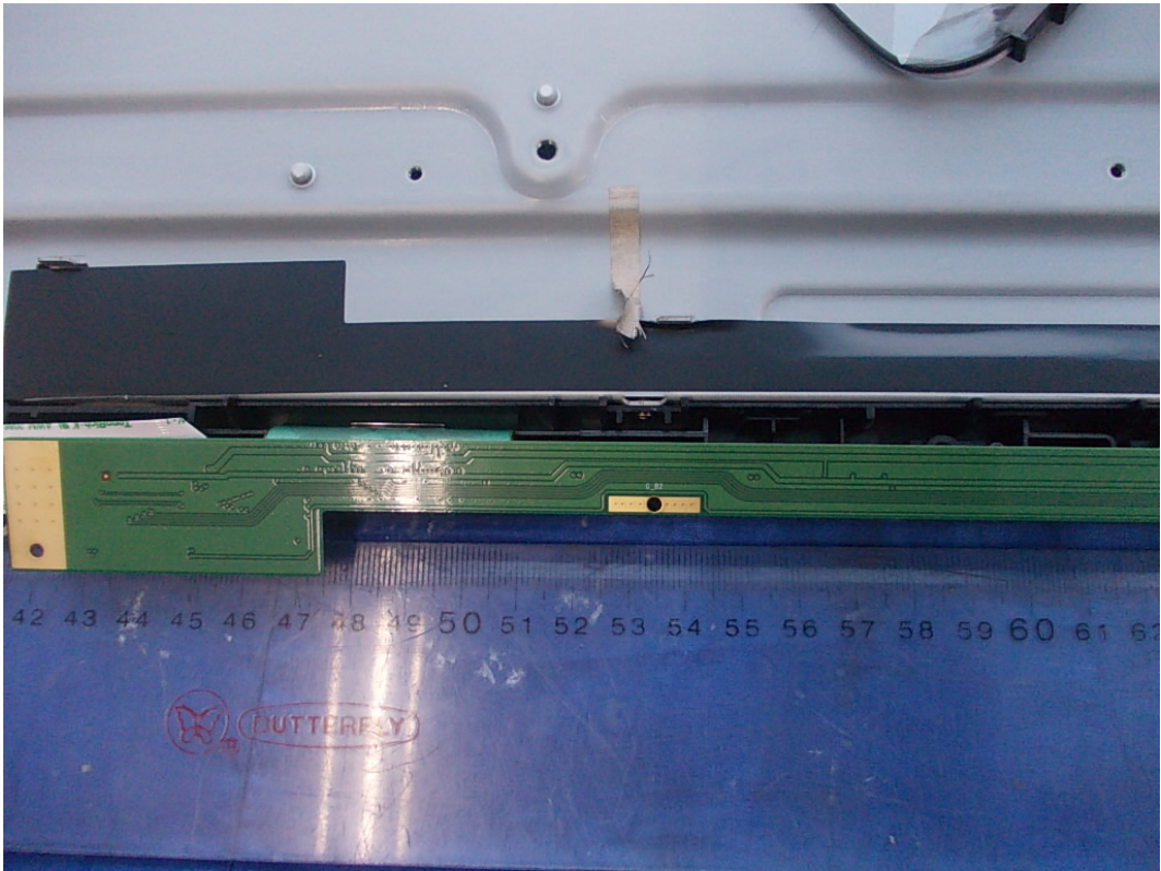
FIGURE 16 LED LCD TV (M/N: LTDN42A300US) LCD PANEL CONTROL BOARD (SOLDERED SIDE #3)
