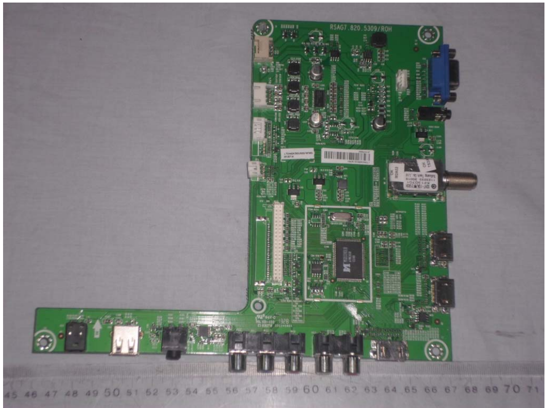
FIGURE 5 LED LCD TV (M/N: LTDN42A300US) MAIN BOARD (COMPONENT SIDE)
