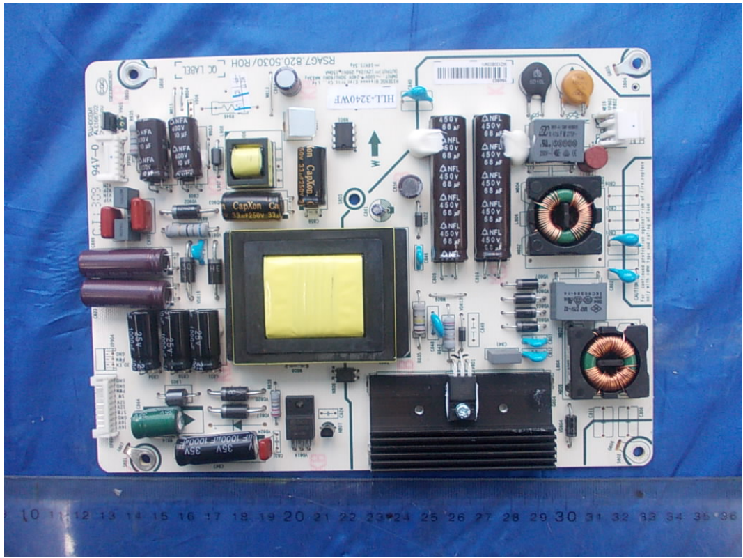
FIGURE 3 LED LCD TV (M/N: LTDN42A300US) POWER BOARD (COMPONENT SIDE)
