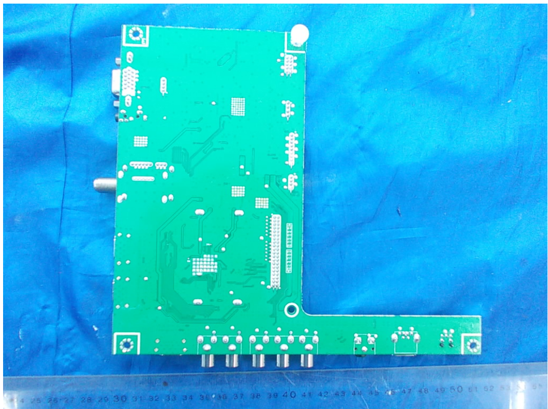
FIGURE 6 LED LCD TV (M/N: LTDN42A300US) MAIN BOARD (SOLDERED SIDE)
