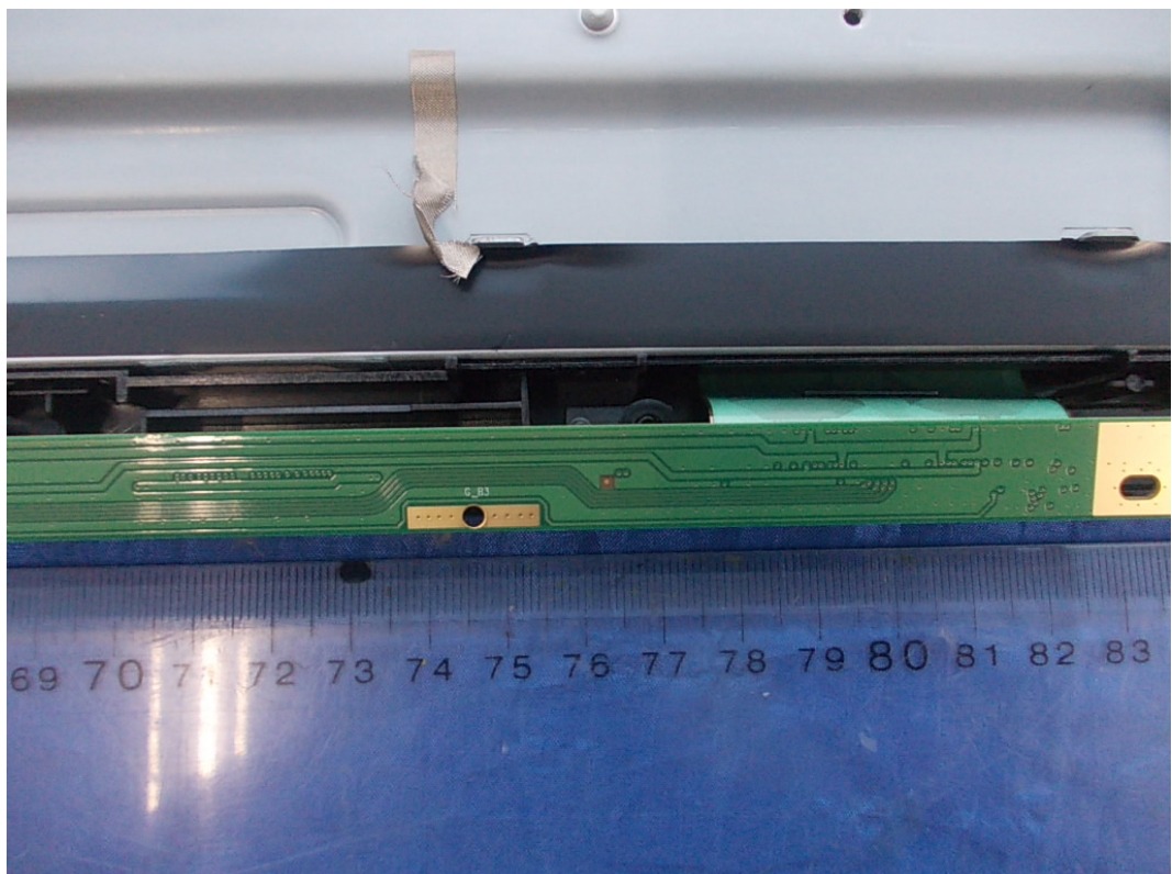
FIGURE 14 LED LCD TV (M/N: LTDN42A300US) LCD PANEL CONTROL BOARD (SOLDERED SIDE #1)
