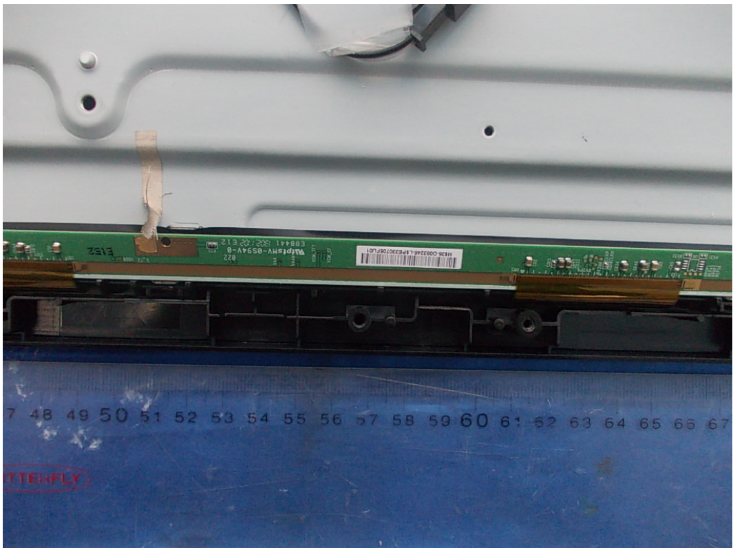
FIGURE 12 LED LCD TV (M/N: LTDN42A300US) LCD PANEL CONTROL BOARD (COMPONENT SIDE #2)
