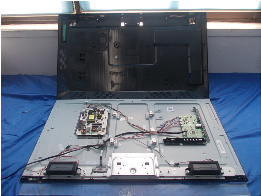
FIGURE 1 LED LCD TV (M/N: LTDN42A300US) COVER REMOVED
