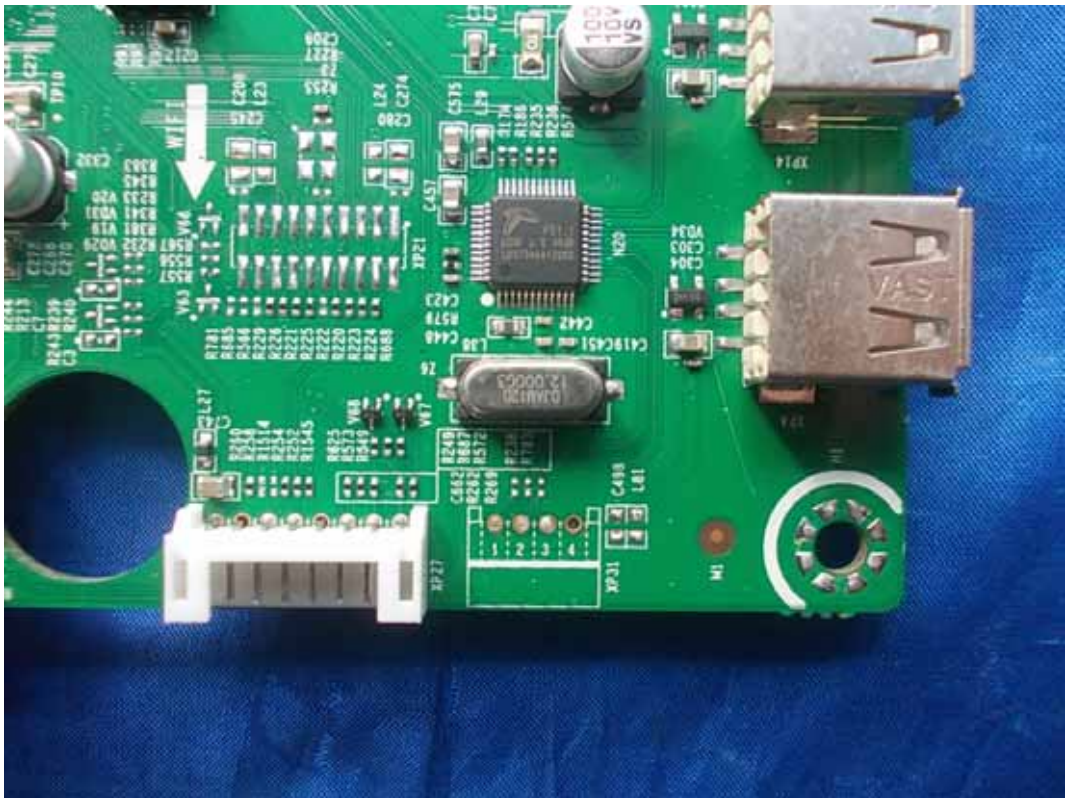
FIGURE 11 LED LCD TV (M/N: 40K368AW) CRYSTAL #2 ON MAIN BOARD
