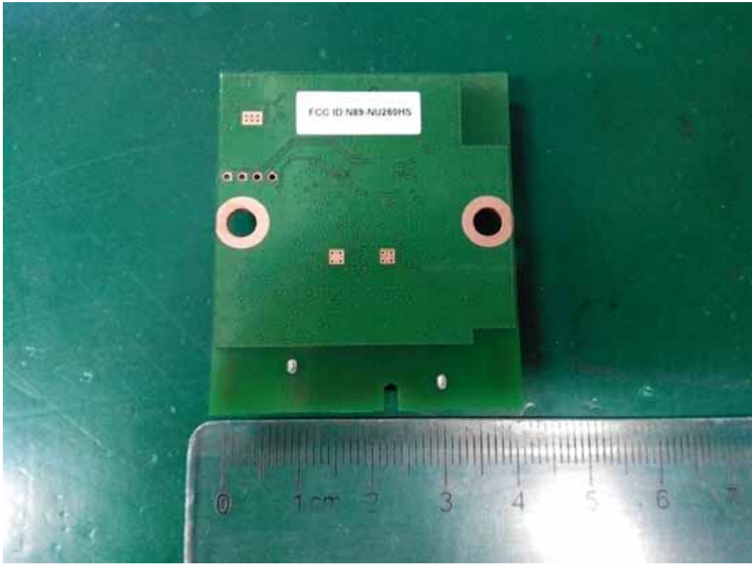
FIGURE 13 LED LCD TV (M/N: 40K368AW) RF BOARD (SOLDERED SIDE)
