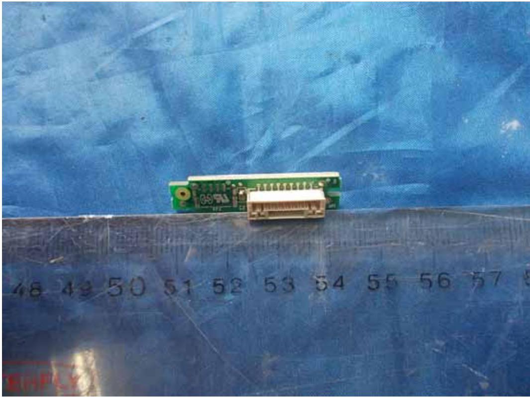
FIGURE 19 LED LCD TV (M/N: 40K368AW) IR BOARD (SOLDERED SIDE)
