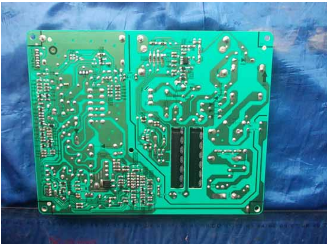
FIGURE 4 LED LCD TV (M/N: 40K368AW) POWER BOARD (SOLDERED SIDE)
