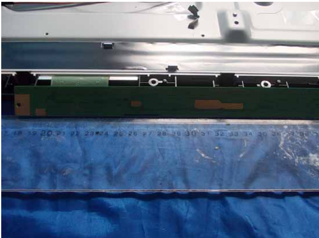
FIGURE 16 LED LCD TV (M/N: 40K368AW) LCD PANEL CONTROL BOARD (SOLDERED SIDE)
