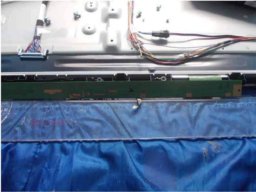
FIGURE 17 LED LCD TV (M/N: 40K368AW) LCD PANEL CONTROL BOARD (SOLDERED SIDE)
