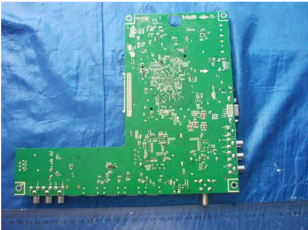
FIGURE 6 LED LCD TV (M/N: 40K368AW) MAIN BOARD (SOLDERED SIDE)
