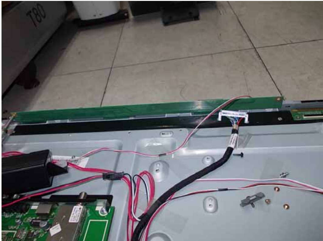
FIGURE 17 LED LCD TV (M/N: LTDN39K366MH) LCD PANEL CONTROL BOARD
