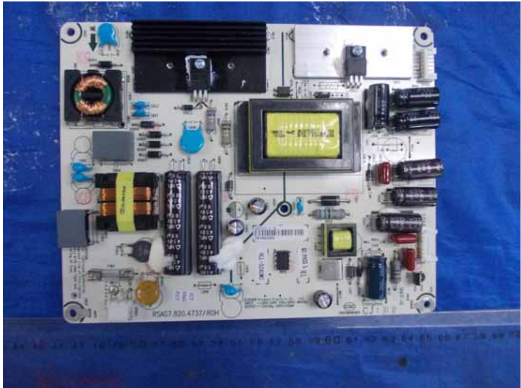
FIGURE 3 LED LCD TV (M/N: LTDN39K366MH) POWER BOARD (COMPONENT SIDE)
