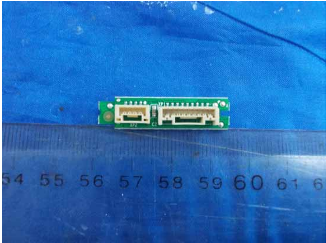
FIGURE 13 LED LCD TV (M/N: LTDN39K366MH) IR BOARD (SOLDERED SIDE)
