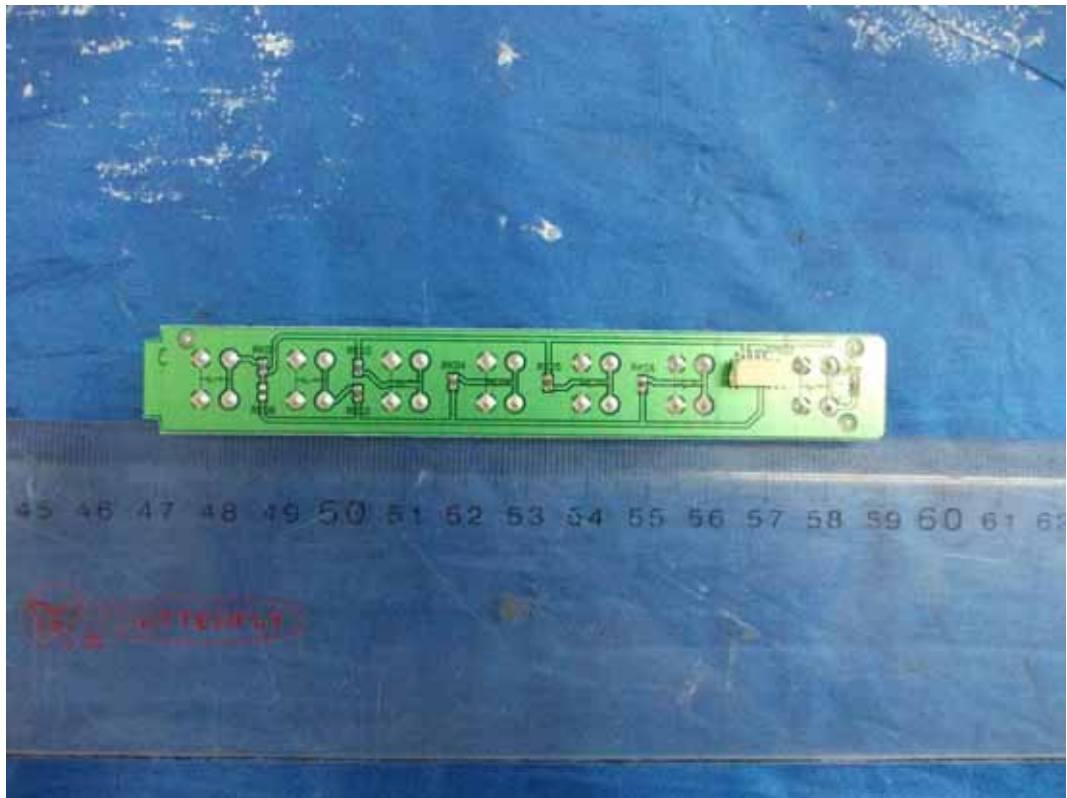
FIGURE 11 LED LCD TV (M/N: LTDN39K366MH) KEY BOARD (SOLDERED SIDE)
