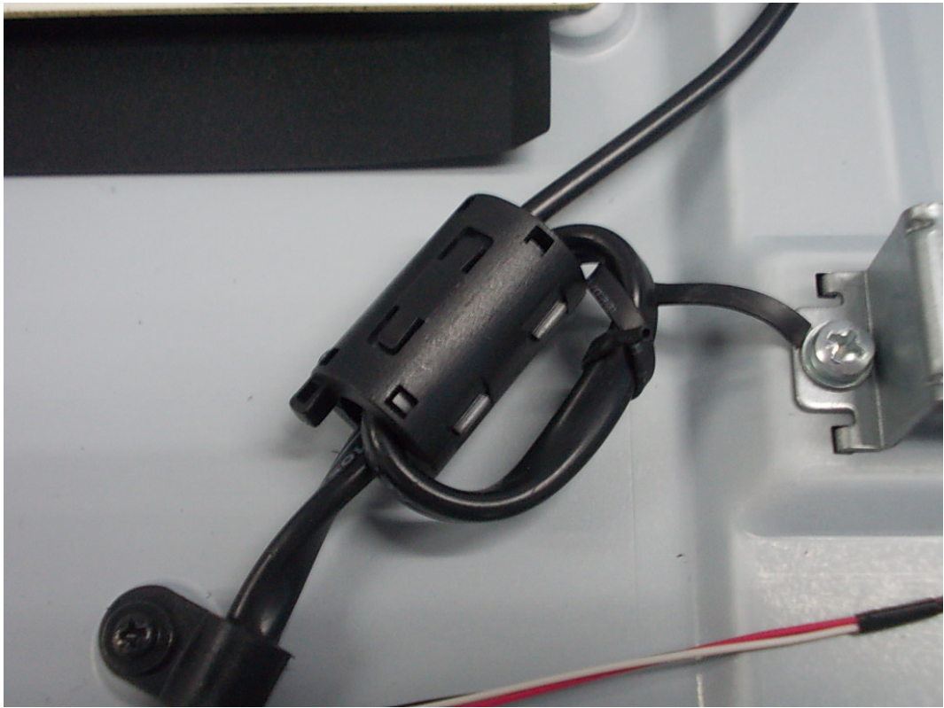
FIGURE 16 LED LCD TV (M/N: 40K360MN) DEBUG 1
