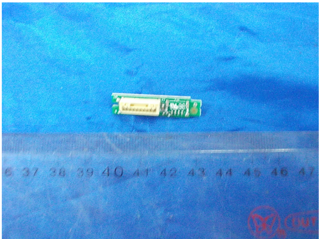
FIGURE 12 LED LCD TV (M/N: 40K360MN) IR BOARD (SOLDERED SIDE)
