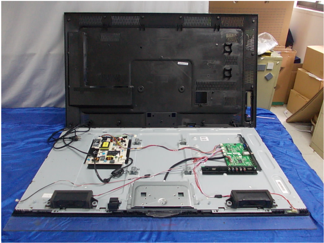
FIGURE 1 LED LCD TV (M/N: 40K360MN) COVER REMOVED
