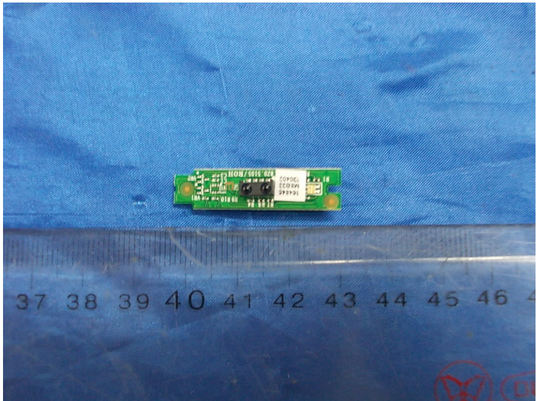
FIGURE 11 LED LCD TV (M/N: 40K360MN) IR BOARD (COMPONENT SIDE)
