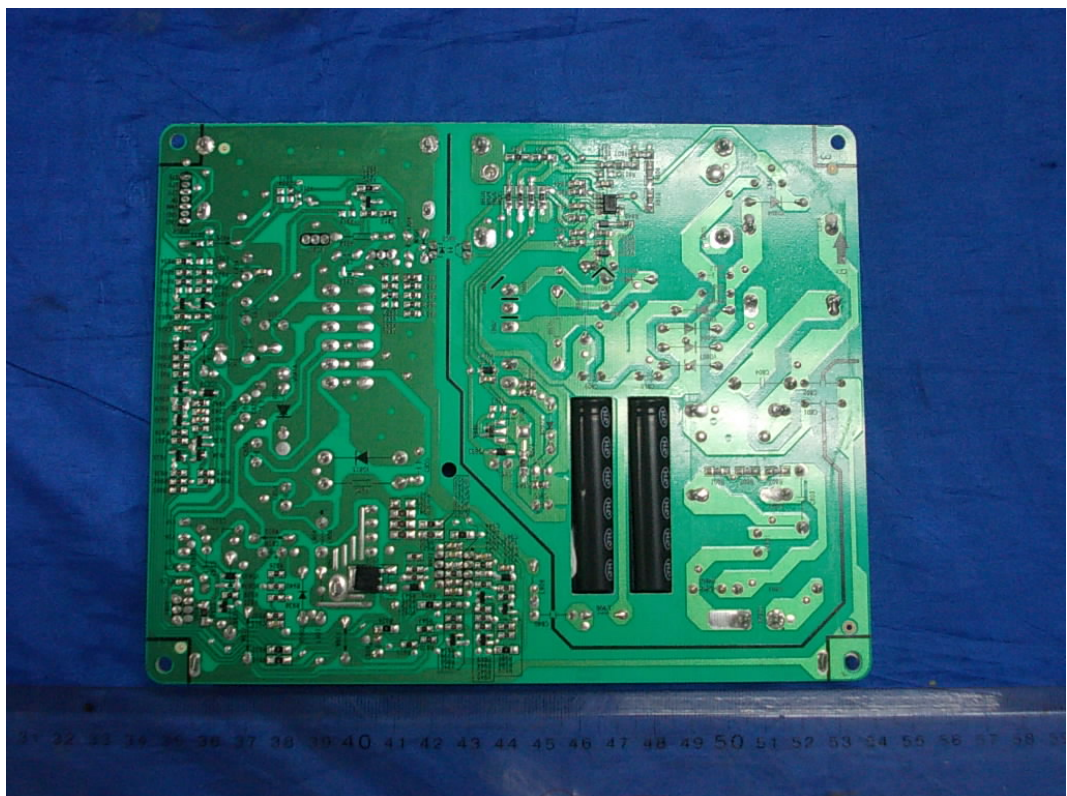
FIGURE 4 LED LCD TV (M/N: 40K360MN) POWER BOARD (SOLDERED SIDE)
