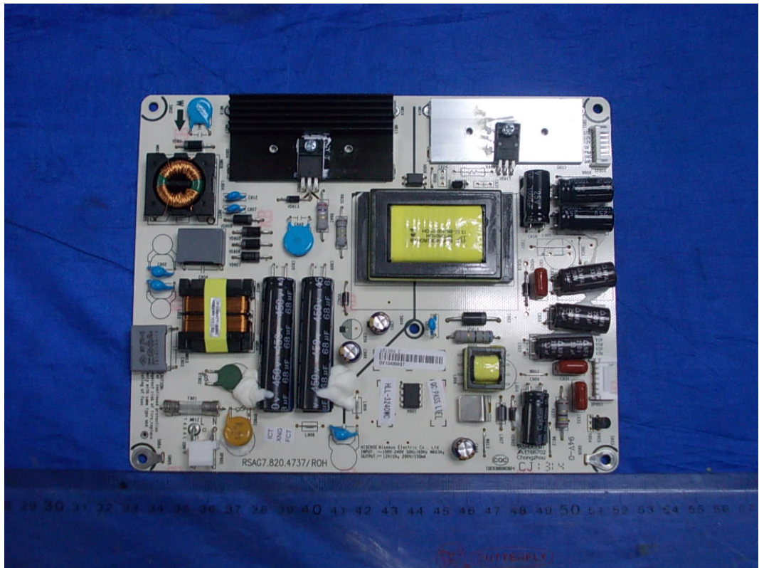
FIGURE 3 LED LCD TV (M/N: 40K360MN) POWER BOARD (COMPONENT SIDE)
