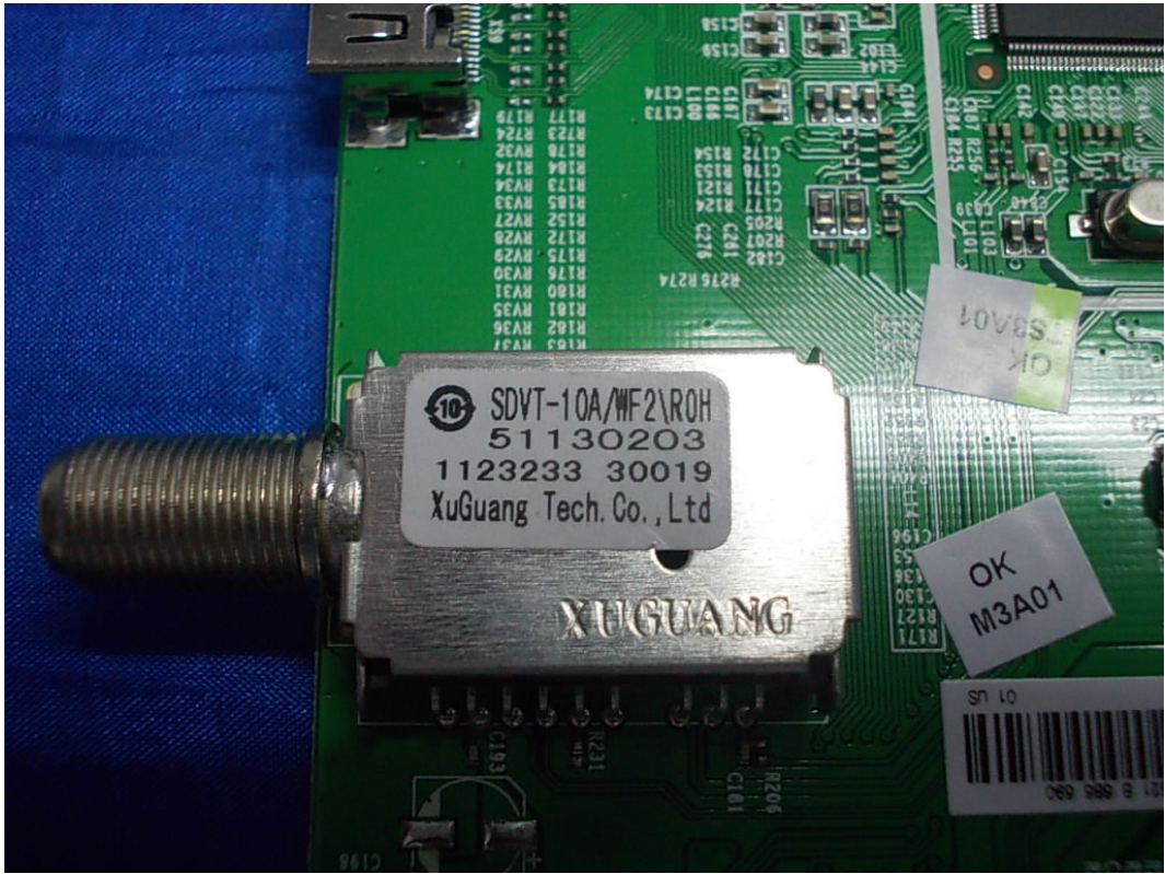
FIGURE 7 LED LCD TV (M/N: 40K360MN) TUNER ON MAIN BOARD
