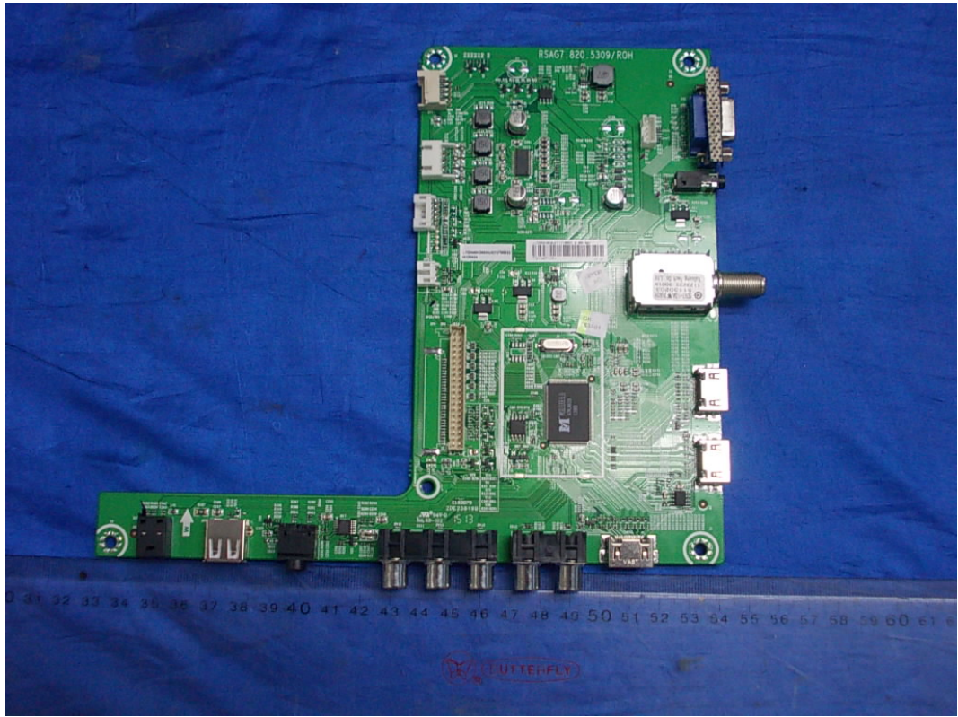
FIGURE 5 LED LCD TV (M/N: 40K360MN) MAIN BOARD (COMPONENT SIDE)
