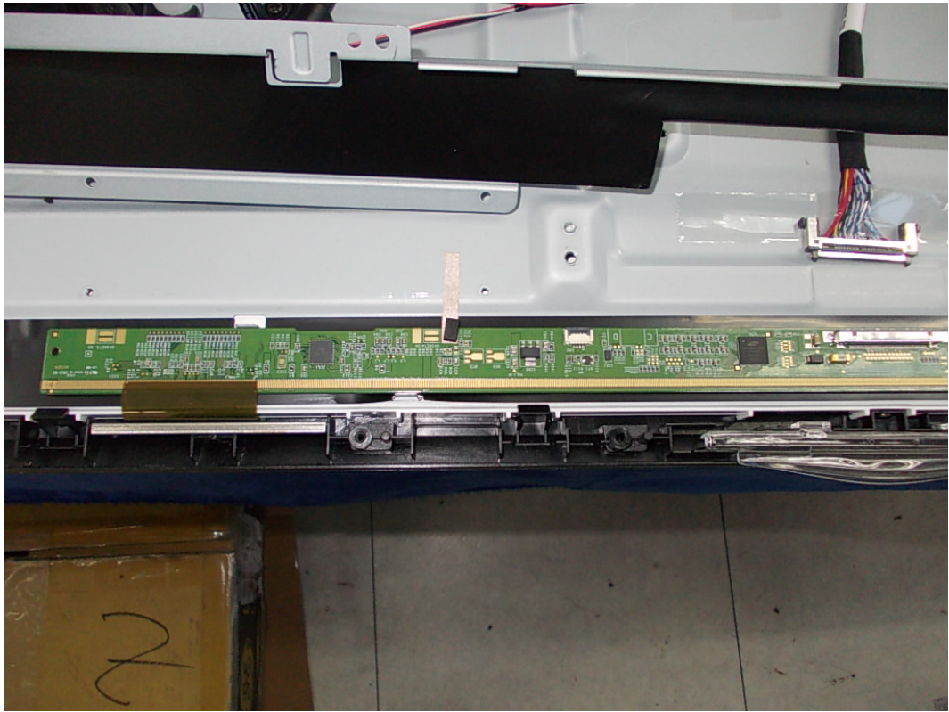
FIGURE 13 LED LCD TV (M/N: 40K360MN) LCD PANEL CONTROL BOARD (COMPONENT SIDE #1)
