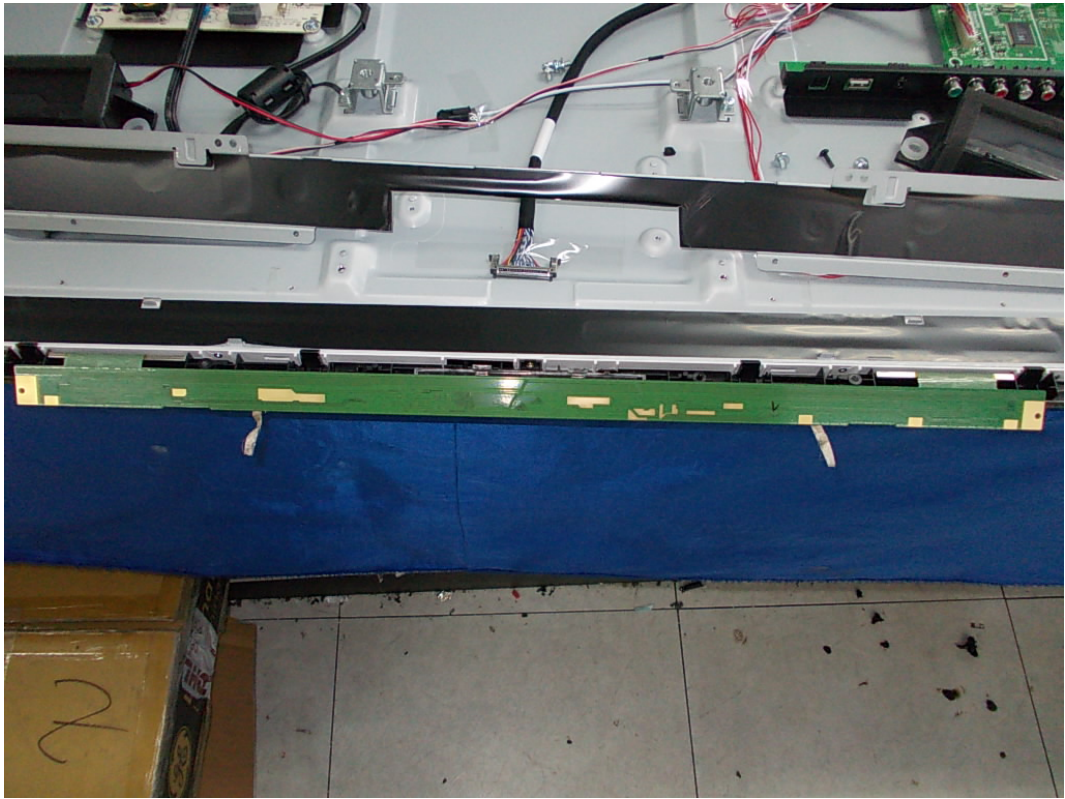
FIGURE 15 LED LCD TV (M/N: 40K360MN) LCD PANEL CONTROL BOARD (SOLDERED SIDE)
