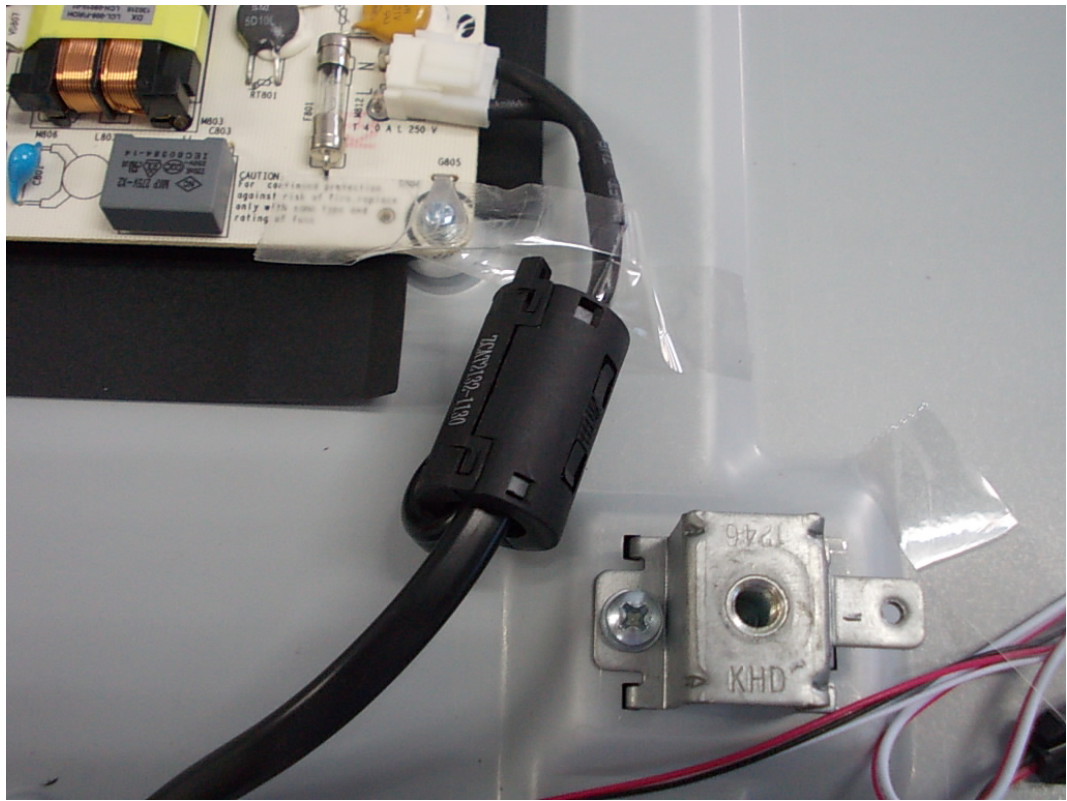
FIGURE 16 LED LCD TV (M/N: 40K366WN) DEBUG 1
