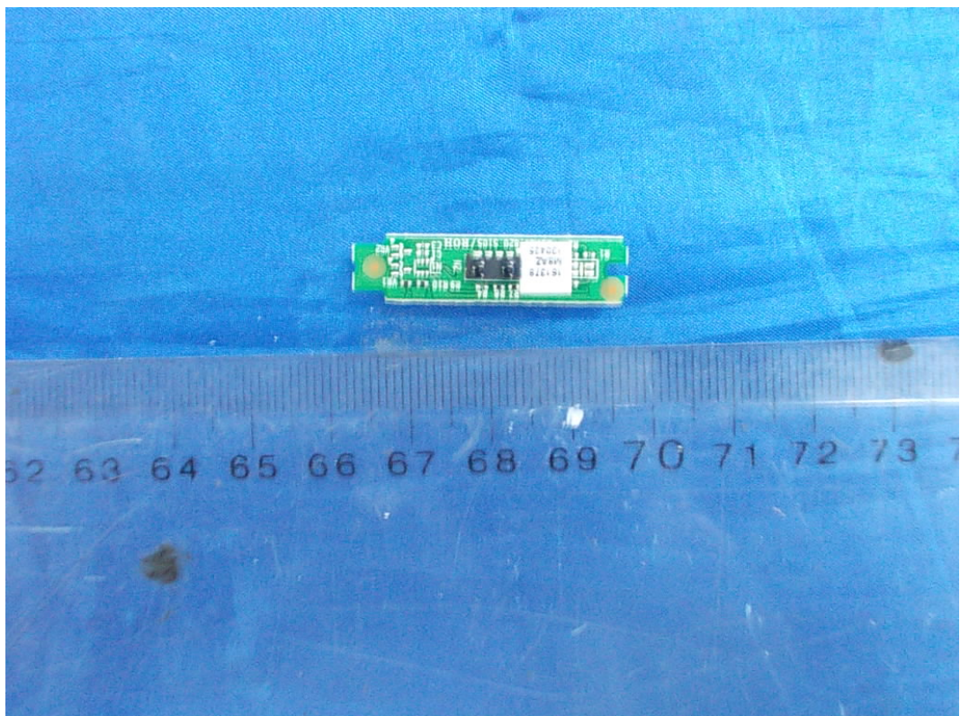
FIGURE 15 LED LCD TV (M/N: 40K366WN) IR BOARD (SOLDERED SIDE)
