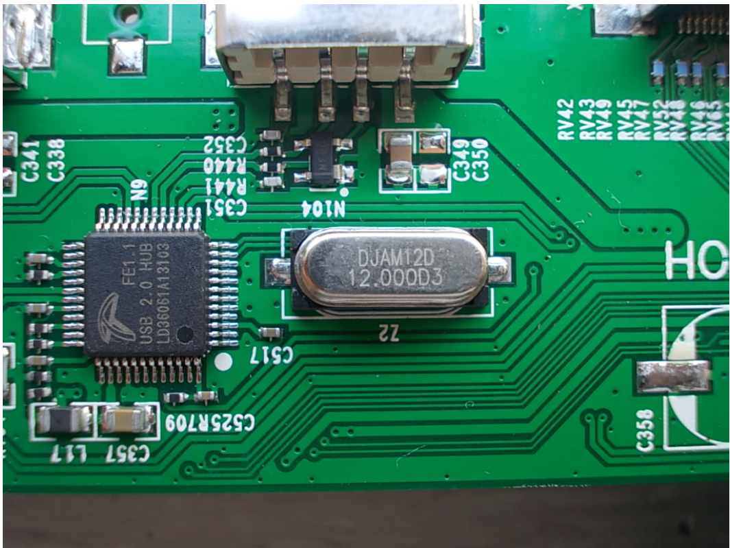
FIGURE 10 LED LCD TV (M/N: 40K366WN) CRYSTAL #2 ON MAIN BOARD
