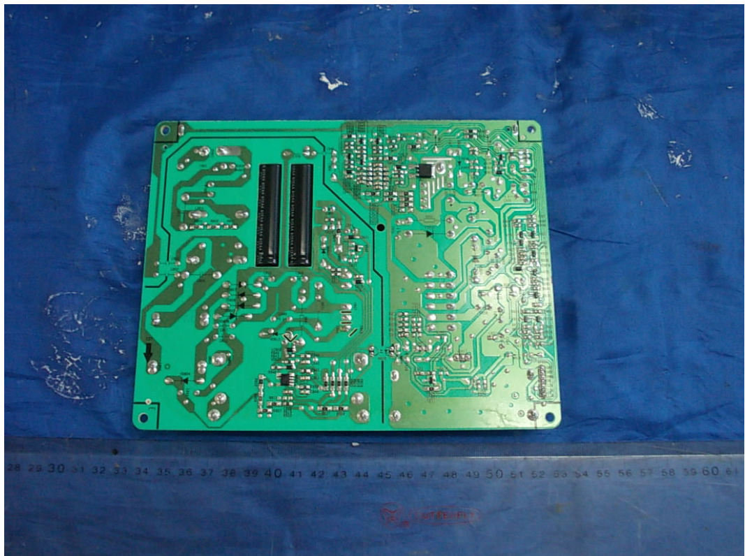
FIGURE 4 LED LCD TV (M/N: 40K366WN) POWER BOARD (SOLDERED SIDE)
