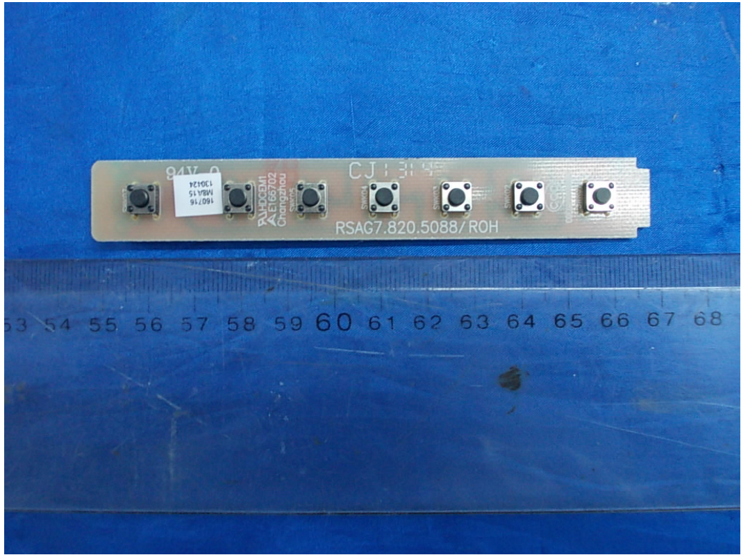
FIGURE 12 LED LCD TV (M/N: 40K366WN) KEY BOARD (COMPONENT SIDE)
