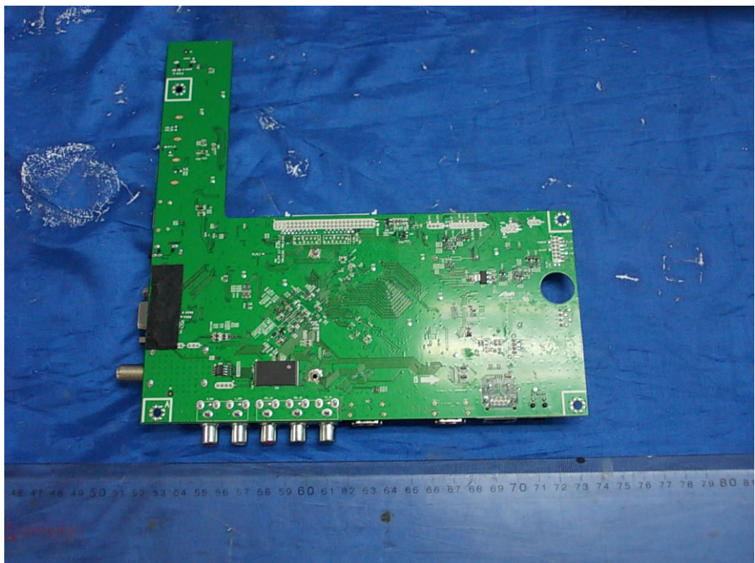
FIGURE 6 LED LCD TV (M/N: 40K366WN) MAIN BOARD (SOLDERED SIDE)
