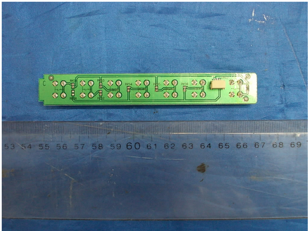
FIGURE 13 LED LCD TV (M/N: 40K366WN) KEY BOARD (SOLDERED SIDE)
