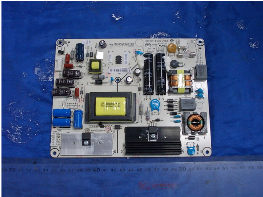
FIGURE 3 LED LCD TV (M/N: 40K366WN) POWER BOARD (COMPONENT SIDE)
