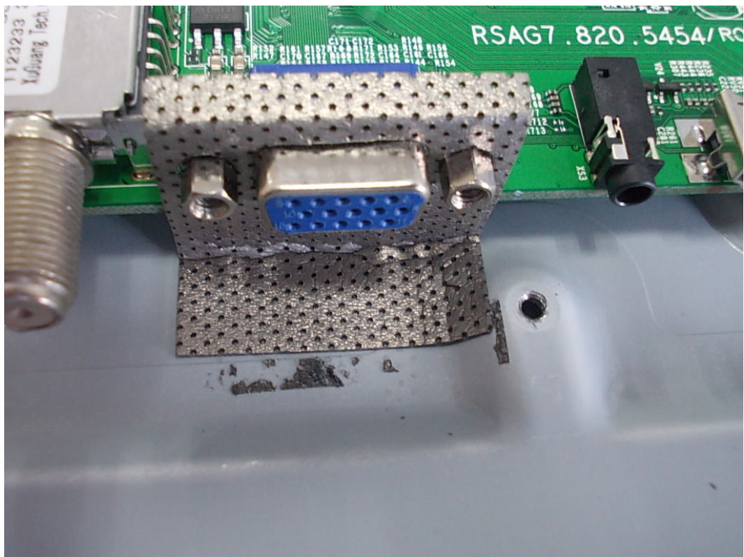
FIGURE 17 LED LCD TV (M/N: 40K366WN) DEBUG 2
