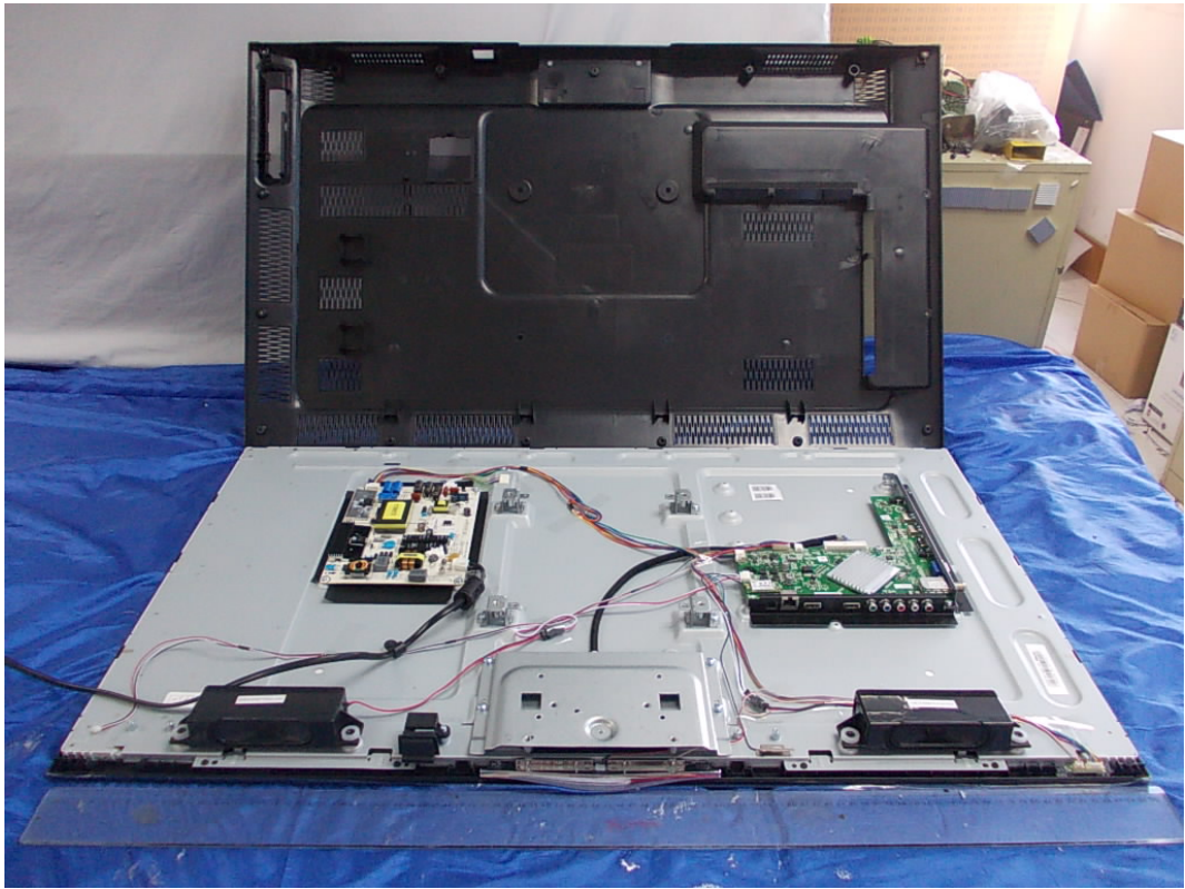
FIGURE 1 LED LCD TV (M/N: 40K366WN) COVER REMOVED
