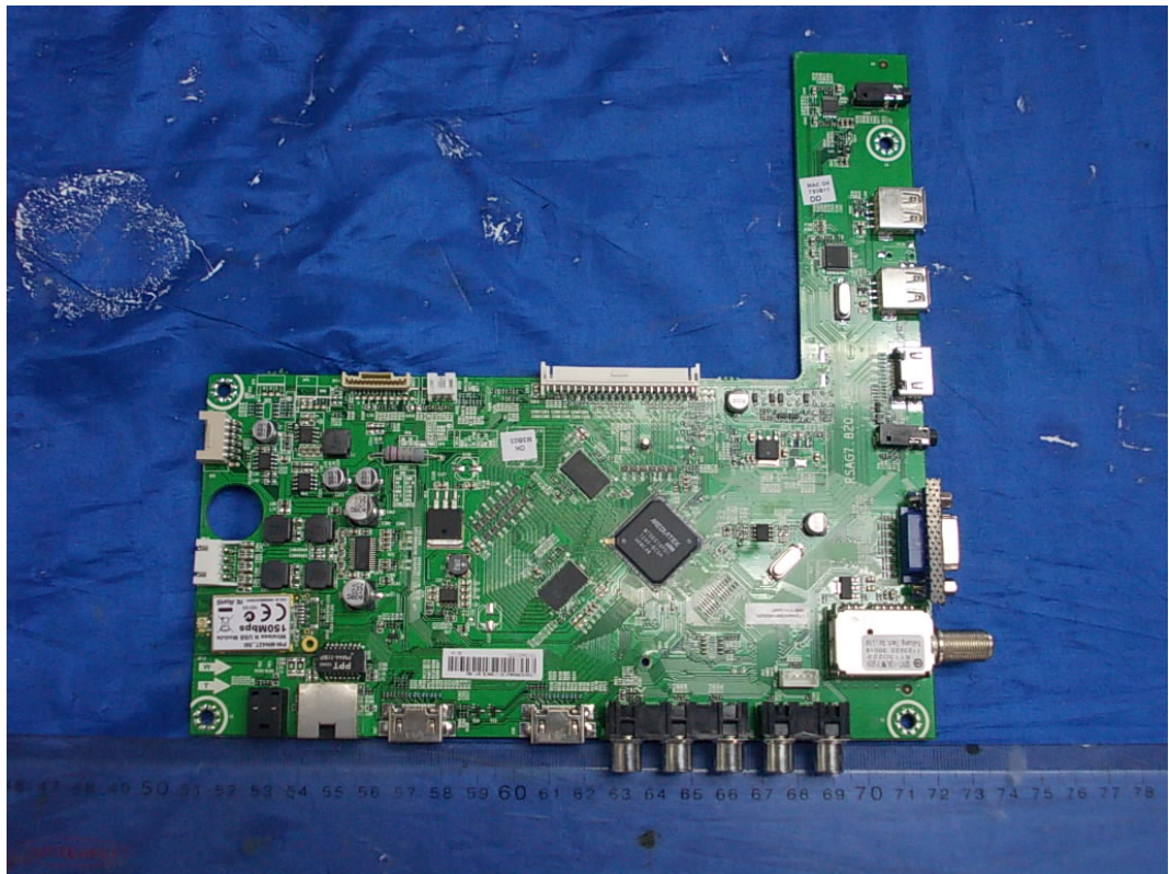
FIGURE 5 LED LCD TV (M/N: 40K366WN) MAIN BOARD (COMPONENT SIDE)
