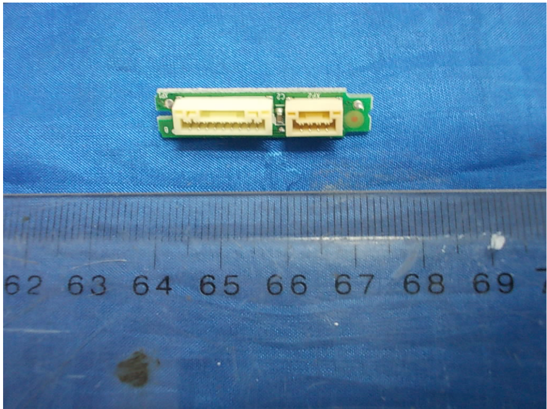
FIGURE 14 LED LCD TV (M/N: 40K366WN) IR BOARD (COMPONENT SIDE)
