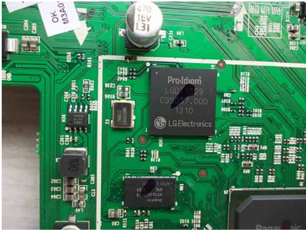
FIGURE 9 LED LCD TV (M/N: LTDN42A300MH) CRYSTAL #3 ON MAIN BOARD
