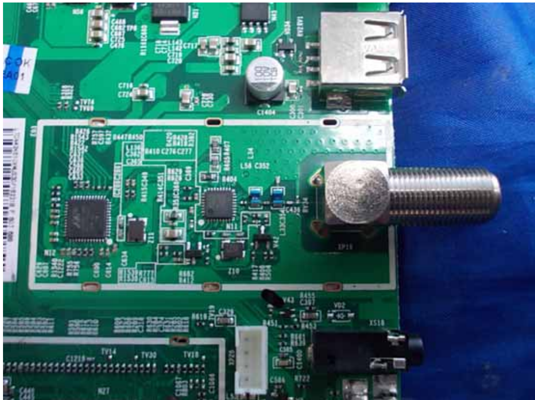
FIGURE 7 LED LCD TV (M/N: LTDN42K610XWUS3D) TUNER ON MAIN BOARD
