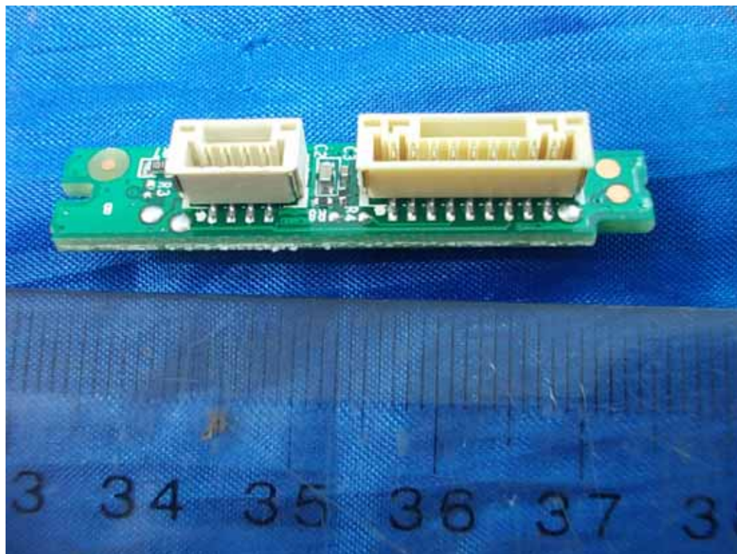
FIGURE 15 LED LCD TV (M/N: LTDN42K610XWUS3D) IR BOARD (SOLDERED SIDE)
