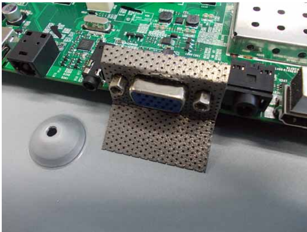
FIGURE 21 LED LCD TV (M/N: LTDN42K610XWUS3D) DEBUG #2
