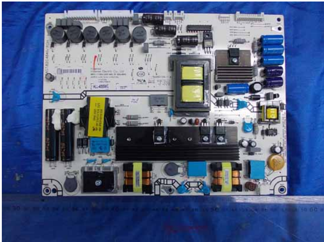
FIGURE 3 LED LCD TV (M/N: LTDN42K610XWUS3D) POWER BOARD (COMPONENT SIDE)
