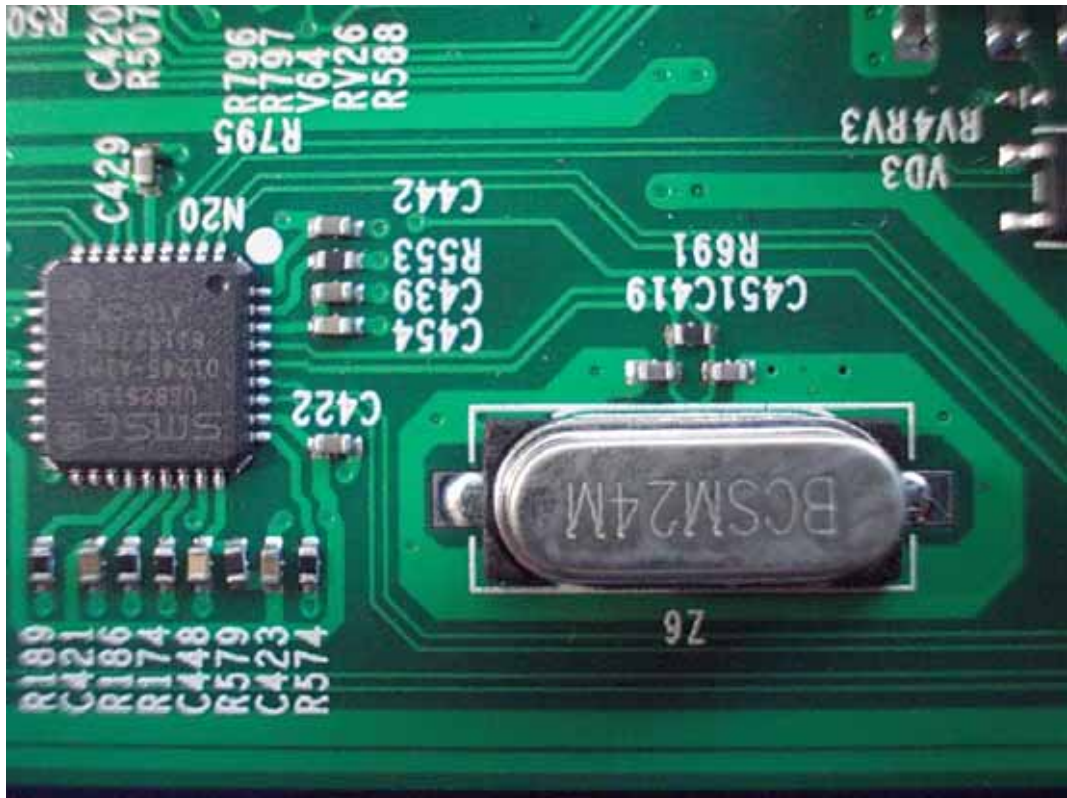
FIGURE 9 LED LCD TV (M/N: LTDN42K610XWUS3D) CHIP #2 & CRYSTAL #1 ON MAIN BOARD
