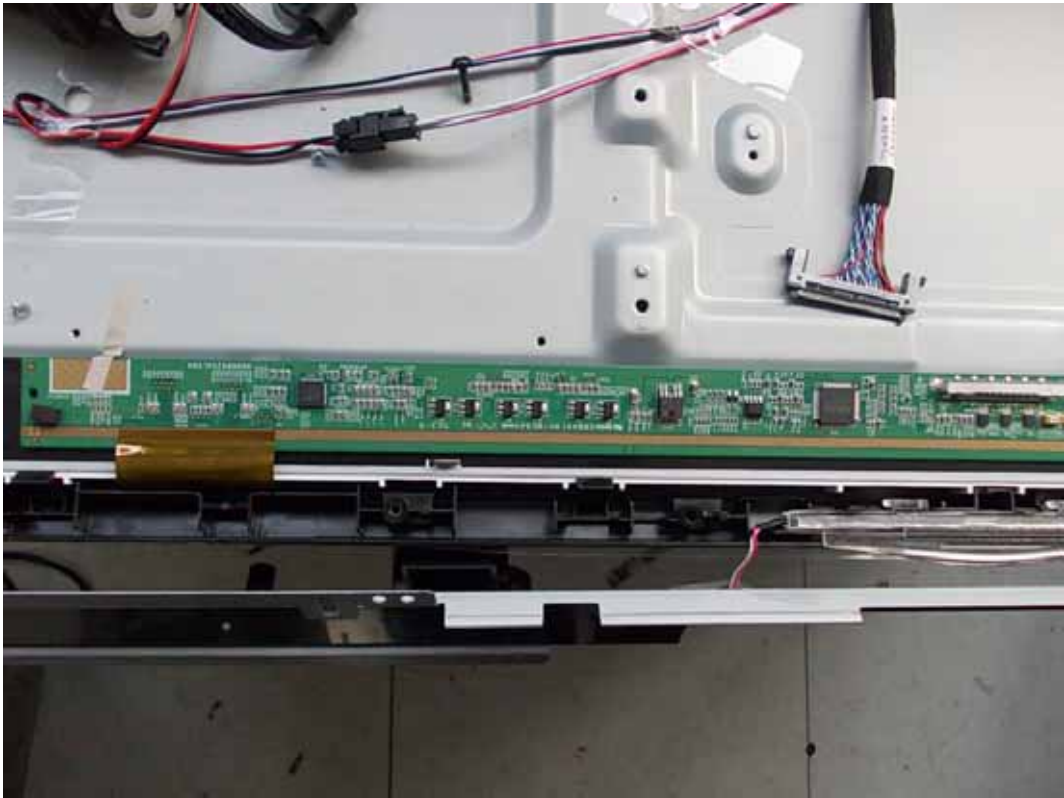
FIGURE 12 LED LCD TV (M/N: LTDN40K360MUS) LCD PANEL BOARD (COMPONENT SIDE #2)
