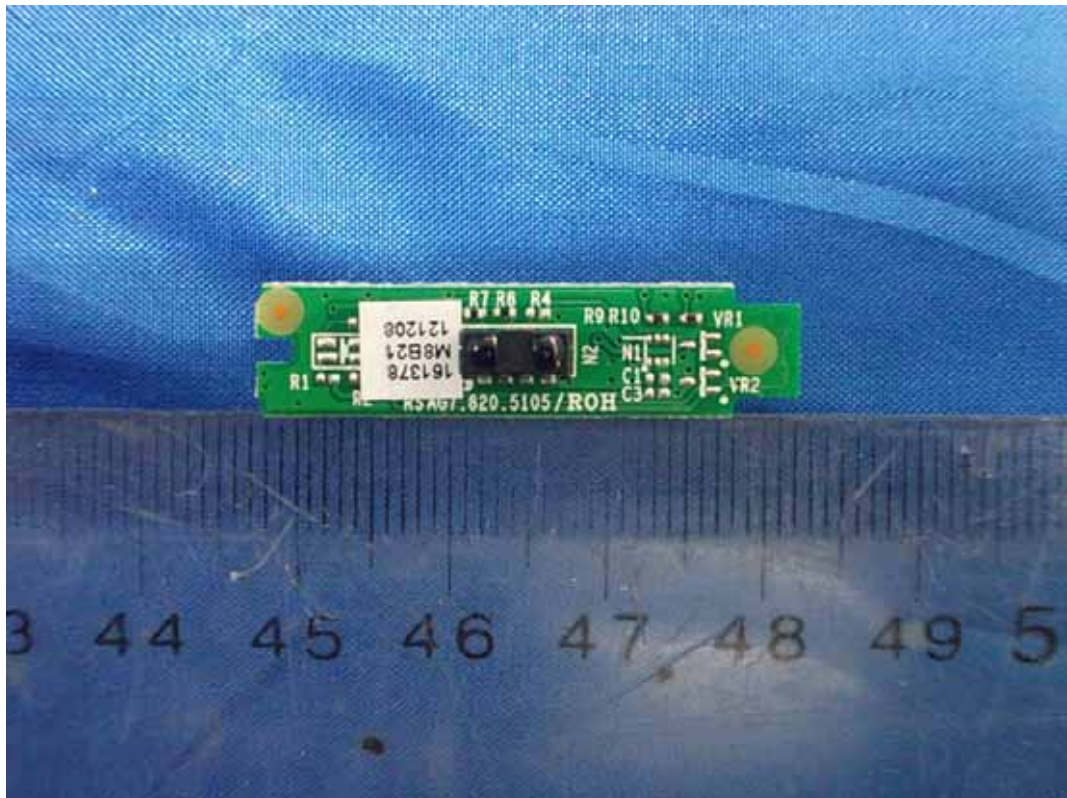
FIGURE 17 LED LCD TV (M/N: LTDN40K360MUS) IR BOARD (COMPONENT SIDE)
