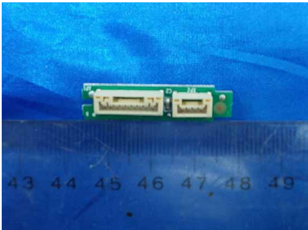
FIGURE 18 LED LCD TV (M/N: LTDN40K360MUS) IR BOARD (SOLDERED SIDE)
