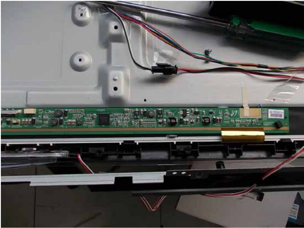
FIGURE 11 LED LCD TV (M/N: LTDN40K360MUS) LCD PANEL BOARD (COMPONENT SIDE #1)
