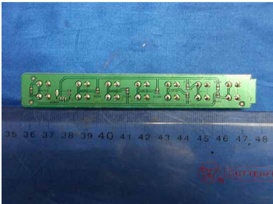
FIGURE 16 LED LCD TV (M/N: LTDN40K360MUS) KEY BOARD (SOLDERED SIDE)
