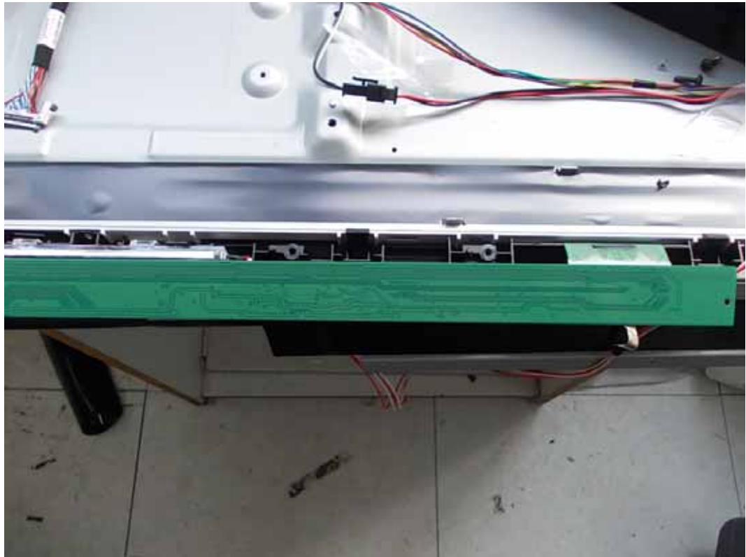
FIGURE 13 LED LCD TV (M/N: LTDN40K360MUS) LCD PANEL BOARD (SOLDERED SIDE #1)
