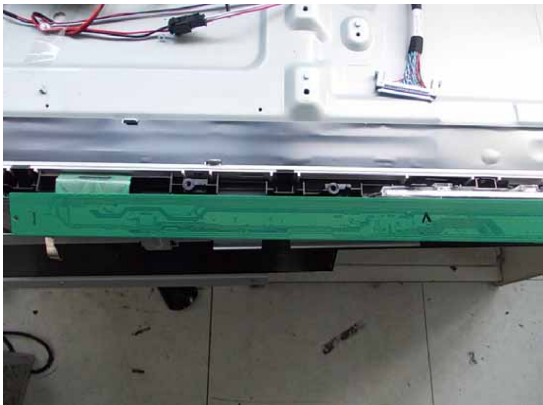
FIGURE 14 LED LCD TV (M/N: LTDN40K360MUS) LCD PANEL BOARD (SOLDERED SIDE #2)
