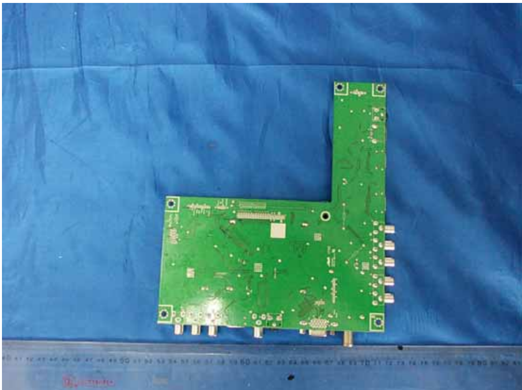
FIGURE 5 LED LCD TV (M/N: LTDN40K360US) MAIN BOARD (SOLDERED SIDE)
