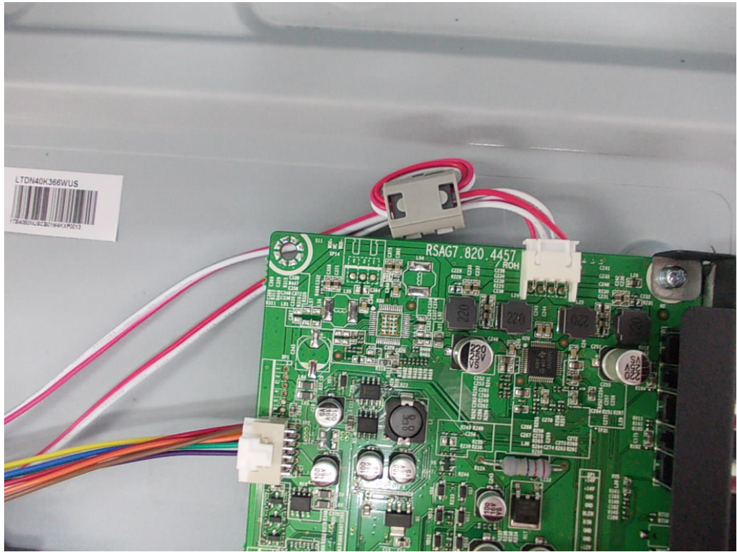
FIGURE 16 LED LCD TV (M/N: LTDN40K366WUS) DEBUG 1
