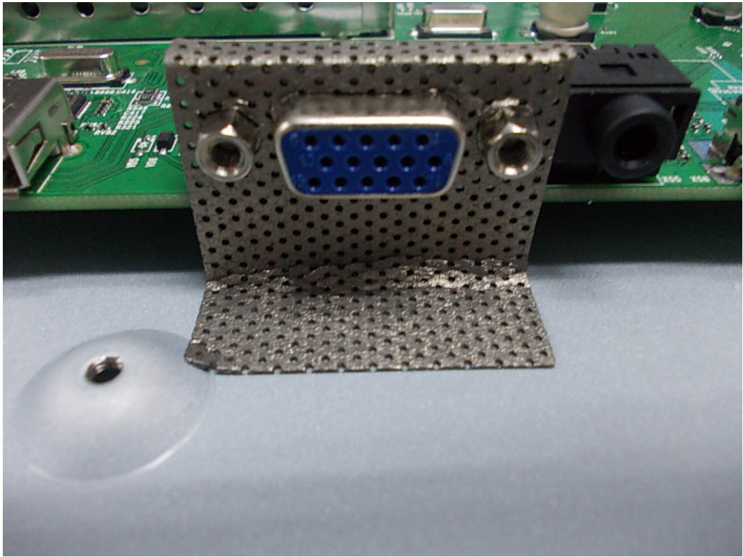
FIGURE 18 LED LCD TV (M/N: LTDN40K366WUS) DEBUG 3
