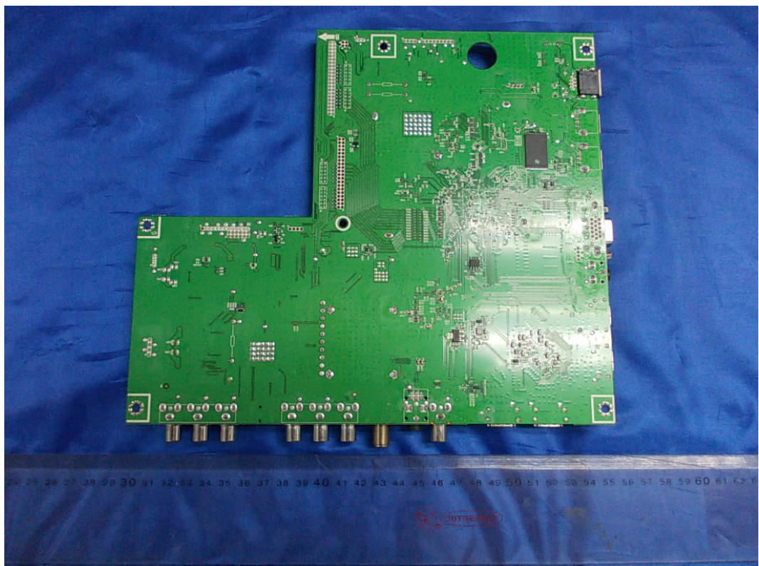
FIGURE 6 LED LCD TV (M/N: LTDN40K366WUS) MAIN BOARD (SOLDERED SIDE)
