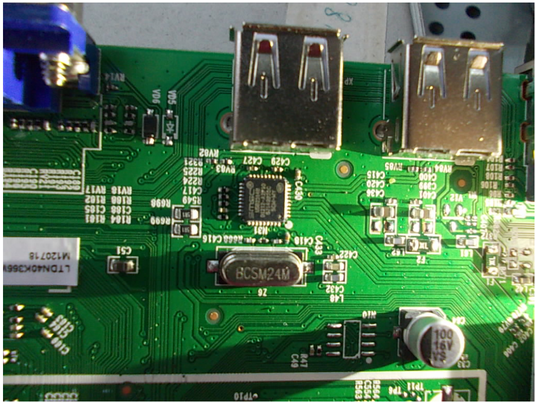
FIGURE 11 LED LCD TV (M/N: LTDN40K366WUS) CRYSTAL #3 ON MAIN BOARD
