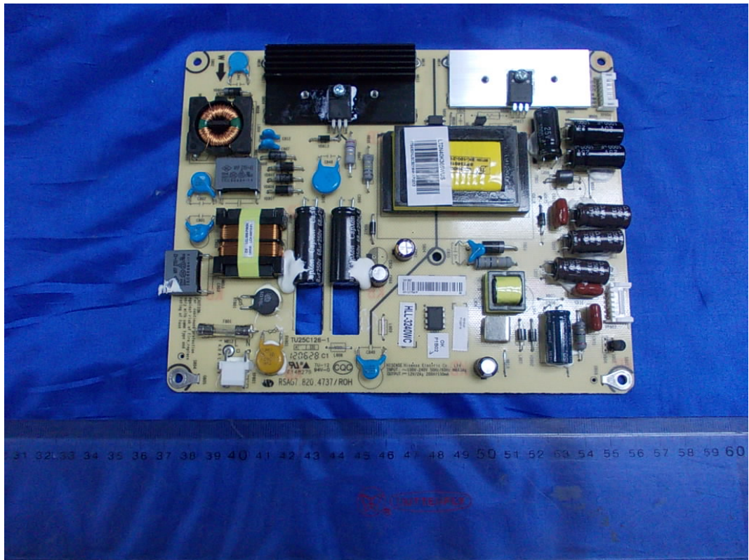
FIGURE 3 LED LCD TV (M/N: LTDN40K366WUS) POWER BOARD (COMPONENT SIDE)
