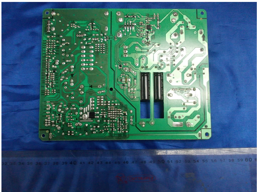
FIGURE 4 LED LCD TV (M/N: LTDN40K366WUS) POWER BOARD (SOLDERED SIDE)
