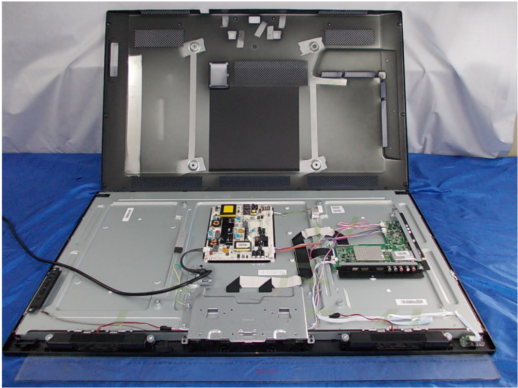
FIGURE 1 LED LCD TV (M/N: LTDN42K20US) COVER REMOVED
