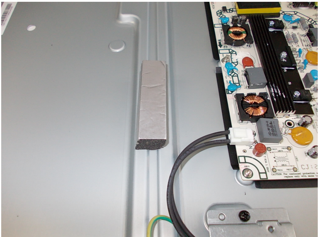
FIGURE 17 LED LCD TV (M/N: LTDN42K20US) DEBUG 2
