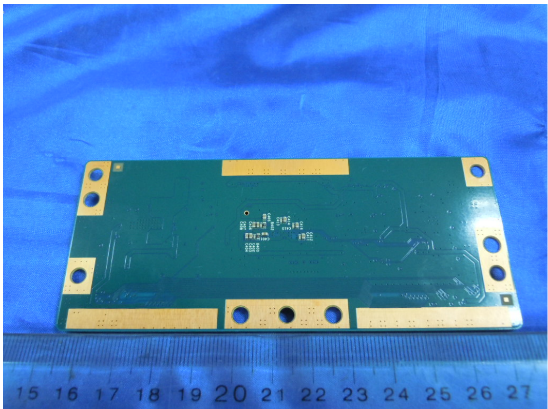
FIGURE 15 LED LCD TV (M/N: LTDN42K20US) PANEL BOARD (SOLDERED SIDE)
