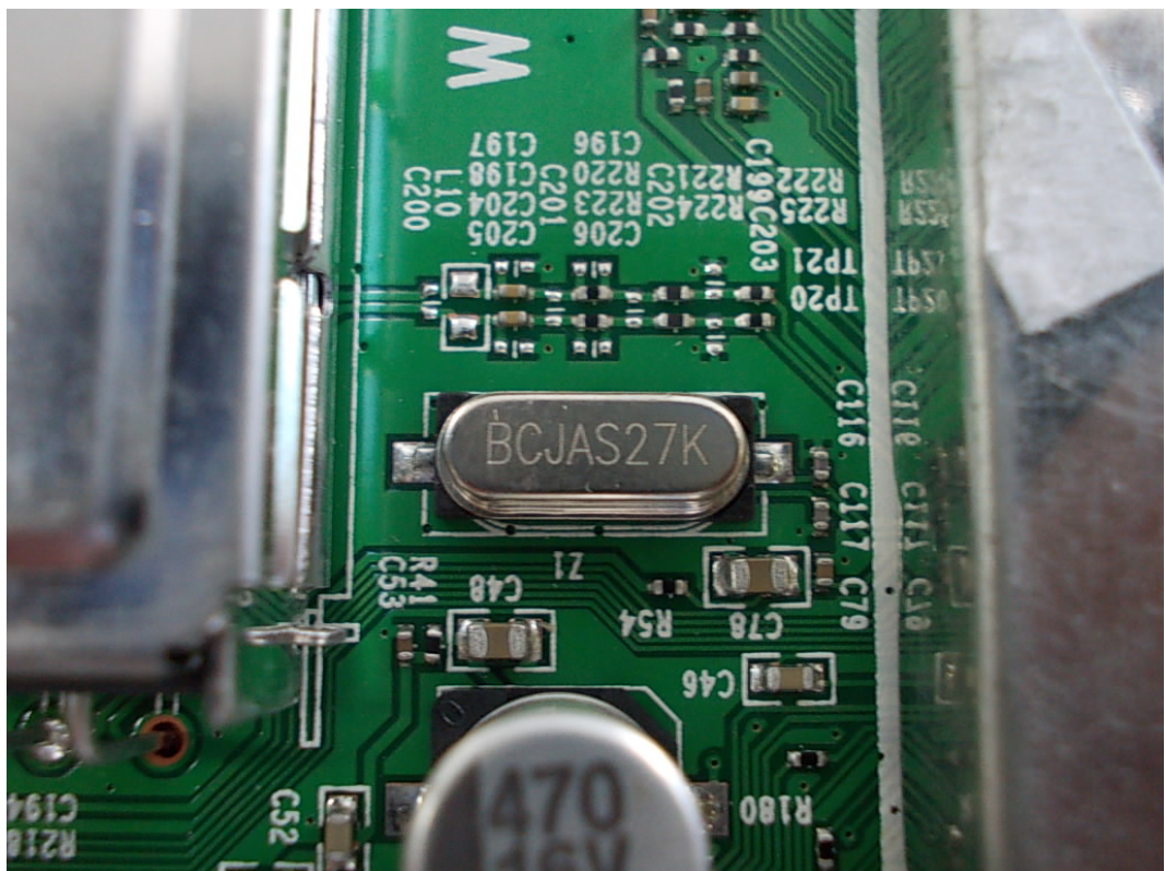
FIGURE 8 LED LCD TV (M/N: LTDN42K20US) CRYSTAL ON MAIN BOARD
