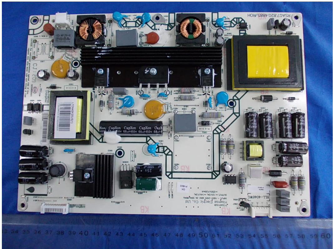
FIGURE 3 LED LCD TV (M/N: LTDN42K20US) POWER BOARD (COMPONENT SIDE)
