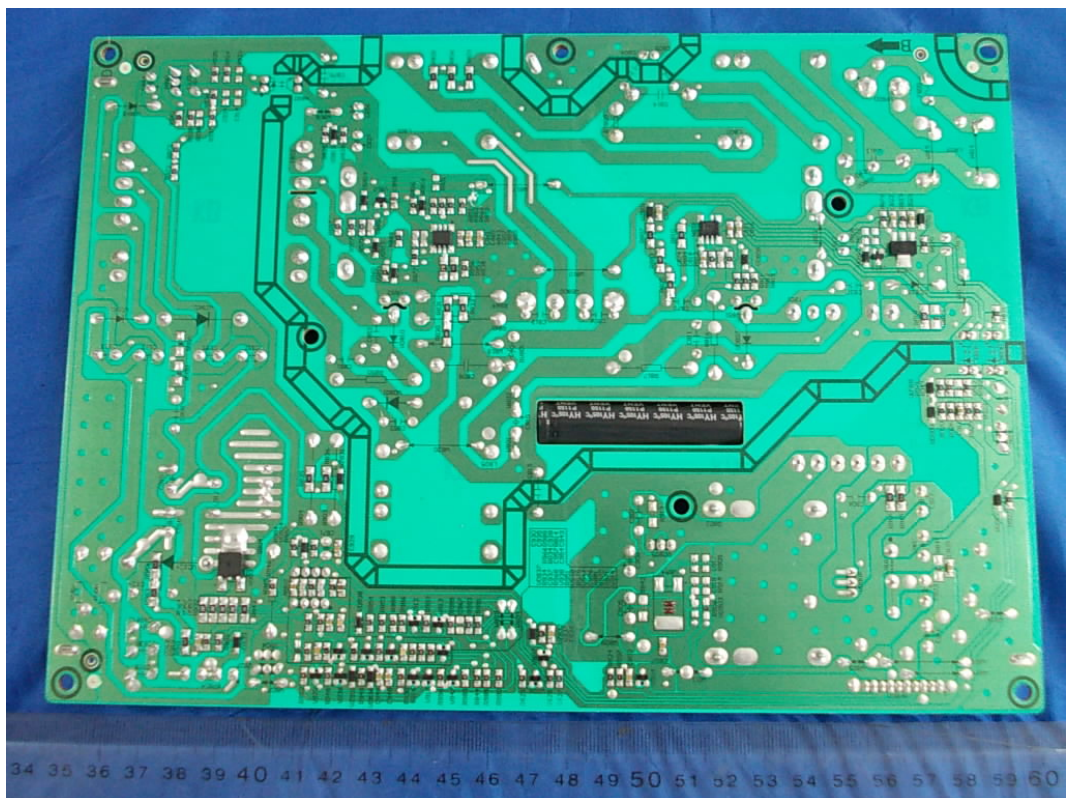
FIGURE 4 LED LCD TV (M/N: LTDN42K20US) POWER BOARD (SOLDERED SIDE)
