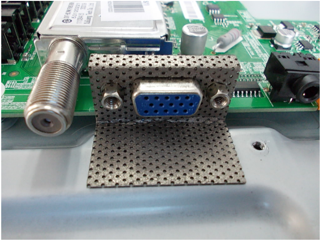
FIGURE 18 LED LCD TV (M/N: LTDN42K20US) DEBUG 3
