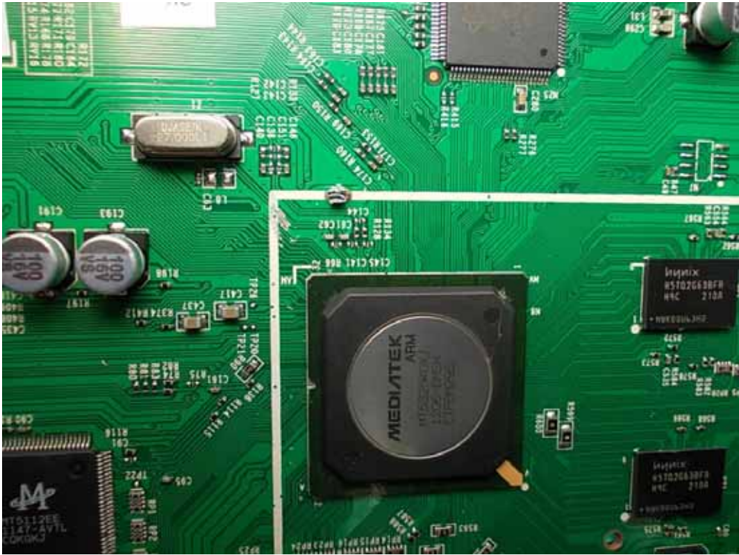
FIGURE 8 LED LCD TV (M/N: LTDN42D77WUS) CHIP#2 & CRYSTAL#2 ON MAIN BOARD
