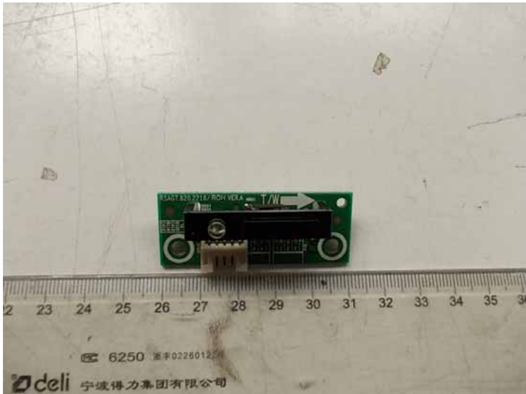
FIGURE 12 LED LCD TV (M/N: LTDN42D77WUS) IR BOARD (COMPONENT SIDE)
