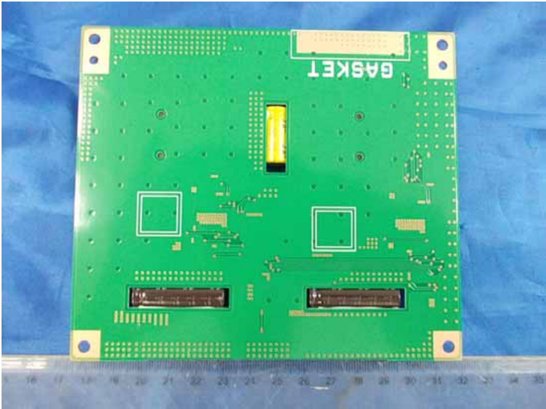
FIGURE 17 LED LCD TV (M/N: LTDN42D77WUS) HIGH VOLTAGE SIGNAL BOARD (SOLDERED SIDE)
