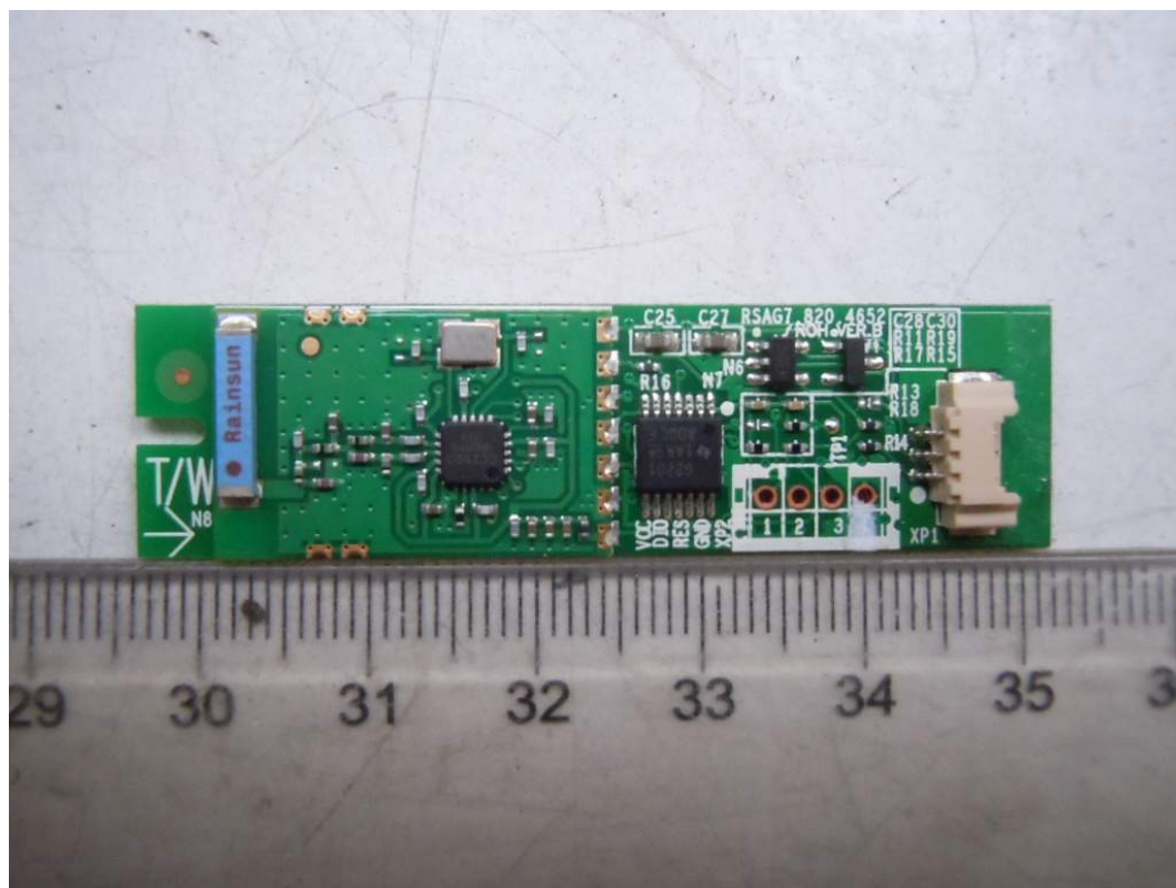
FIGURE 14 LED LCD TV (M/N: LTDN42K316XWUS3D) RF BOARD (COMPONENT SIDE)
