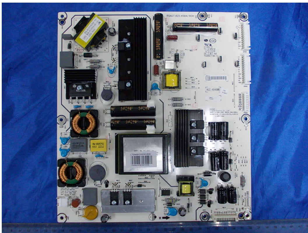
FIGURE 3 LED LCD TV (M/N: LTDN42K316XWUS3D) POWER BOARD (COMPONENT SIDE)
