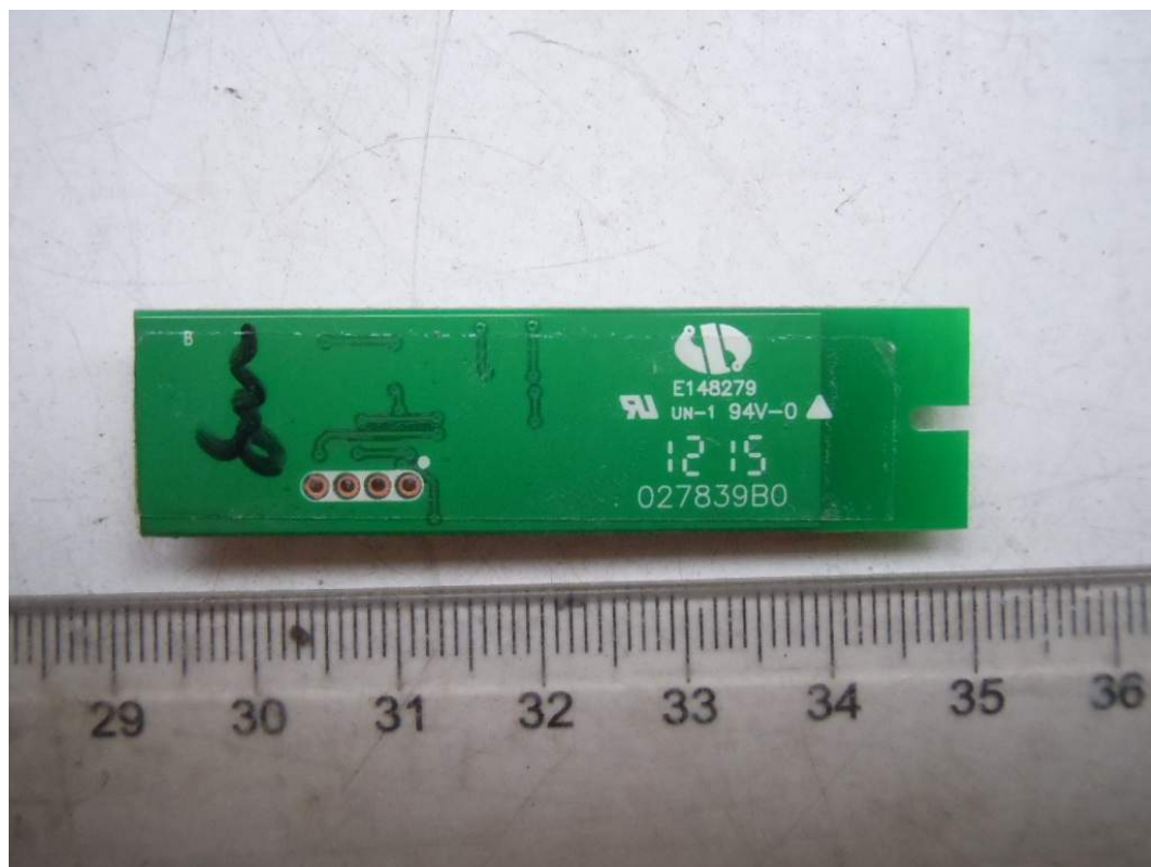
FIGURE 15 LED LCD TV (M/N: LTDN42K316XWUS3D) RF BOARD (SOLDERED SIDE)
