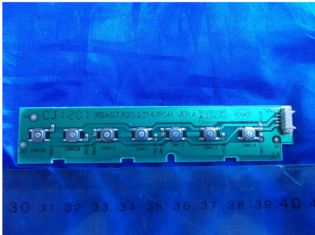
FIGURE 10 LED LCD TV (M/N: LTDN42K316XWUS3D) KEY BOARD (COMPONENT SIDE)
