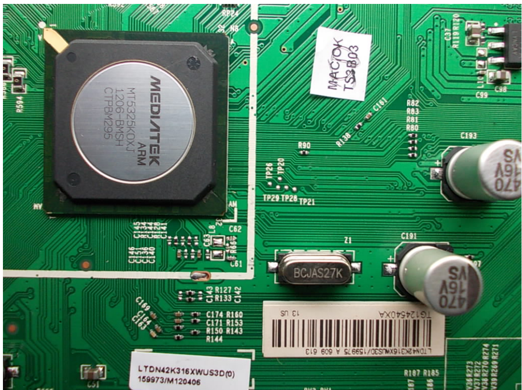
FIGURE 8 LED LCD TV (M/N: LTDN42K316XWUS3D) CHIP ON MAIN BOARD
