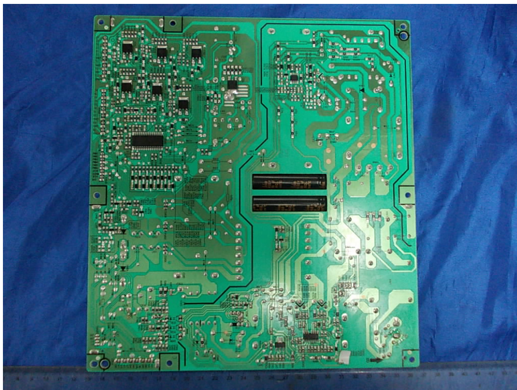
FIGURE 4 LED LCD TV (M/N: LTDN42K316XWUS3D) POWER BOARD (SOLDERED SIDE)
