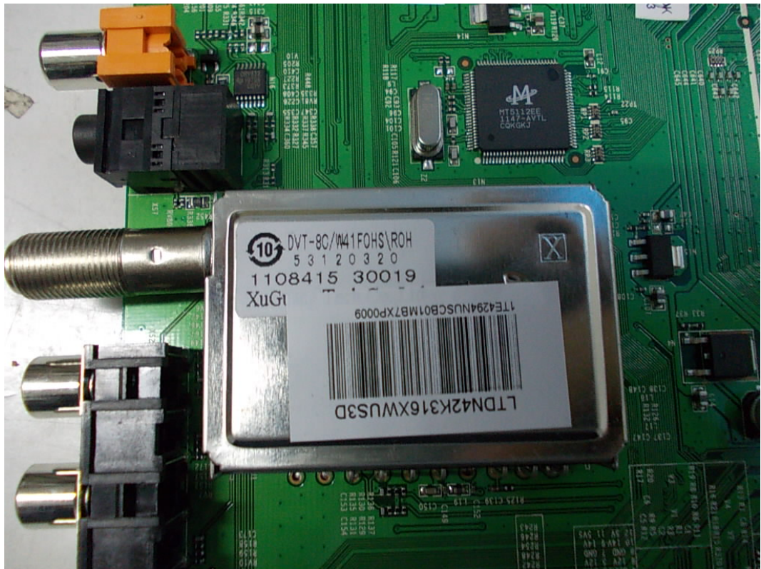
FIGURE 7 LED LCD TV (M/N: LTDN42K316XWUS3D) TUNER ON MAIN BOARD
