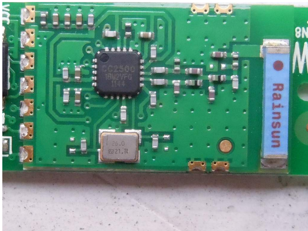
FIGURE 16 LED LCD TV (M/N: LTDN42K316XWUS3D) CHIP & CRYSTAL ON RF BOARD
