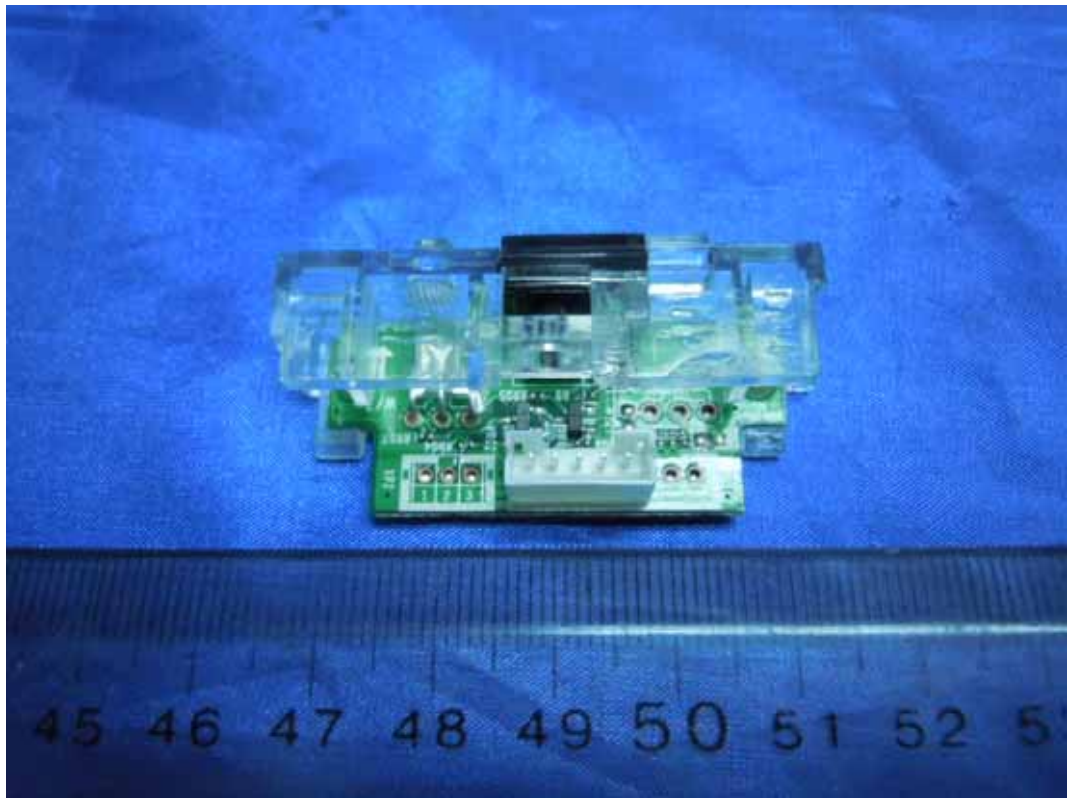
FIGURE 11 LED LCD TV (M/N: LTDN42K20US) IR BOARD (COMPONENT SIDE)
