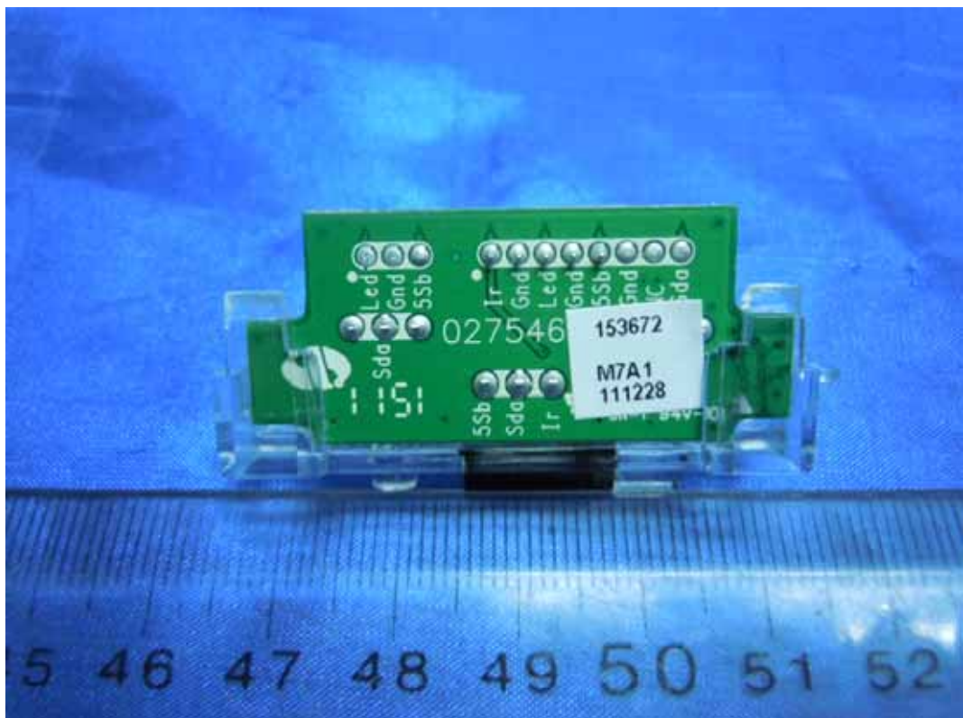
FIGURE 12 LED LCD TV (M/N: LTDN42K20US) IR BOARD (SOLDERED SIDE)
