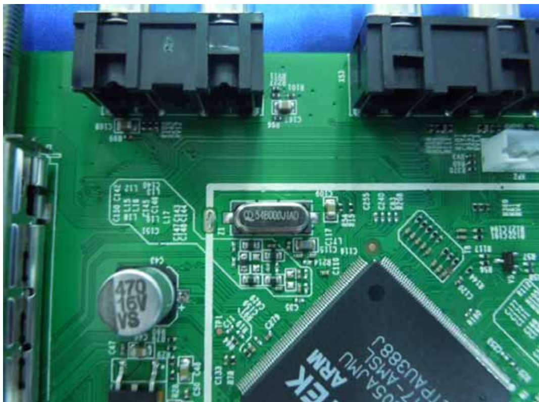
FIGURE 7 LED LCD TV (M/N: LTDN42K20US) CRYSTAL ON MAIN BOARD
