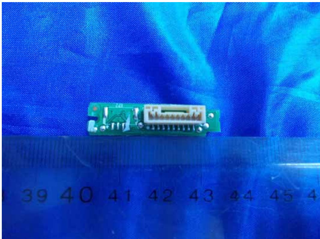
FIGURE 11 LCD TV (M/N: LTDN39V77US) IR BOARD (SOLDERED SIDE)
