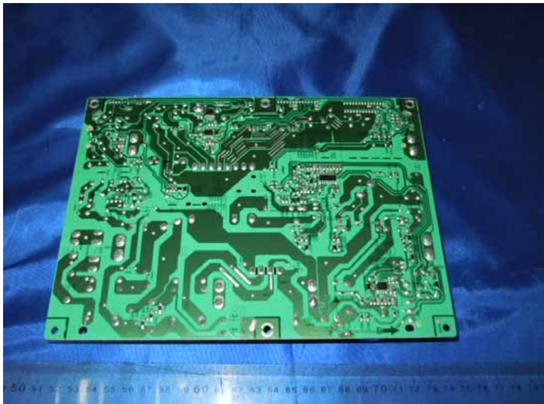
FIGURE 4 LCD TV (M/N: LTDN40V87HUS) POWER BOARD (SOLDERED SIDE)
