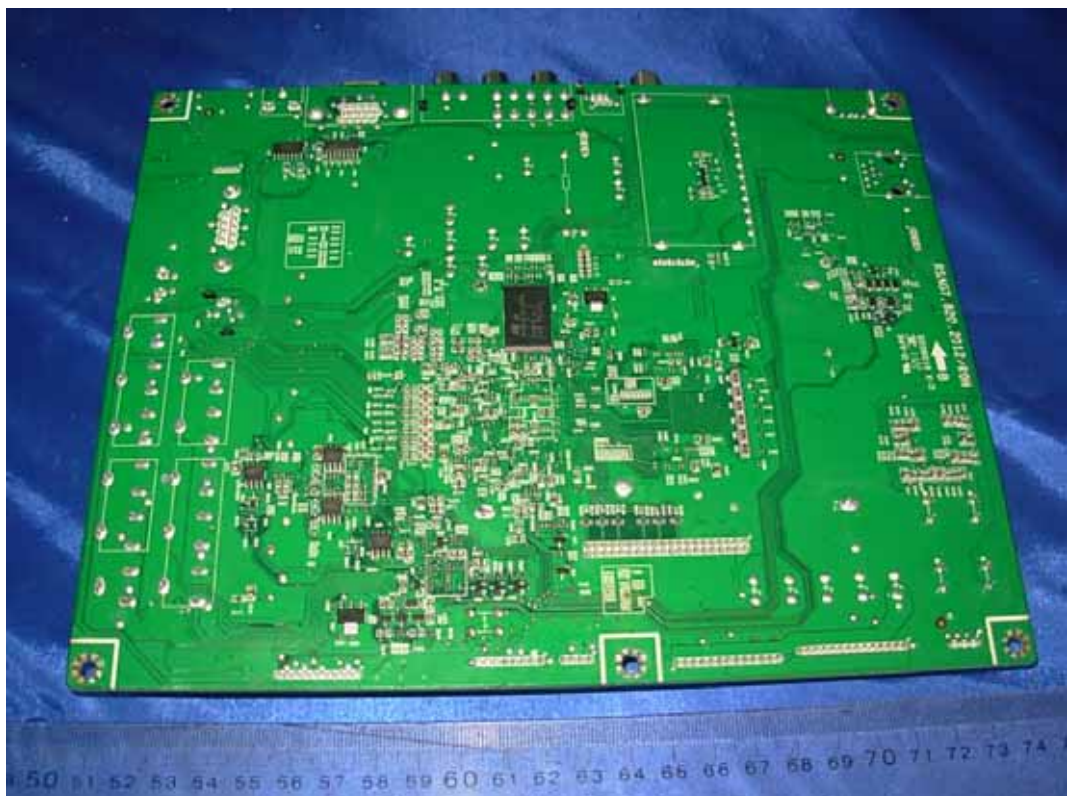
FIGURE 5 LCD TV (M/N: LTDN42V77MH) MAIN BOARD (SOLDERED SIDE)
