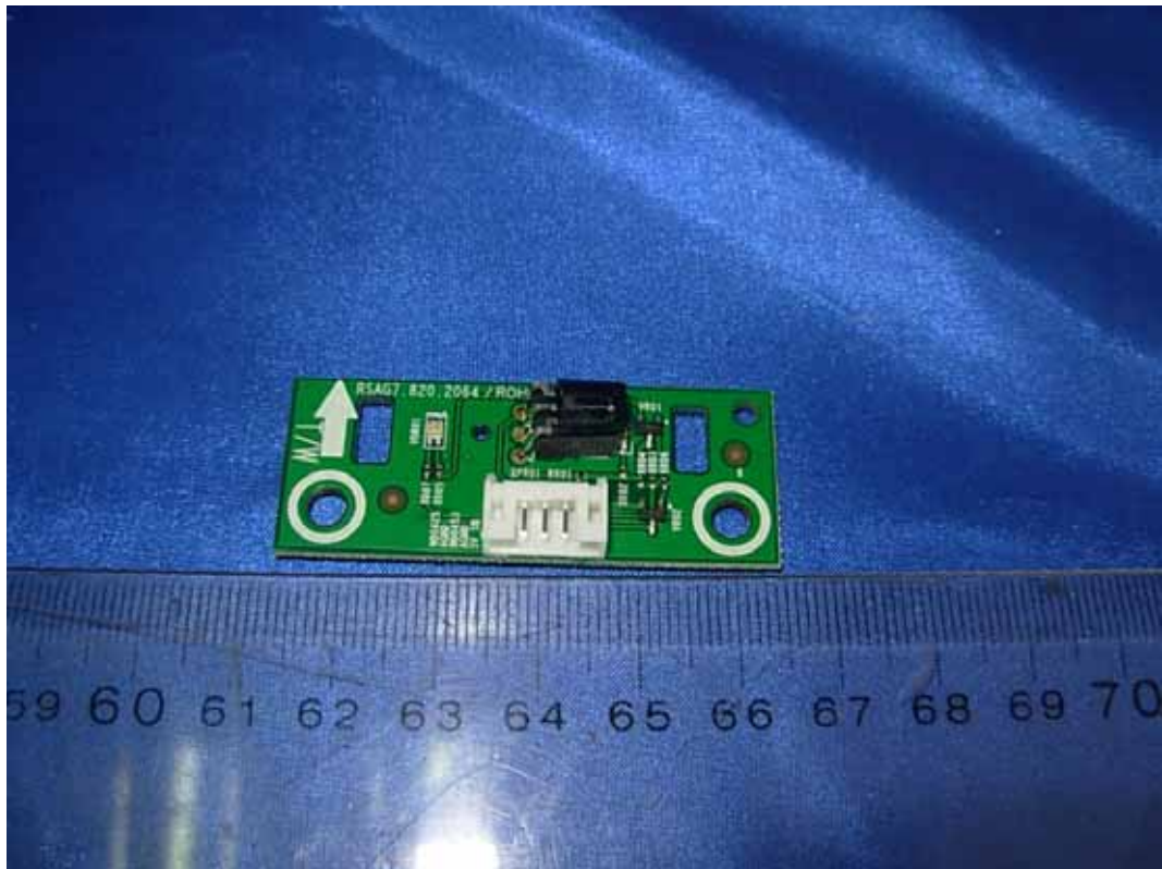
FIGURE 14 LCD TV (M/N: LTDN42V77MH) IR BOARD (COMPONENT SIDE)
