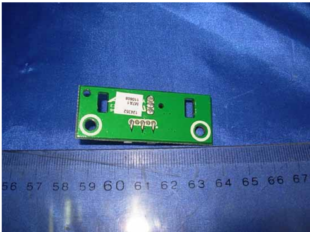
FIGURE 15 LCD TV (M/N: LTDN42V77MH) IR BOARD (SOLDERED SIDE)
