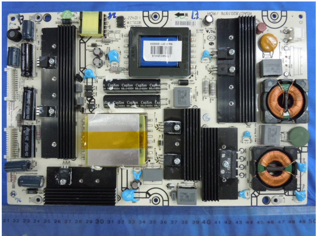
FIGURE 3 LED LCD TV (M/N: LTDN40K26WUS) POWER BOARD (COMPONENT SIDE)
