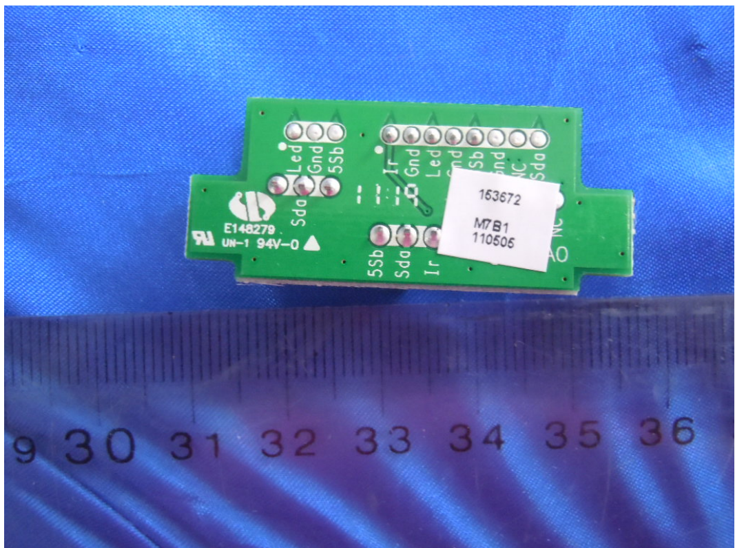
FIGURE 13 LED LCD TV (M/N: LTDN40K26WUS) IR BOARD (SOLDERED SIDE)
