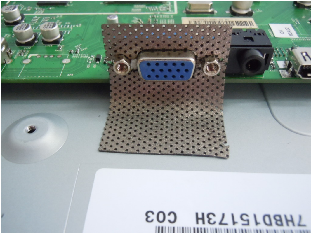
FIGURE 16 LED LCD TV (M/N: LTDN40K26WUS) DEBUG 1
