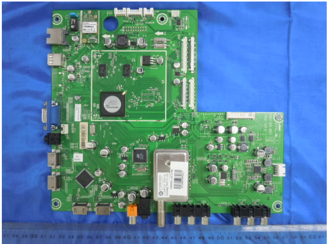
FIGURE 5 LED LCD TV (M/N: LTDN40K26WUS) MAIN BOARD (COMPONENT SIDE)
