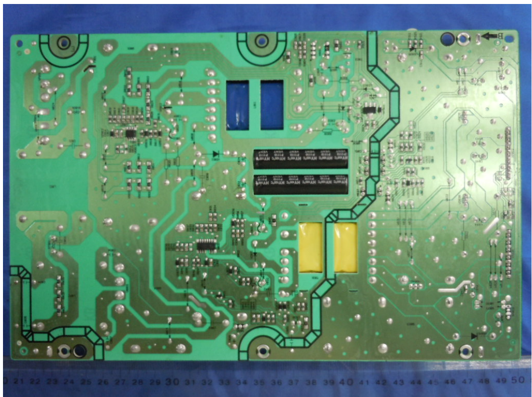
FIGURE 4 LED LCD TV (M/N: LTDN40K26WUS) POWER BOARD (SOLDERED SIDE)
