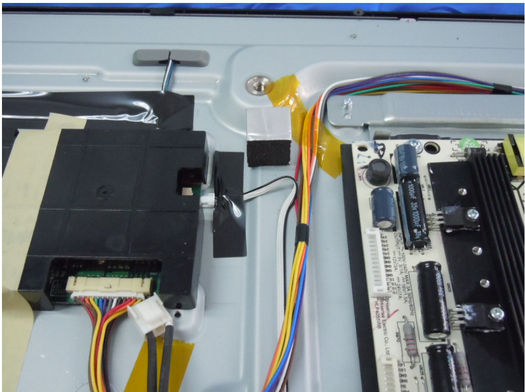
FIGURE 17 LED LCD TV (M/N: LTDN40K26WUS) DEBUG 2
