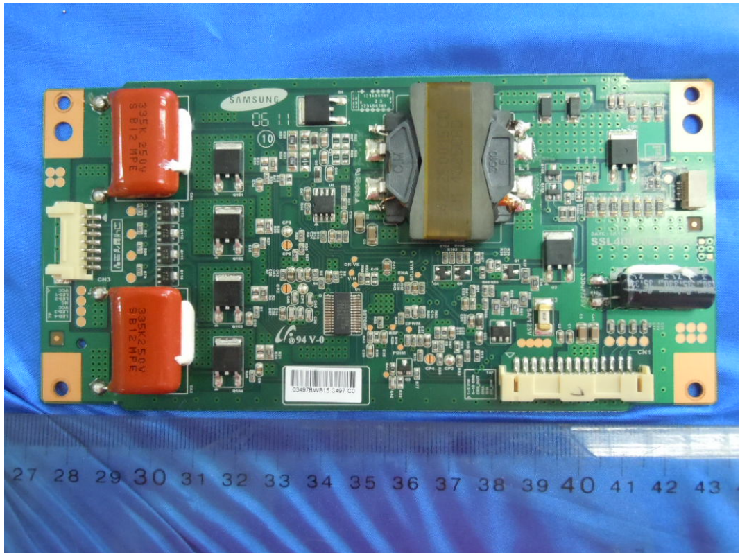
FIGURE 14 LED LCD TV (M/N: LTDN40K26WUS) HIGH VOLTAGE SIGNAL BOARD (COMPONENT SIDE)
