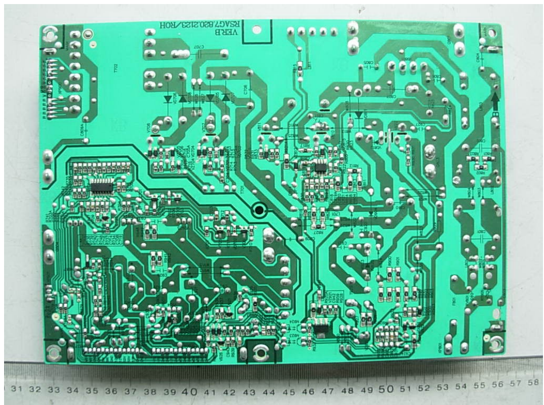
FIGURE 4 LCD TV (M/N: LCD42V68PCA) POWER BOARD (SOLDERED SIDE)
