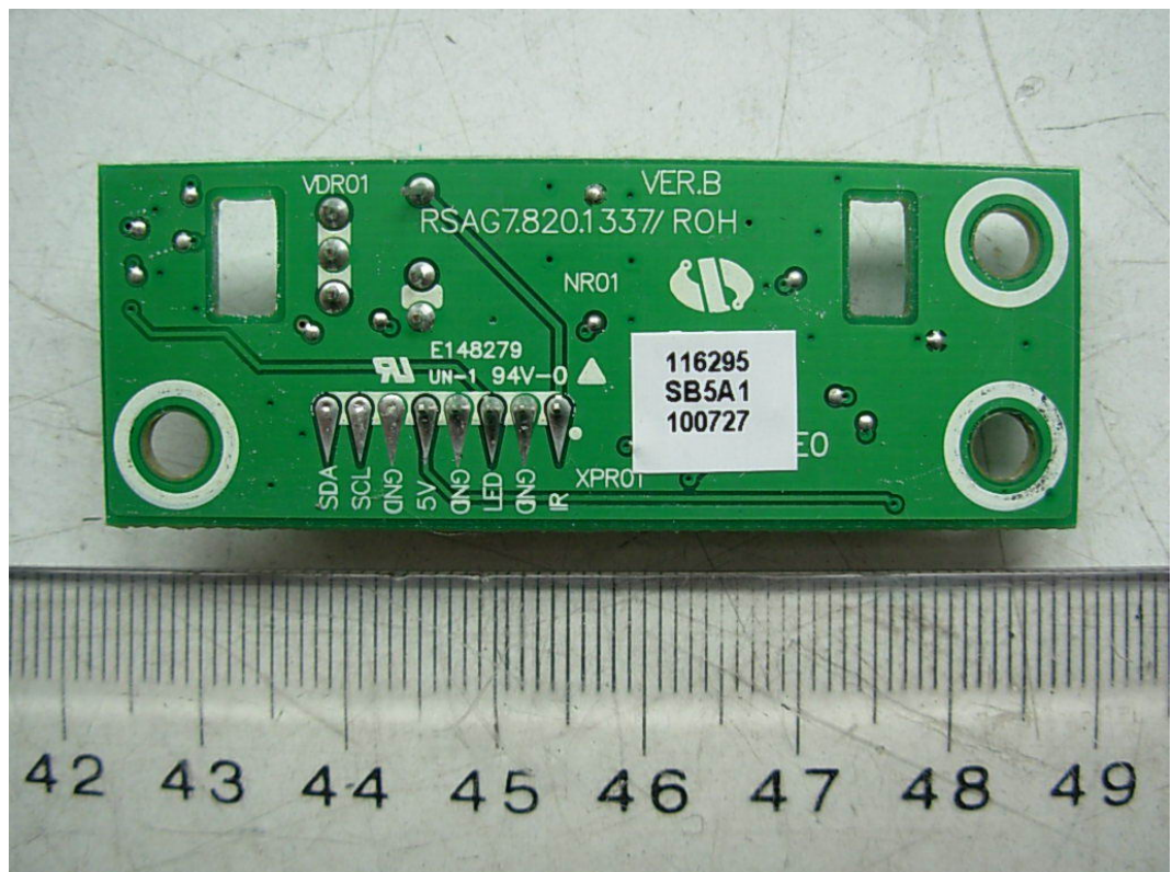
FIGURE 11 LCD TV (M/N: LCD42V68PCA) IR BOARD (SOLDERED SIDE)
