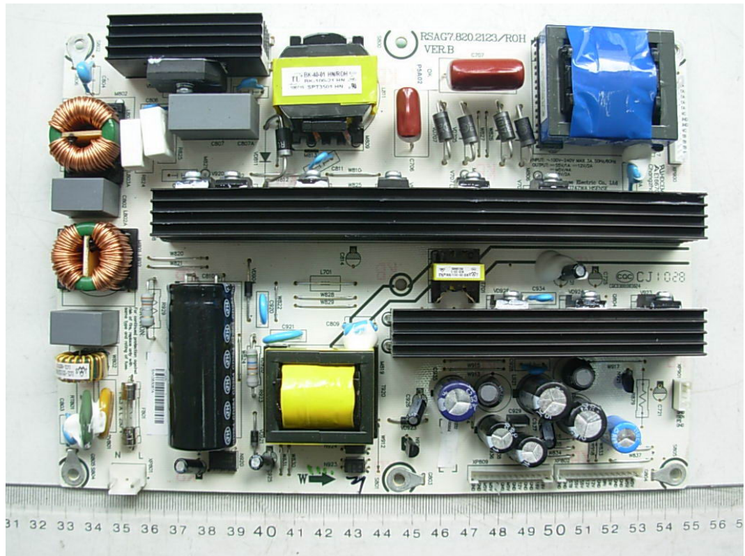
FIGURE 3 LCD TV (M/N: LCD42V68PCA) POWER BOARD (COMPONENT SIDE)
