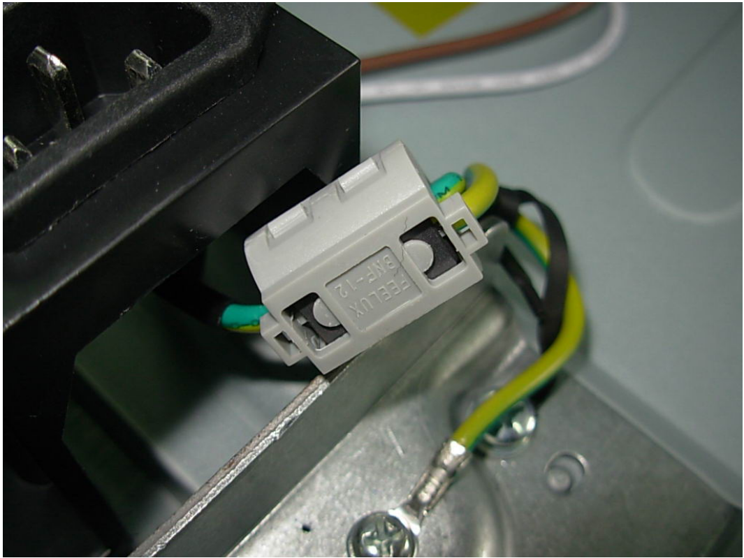
FIGURE 20 LCD TV (M/N: LCD42V68PCA) DEBUG 3
