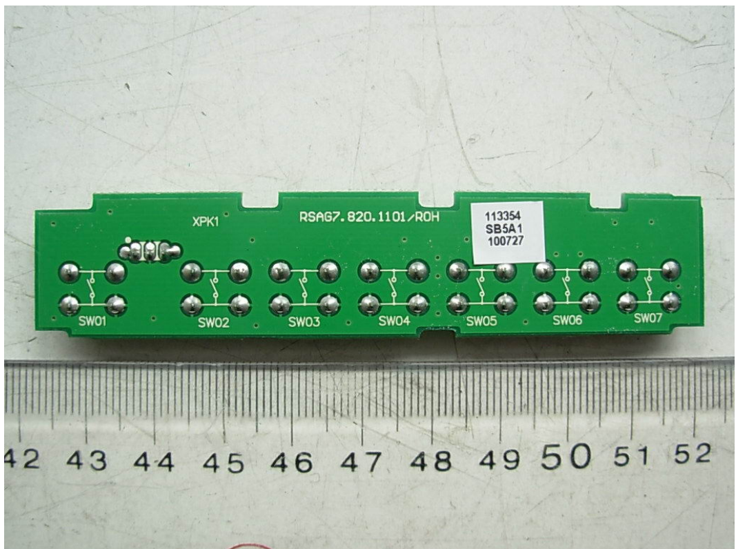
FIGURE 15 LCD TV (M/N: LCD42V68PCA) BOTTON BOARD (SOLDERED SIDE)
