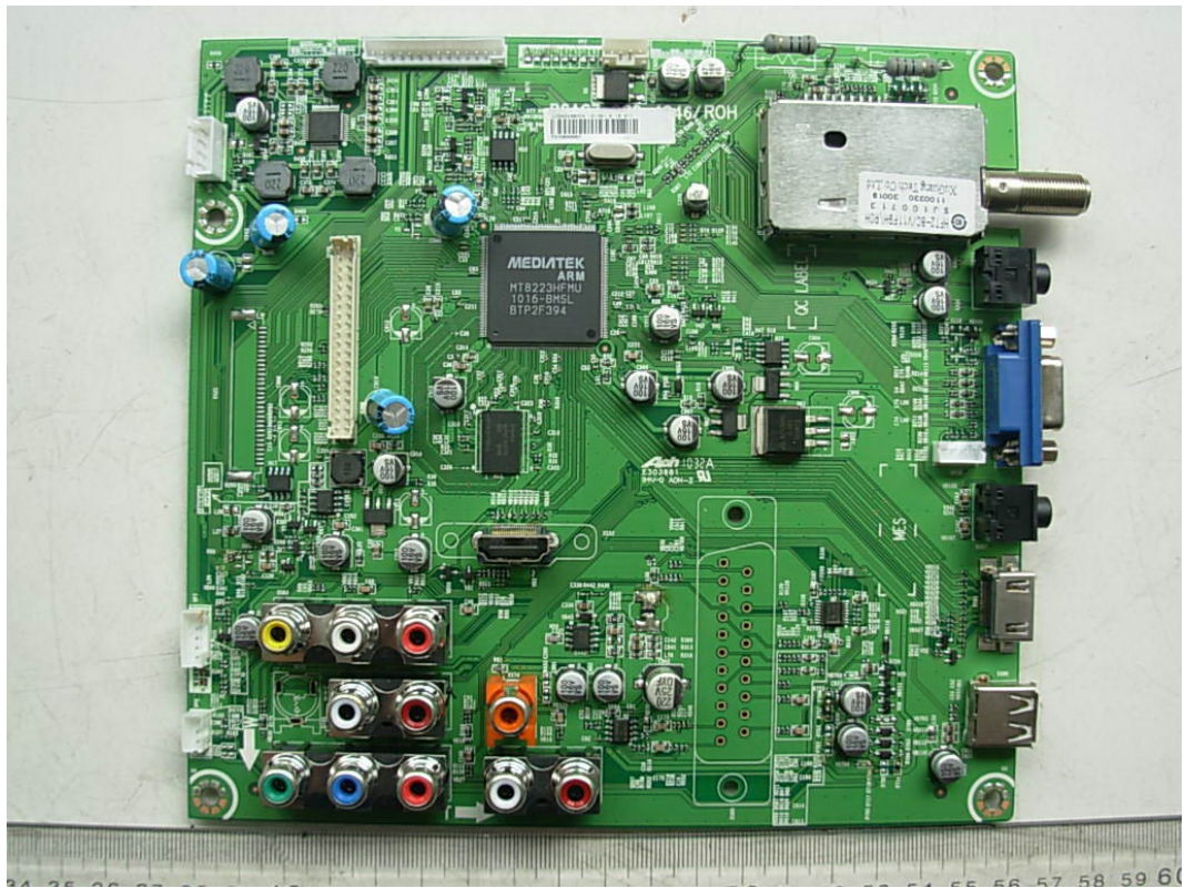
FIGURE 5 LCD TV (M/N: LCD42V68PCA) MAIN BOARD (COMPONENT SIDE)
