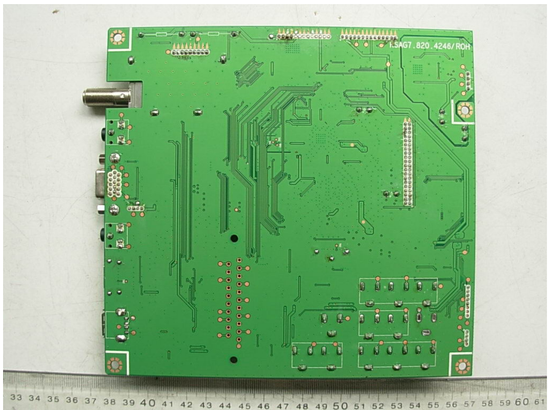
FIGURE 6 LCD TV (M/N: LCD42V68PCA) MAIN BOARD (SOLDERED SIDE)
