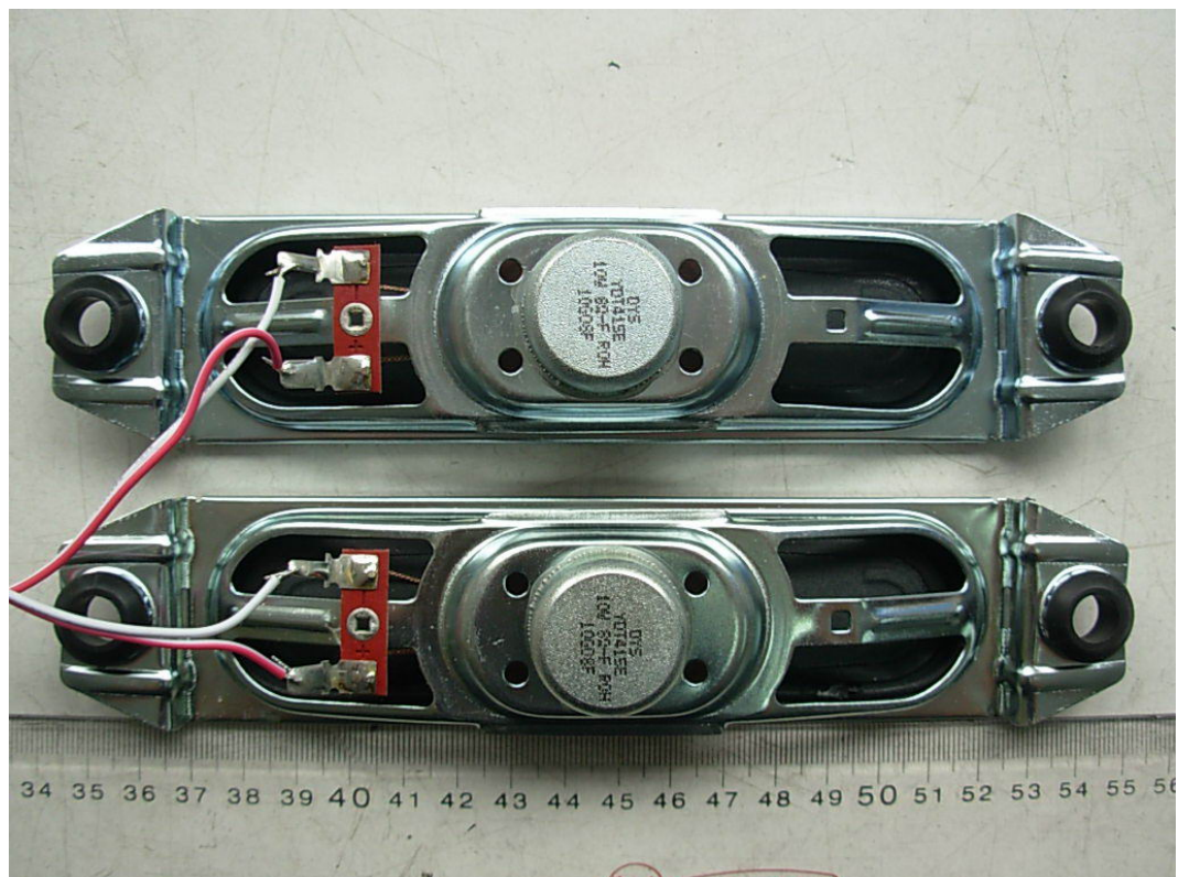
FIGURE 17 LCD TV (M/N: LCD42V68PCA) SPEAKER (BACK VIEW)
