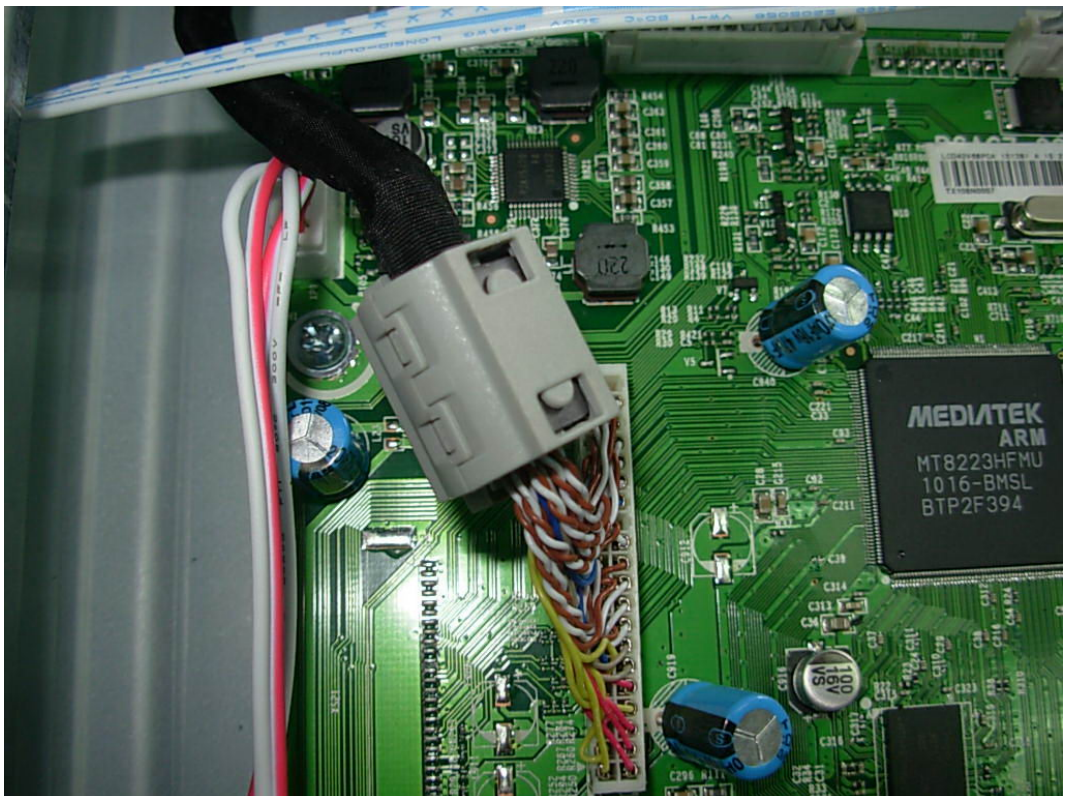
FIGURE 19 LCD TV (M/N: LCD42V68PCA) DEBUG 2
