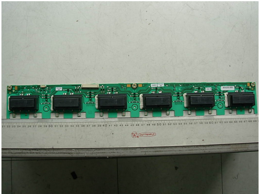
FIGURE 12 LCD TV (M/N: LCD42V68PCA) INVERTER BOARD (COMPONENT SIDE)
