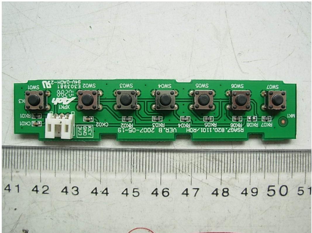
FIGURE 14 LCD TV (M/N: LCD42V68PCA) BOTTON BOARD (COMPONENT SIDE)
