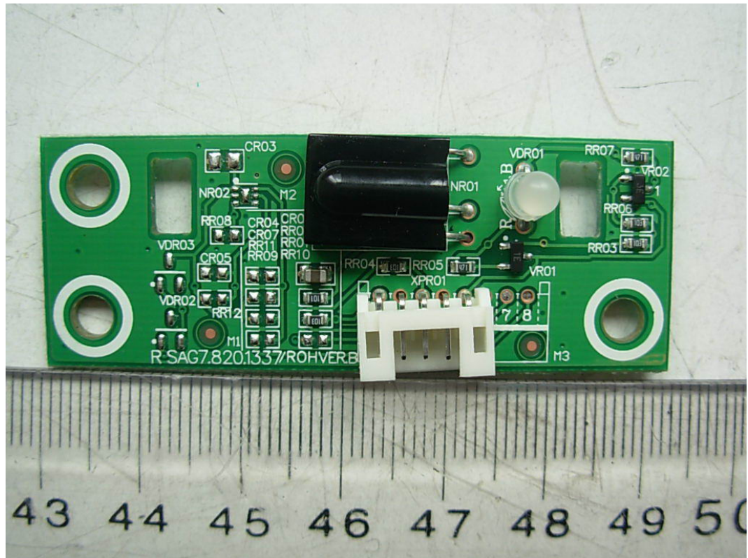
FIGURE 10 LCD TV (M/N: LCD42V68PCA) IR BOARD (COMPONENT SIDE)
