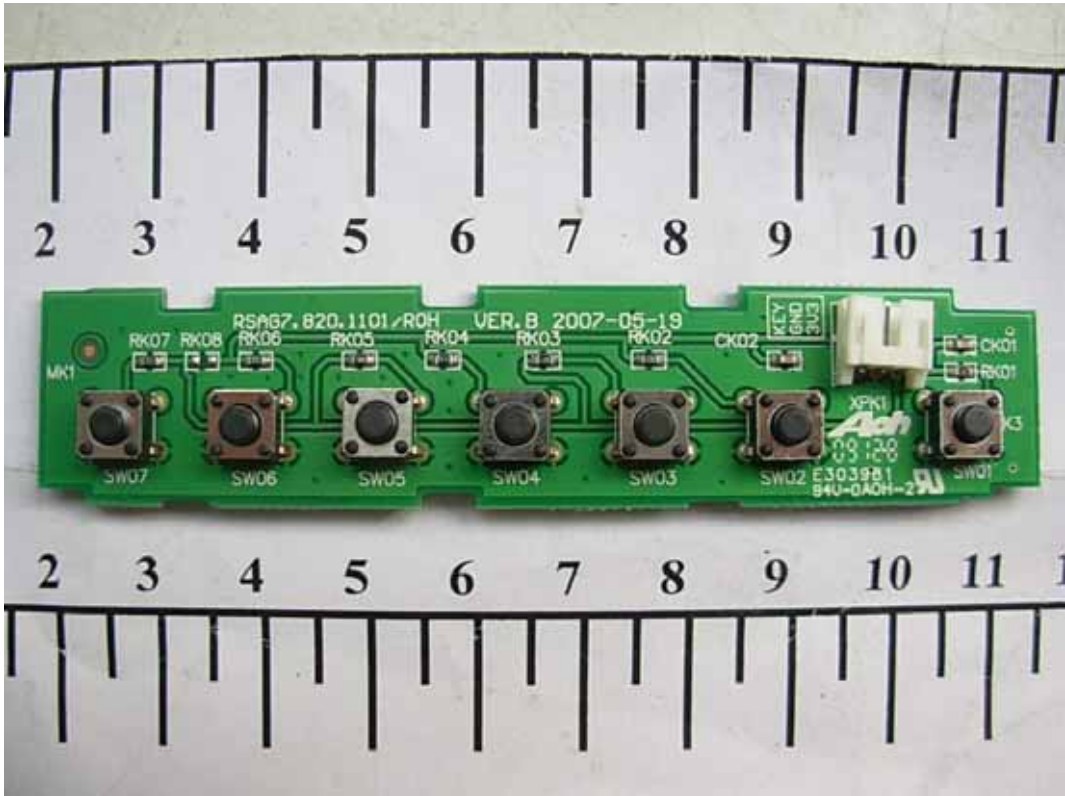
FIGURE 10 LCD TV (M/N: LTDN42W58US) KEY BOARD (COMPONENT SIDE)
