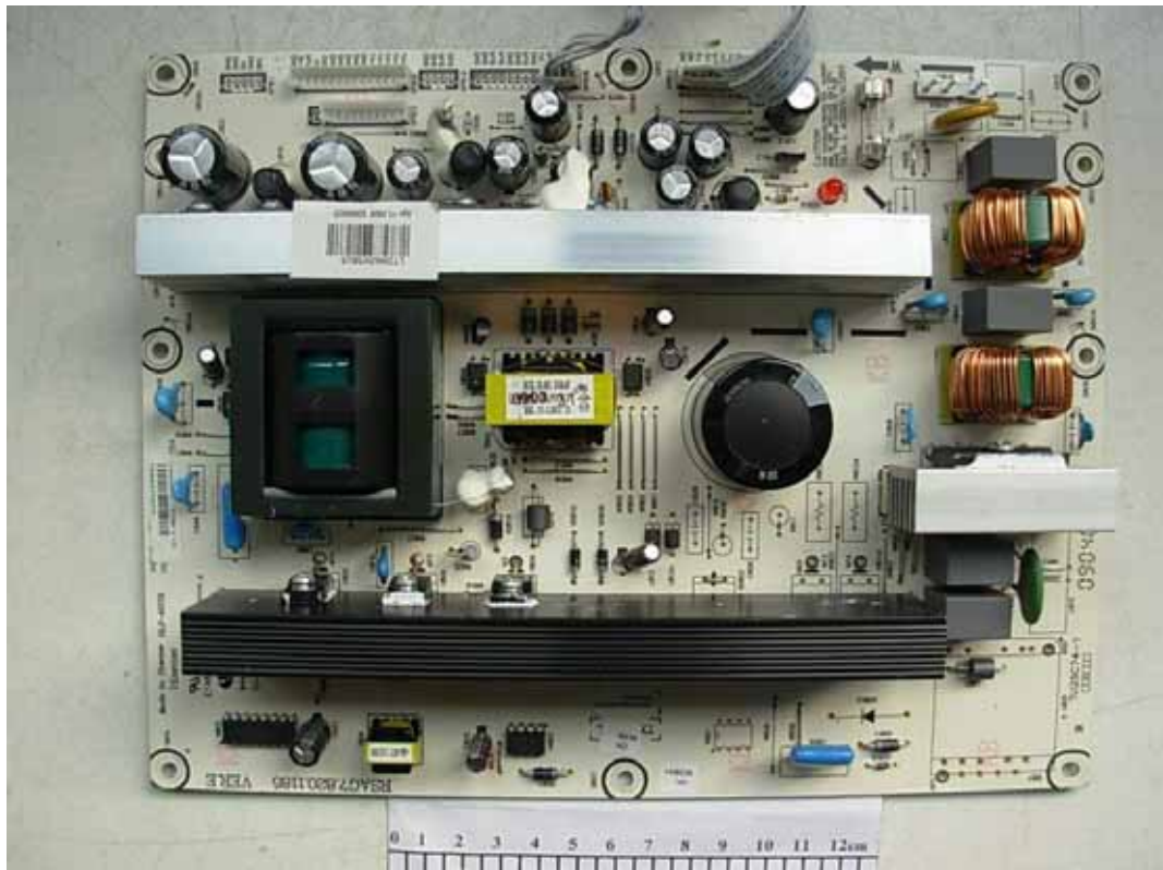
FIGURE 6 LCD TV (M/N: LTDN42W58US) POWER BOARD (COMPONENT SIDE)
