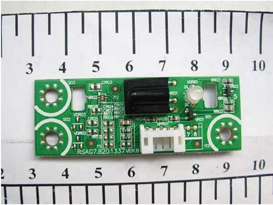
FIGURE 8 LCD TV (M/N: LTDN42W58US) IR BOARD (COMPONENT SIDE)
