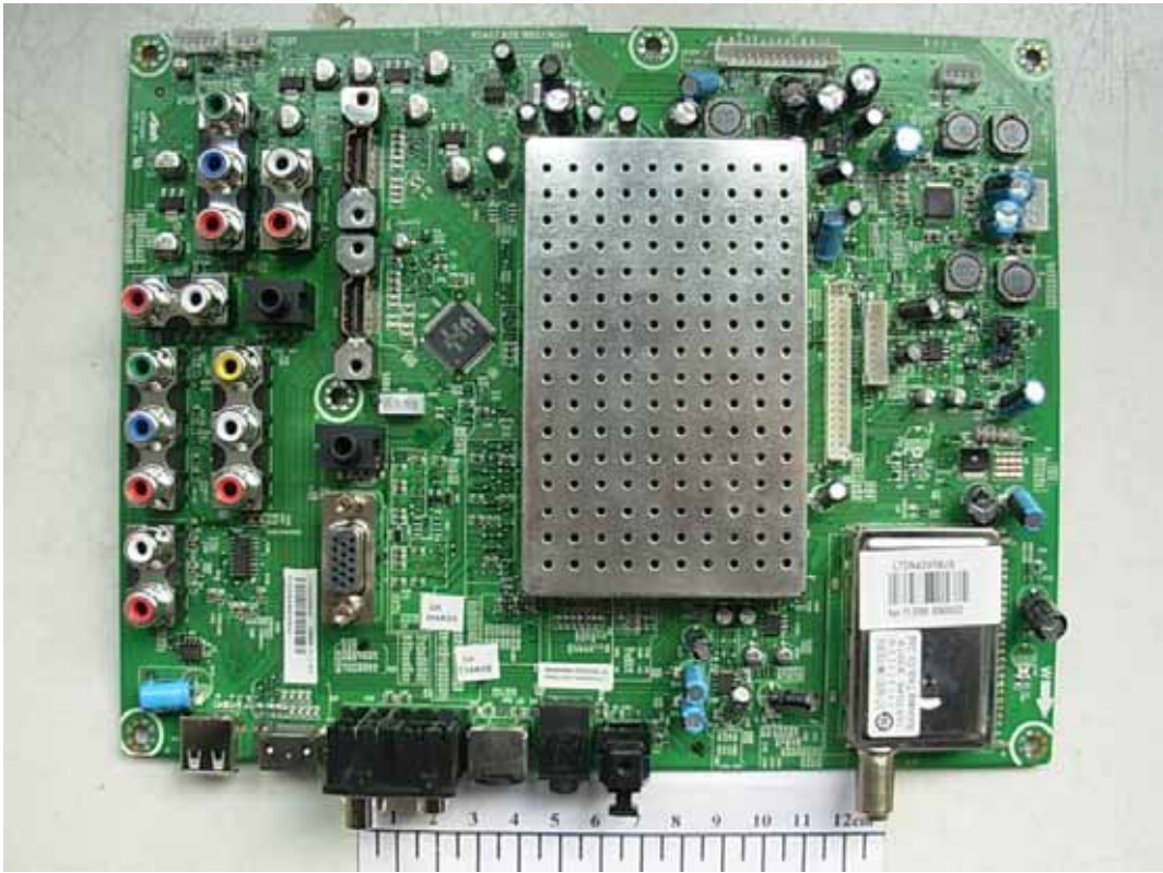
FIGURE 2 LCD TV (M/N: LTDN46T28GUS) MAIN BOARD (COMPONENT SIDE)
