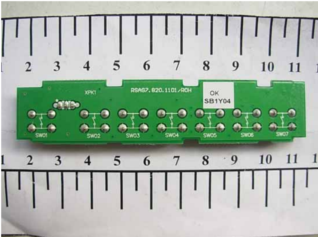
FIGURE 11 LCD TV (M/N: LTDN42W58US) KEY BOARD (SOLDERED SIDE)
