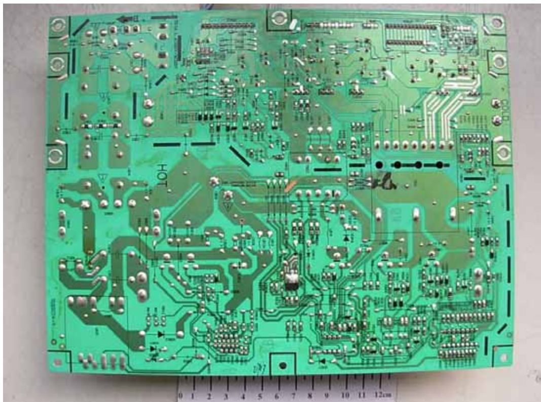
FIGURE 7 LCD TV (M/N: LTDN42W58US) POWER BOARD (SOLDERED SIDE)
