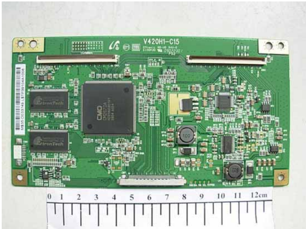
FIGURE 18 LCD TV (M/N: LTDN42W58US) LCD PANEL MAIN BOARD (COMPONENT SIDE)
