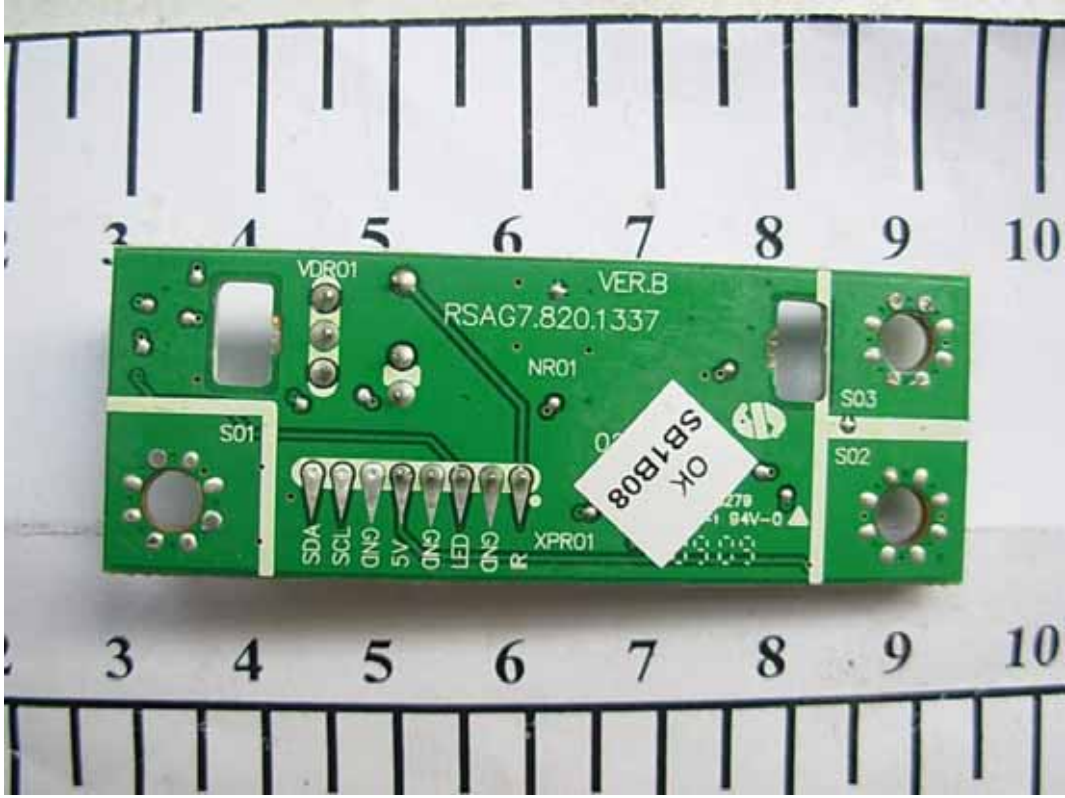
FIGURE 9 LCD TV (M/N: LTDN42W58US) IR BOARD (SOLDERED SIDE)
