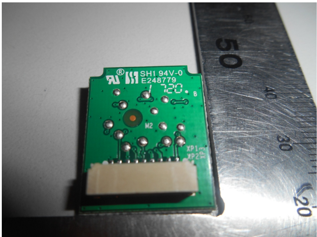
FIGURE 8 LED LCD TV (M/N: LC-32P3000U) IR BOARD (SOLDERED SIDE)
