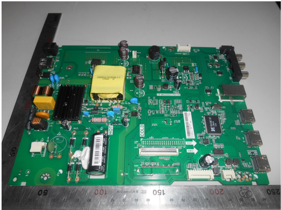
FIGURE 3 LED LCD TV (M/N: LC-32P3000U) MAIN BOARD (COMPONENT SIDE)
