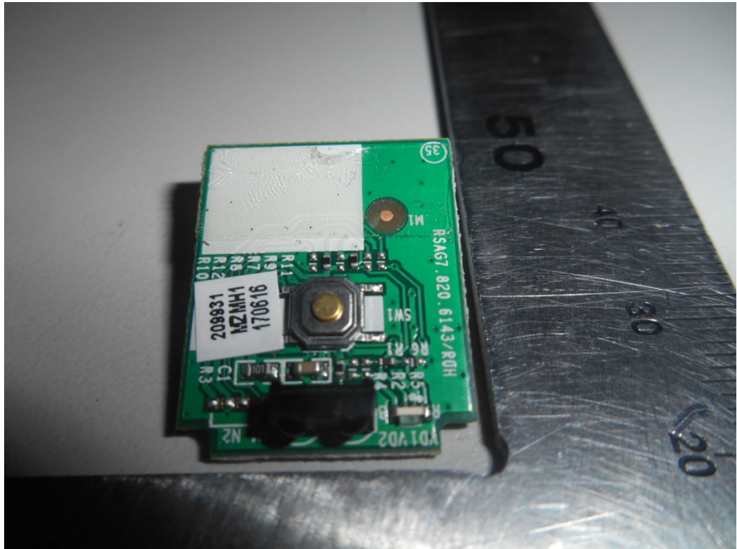
FIGURE 7 LED LCD TV (M/N: LC-32P3000U) IR BOARD (COMPONENT SIDE)
