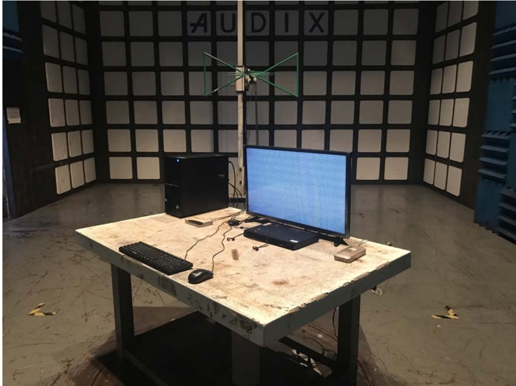
SETUP WITH MAXIMUM DETECTED EMISSION AT HORIZONTAL POLARIZATION (TEST MODE: HDMI3 1920*1080@60Hz & 1kHz PLAYING)
