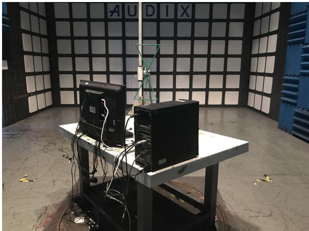
SETUP WITH MAXIMUM DETECTED EMISSION AT VERTICAL POLARIZATION (TEST MODE: HDMI3 1920*1080@60Hz & 1kHz PLAYING)
