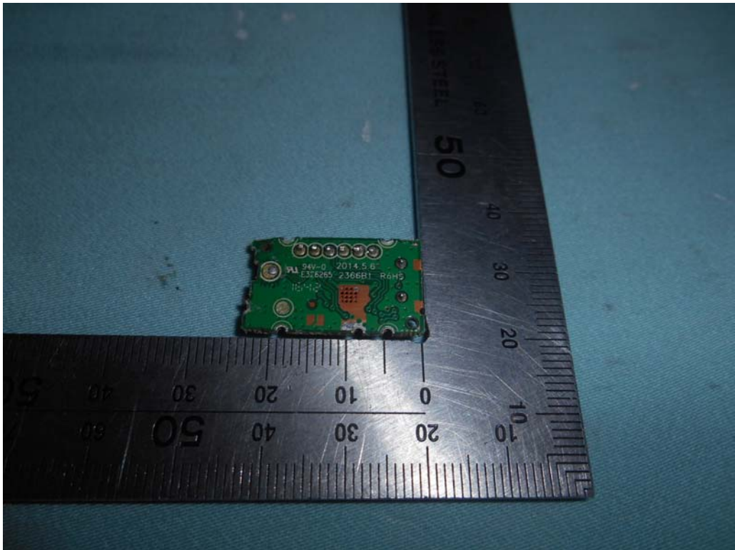
FIGURE 8 LED LCD TV (M/N: 32H4D) TUNER BOARD (SOLDERED SIDE)
