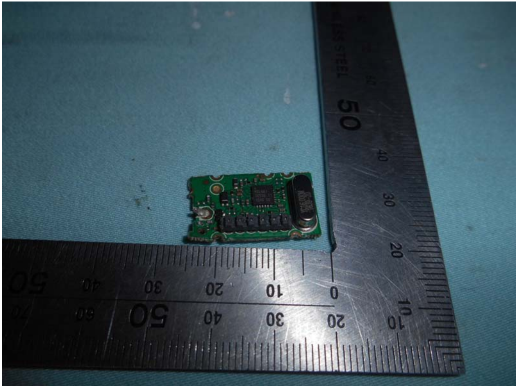
FIGURE 7 LED LCD TV (M/N: 32H4D) TUNER BOARD (COMPONENT SIDE)
