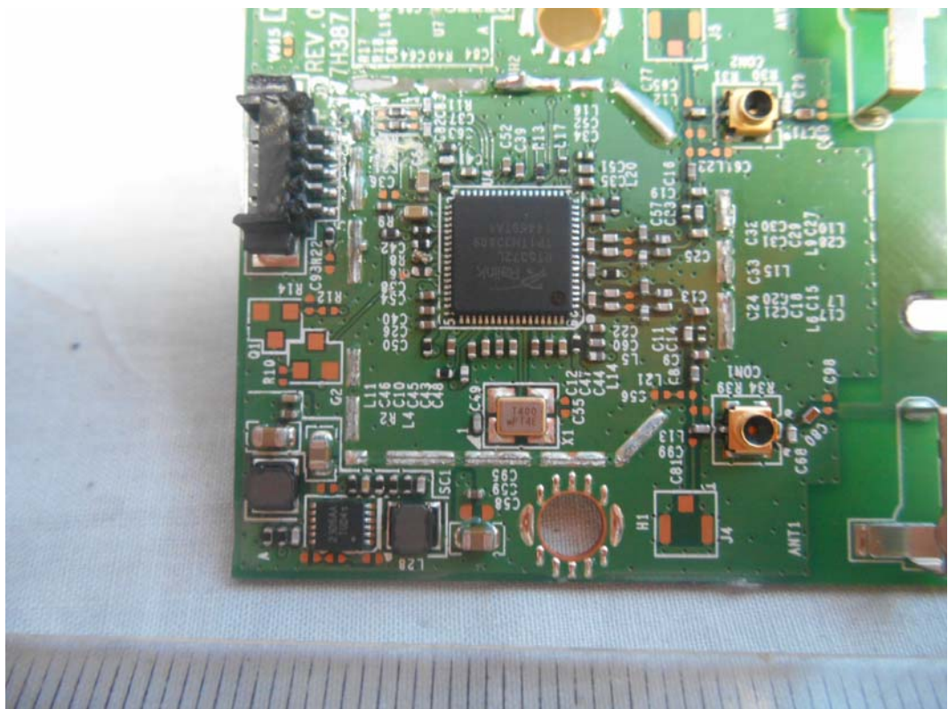
FIGURE 20 LED LCD TV (M/N: LTDN50K2203WUS) CHIP AND CRYSTAL ON RF BOARD
