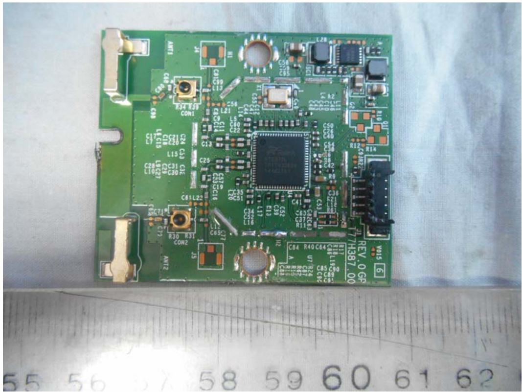
FIGURE 19 LED LCD TV (M/N: LHD32K220WUS) RF BOARD (COMPONENT SIDE)
