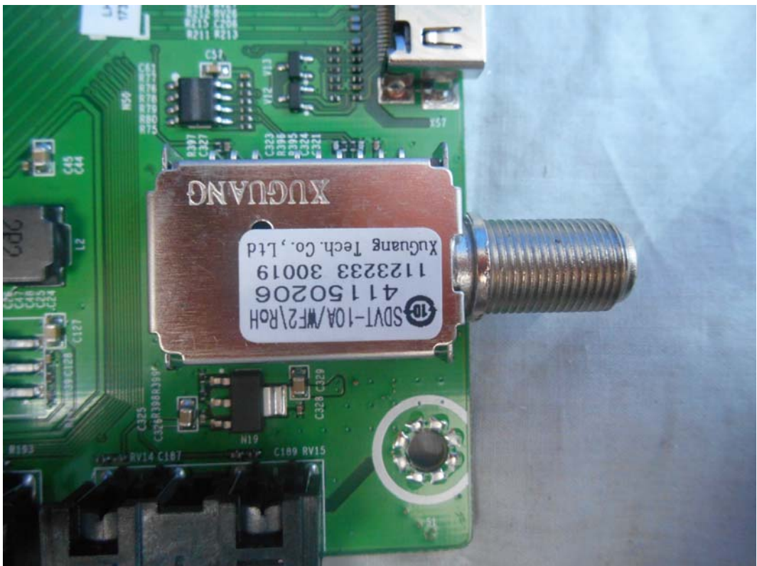
FIGURE 10 LED LCD TV (M/N: LHD32K220WUS) TUNER ON MAIN BOARD
