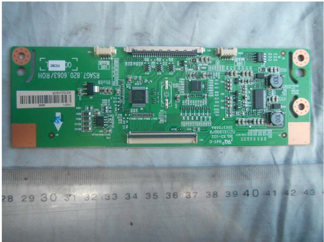
FIGURE 21 LED LCD TV (M/N: LHD32K220WUS) SIGNAL BOARD (COMPONENT SIDE)
