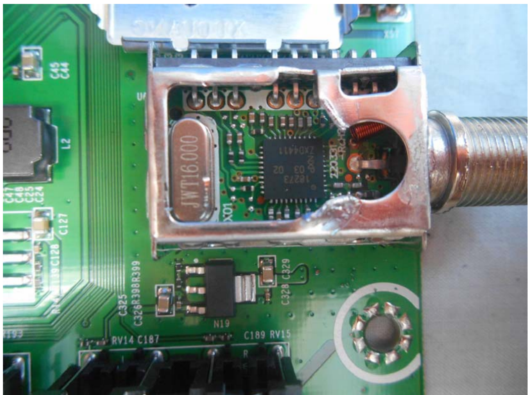
FIGURE 12 LED LCD TV (M/N: LHD32K220WUS) CHIP & CRYSTAL ON TUNER BOARD
