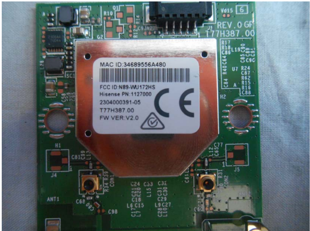
FIGURE 17 LED LCD TV (M/N: LHD32K220WUS) LABEL ON RF BOARD
