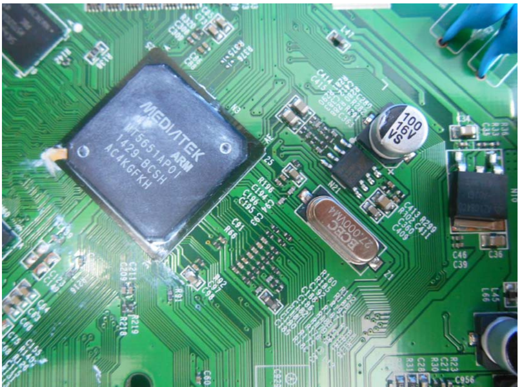
FIGURE 8 LED LCD TV (M/N: LHD32K220WUS) CHIP #2 & CRYSTAL ON MAIN BOARD
