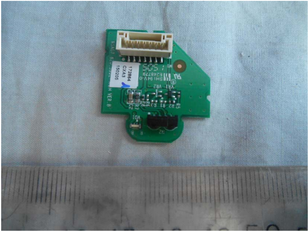
FIGURE 28 LED LCD TV (M/N: LHD32K220WUS) IR BOARD (COMPONENT SIDE)
