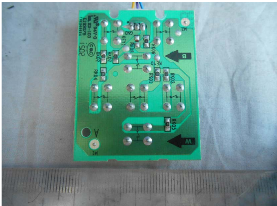
FIGURE 14 LED LCD TV (M/N: LHD32K220WUS) KEY BOARD (SOLDERED SIDE)
