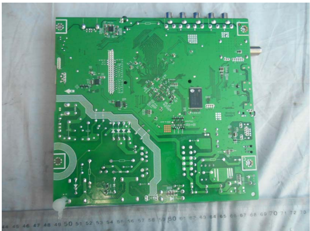
FIGURE 6 LED LCD TV (M/N: LHD32K220WUS) MAIN BOARD (SOLDERED SIDE)
