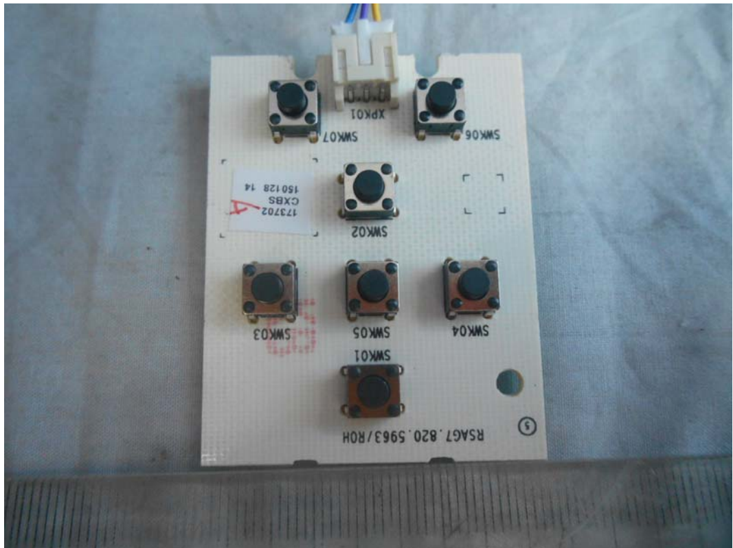
FIGURE 13 LED LCD TV (M/N: LHD32K220WUS) KEY BOARD (COMPONENT SIDE)
