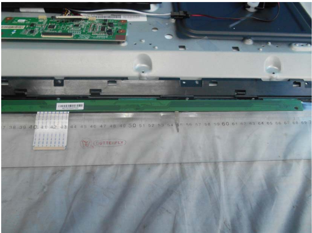
FIGURE 27 LED LCD TV (M/N: LHD32K220WUS) CONTROL BOARD #2 (SOLDERED SIDE)
