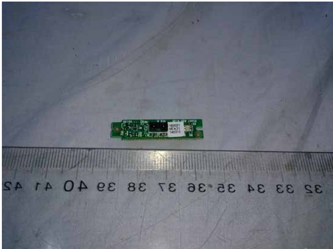
FIGURE 11 LED LCD TV (M/N: 32K20D) IR BOARD (COMPONENT SIDE)
