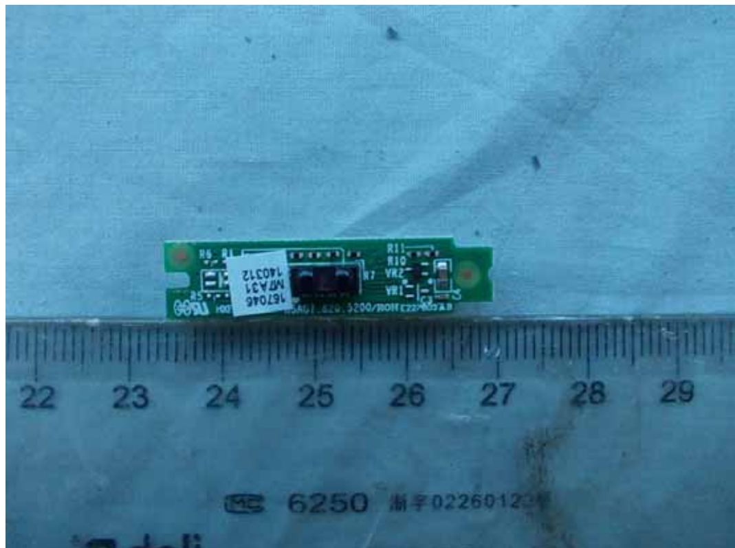
FIGURE 14 LED LCD TV (M/N: 32K366MH) IR BOARD (COMPONENT SIDE)
