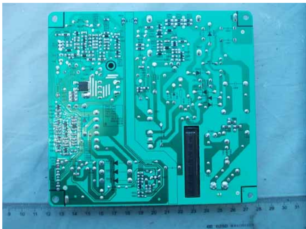
FIGURE 4 LED LCD TV (M/N: 32K366MH) POWER BOARD (SOLDERED SIDE)
