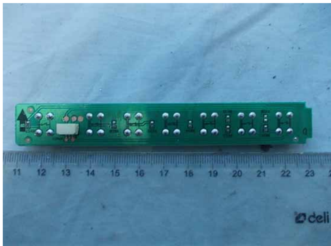
FIGURE 13 LED LCD TV (M/N: 32K366MH) KEY BOARD (SOLDERED SIDE)
