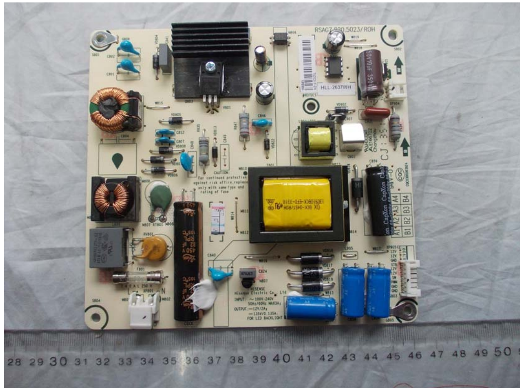
FIGURE 3 LED LCD TV (M/N: 32K366HS) POWER BOARD (COMPONENT SIDE)
