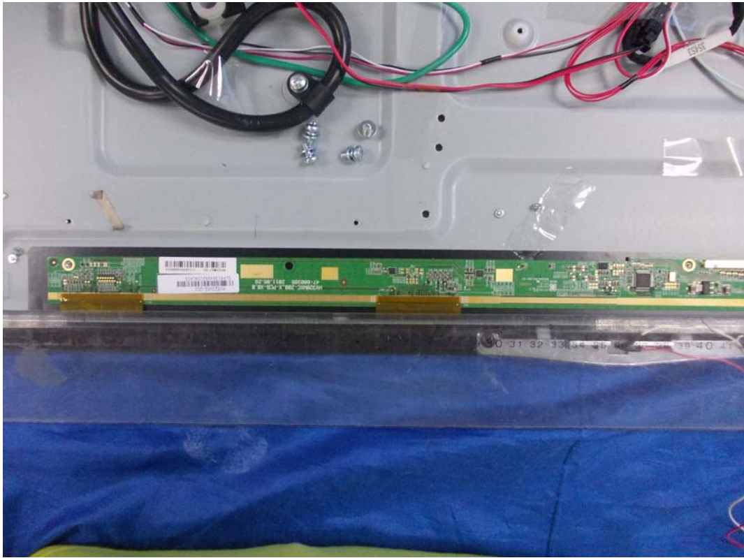
FIGURE 13 LED LCD TV (M/N: 32K366HS) LCD PANEL CONTROL BOARD (COMPONENT SIDE #1)
