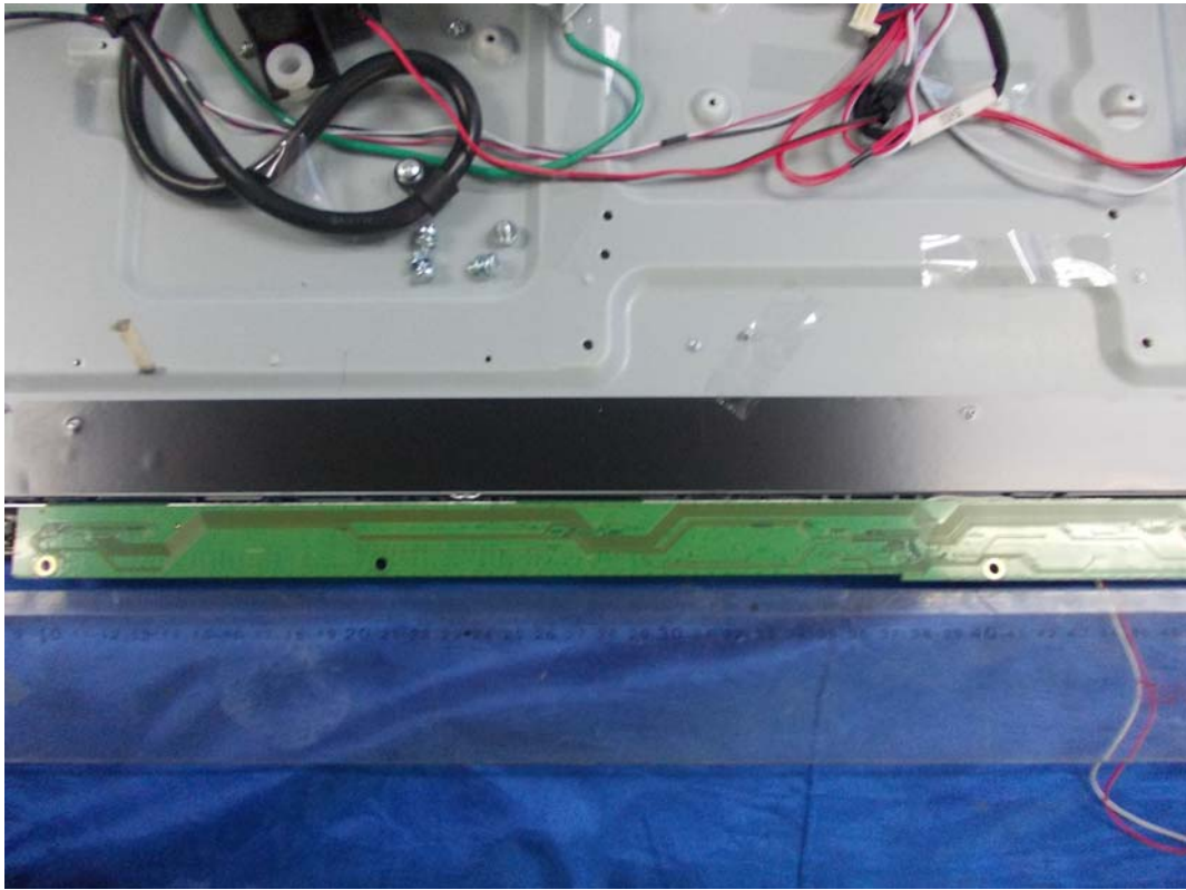
FIGURE 15 LED LCD TV (M/N: 32K366HS) LCD PANEL CONTROL BOARD (SOLDERED SIDE #1)
