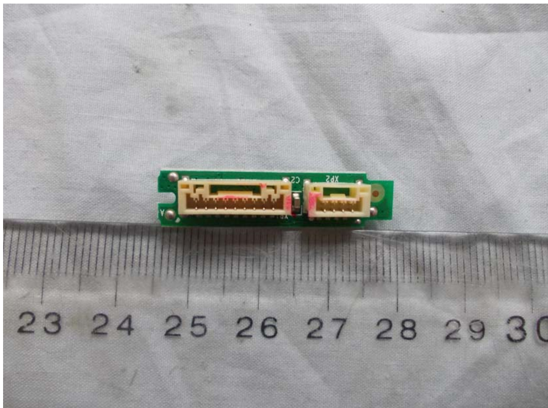
FIGURE 12 LED LCD TV (M/N: 32K366HS) IR BOARD (SOLDERED SIDE)
