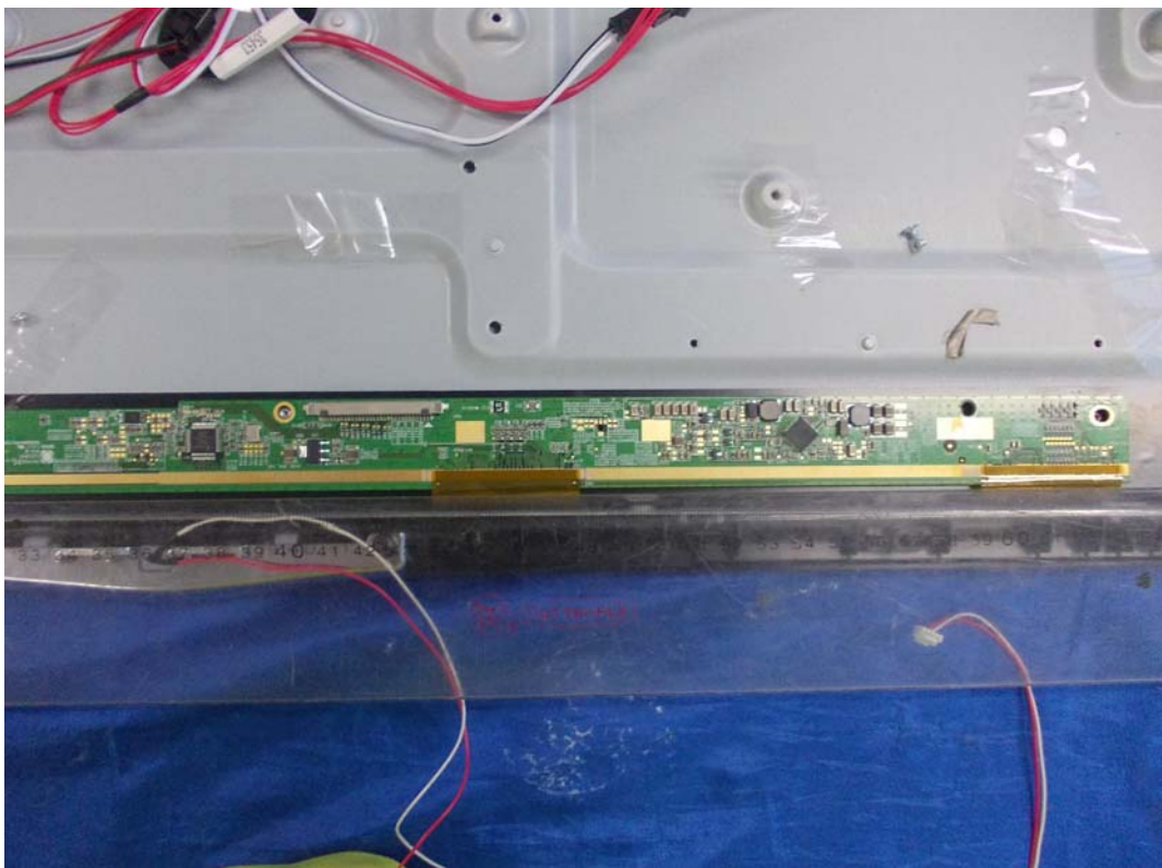
FIGURE 14 LED LCD TV (M/N: 32K366HS) LCD PANEL CONTROL BOARD (COMPONENT SIDE #2)
