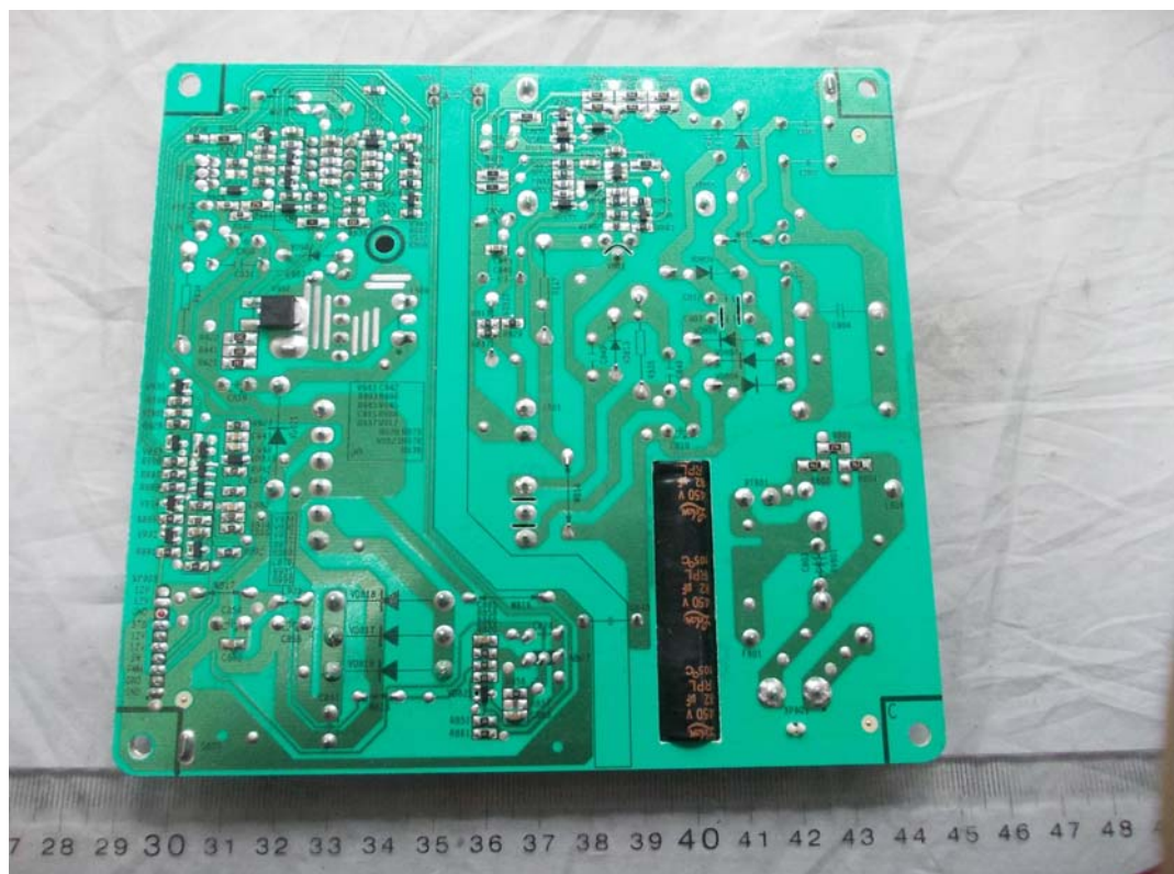
FIGURE 4 LED LCD TV (M/N: 32K366HS) POWER BOARD (SOLDERED SIDE)
