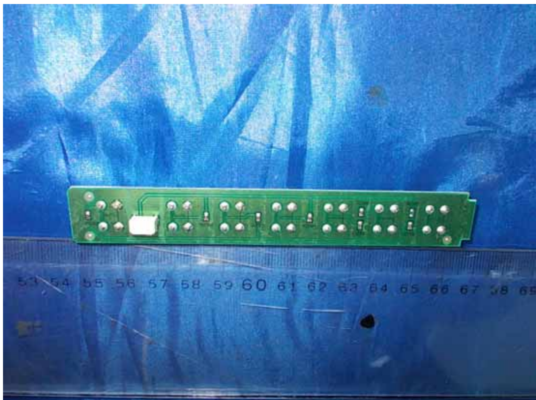
FIGURE 11 LED LCD TV (M/N: 32K366W) KEY BOARD (SOLDERED SIDE)
