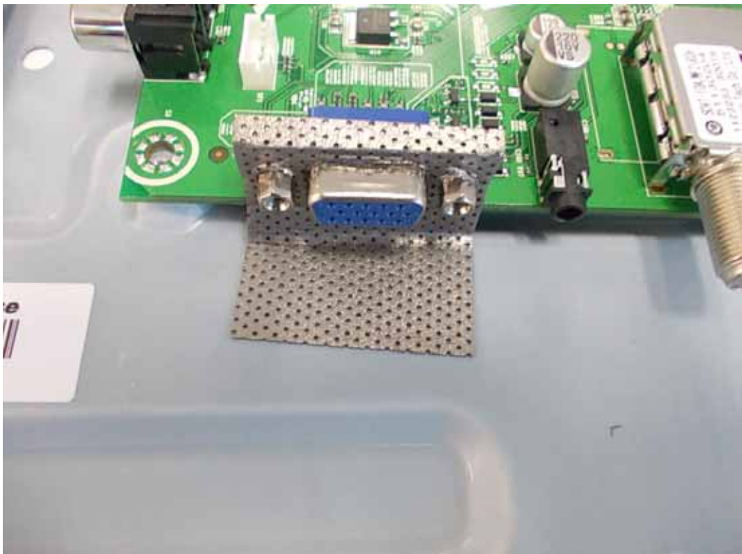
FIGURE 15 LED LCD TV (M/N: 32K366W) DEBUG #2
