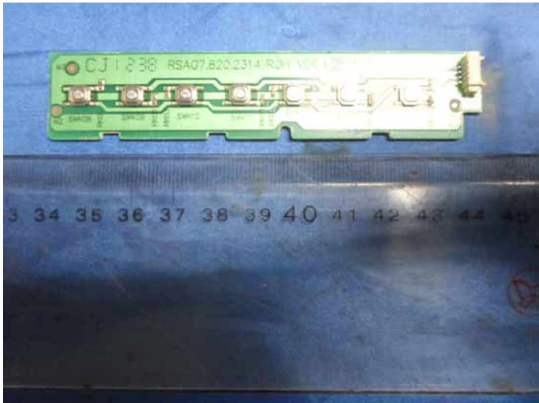
FIGURE 9 LED LCD TV (M/N: LHD32K310HUS) KEY BOARD (COMPONENT SIDE)
