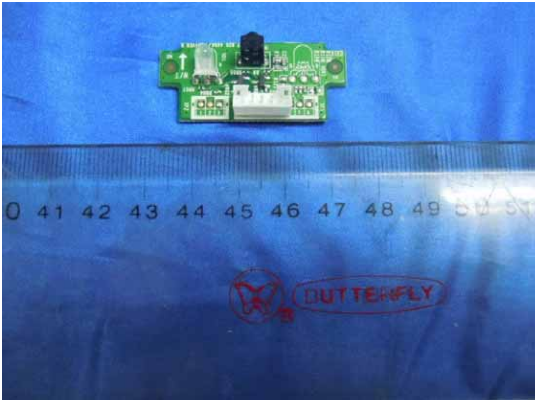
FIGURE 14 LED TV (M/N: LHD32K21MH) IR BOARD (COMPONENT SIDE)
