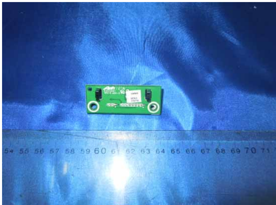
FIGURE 12 LCD TV (M/N: LHD32V77US) IR BOARD (SOLDERED SIDE)
