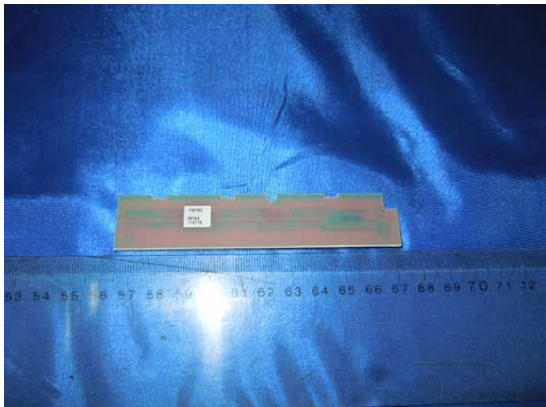
FIGURE 10 LCD TV (M/N: LHD32V77US) KEY BOARD (SOLDERED SIDE)
