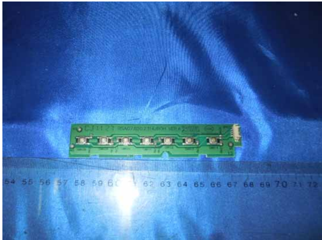
FIGURE 9 LCD TV (M/N: LHD32V77US) KEY BOARD (COMPONENT SIDE)
