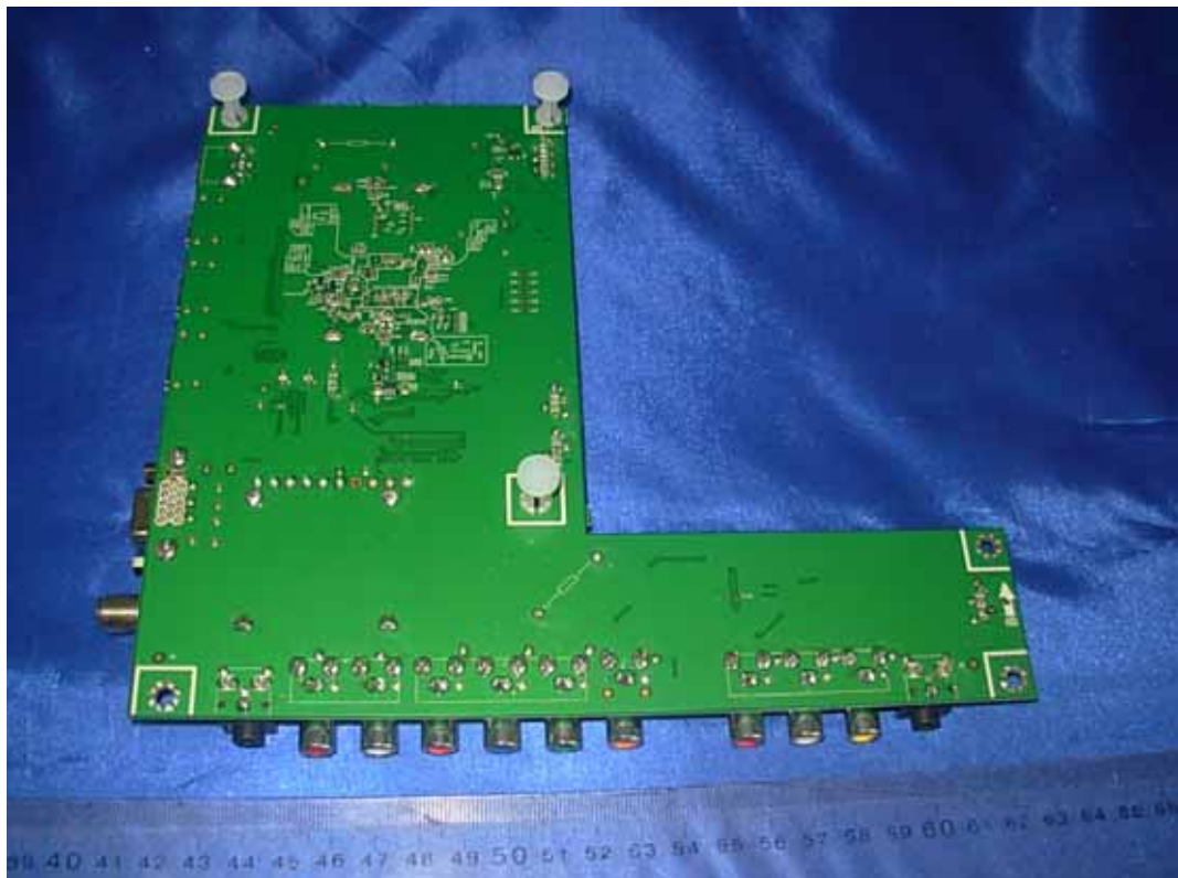
FIGURE 6 LCD TV (M/N: LHD32K20US) MAIN BOARD (SOLDERED SIDE)
