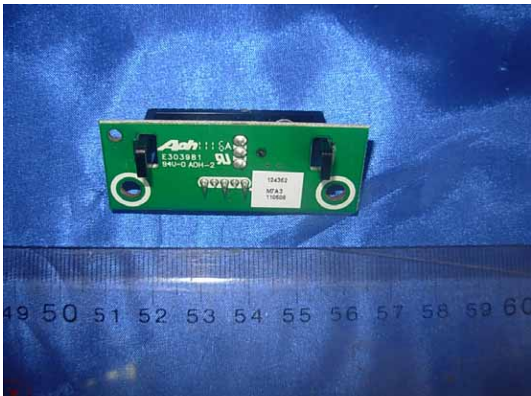
FIGURE 11 LCD TV (M/N: LHD32V77MH) IR BOARD (SOLDERED SIDE)
