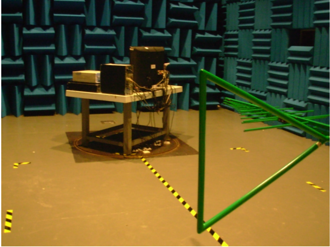
SETUP WITH MAXIMUM DETECTED EMISSION AT HORIZONTAL POLARIZATION (HDMI 640*480@60Hz)
