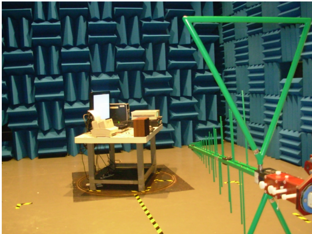
SETUP WITH MAXIMUM DETECTED EMISSION AT VERTICAL POLARIZATION (HDMI 640*480@60Hz)
